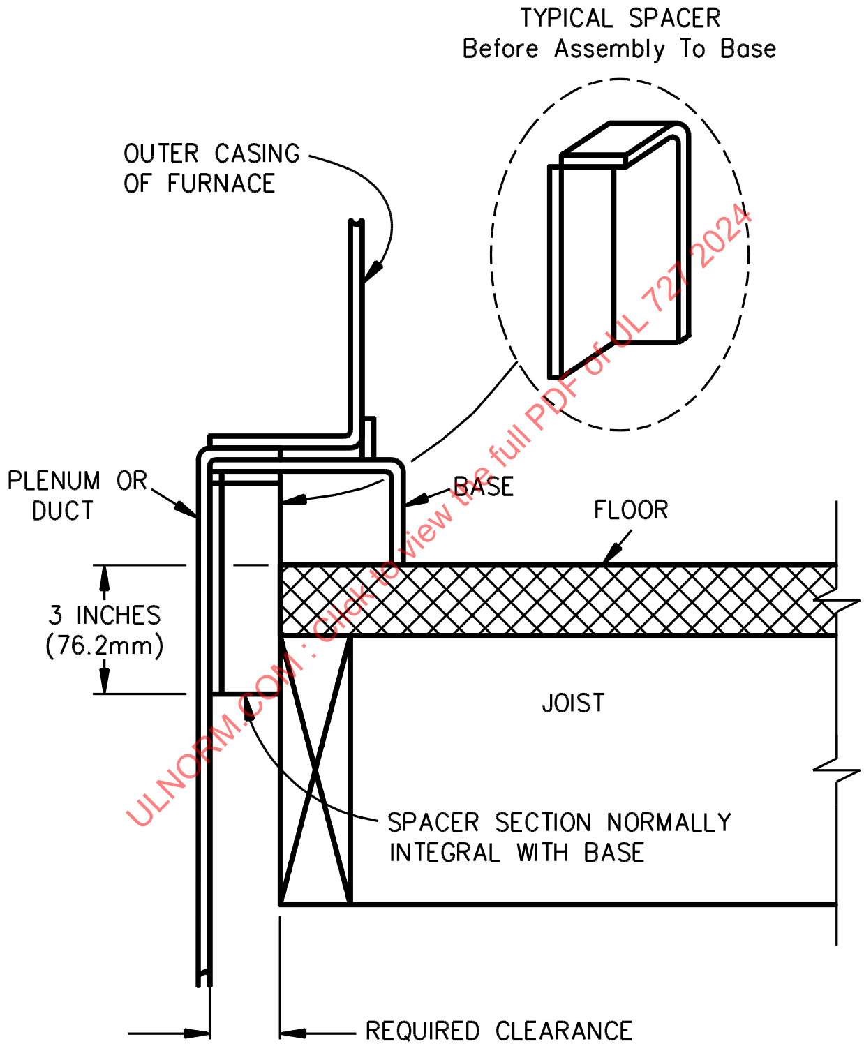
Figure 8.1 Acceptable base construction for downflow furnace
