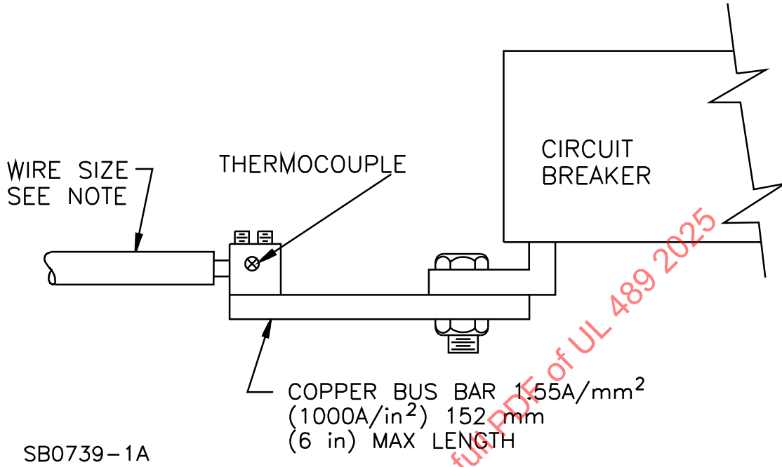
Figure 26.2 Connection for Bolt-On Circuit Breaker Rated Less Than 1600 A
