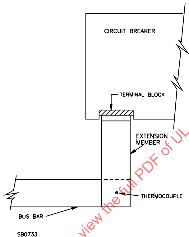
Figure 26.4 Connection for Circuit Breaker with Extension Member
