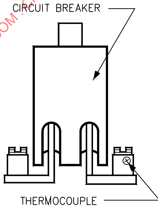
Figure 26.3 Connection for Plug-In Circuit Breakers
