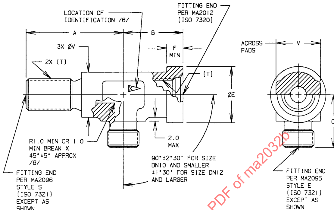
FIGURE 1 TEE, FLARELESS
