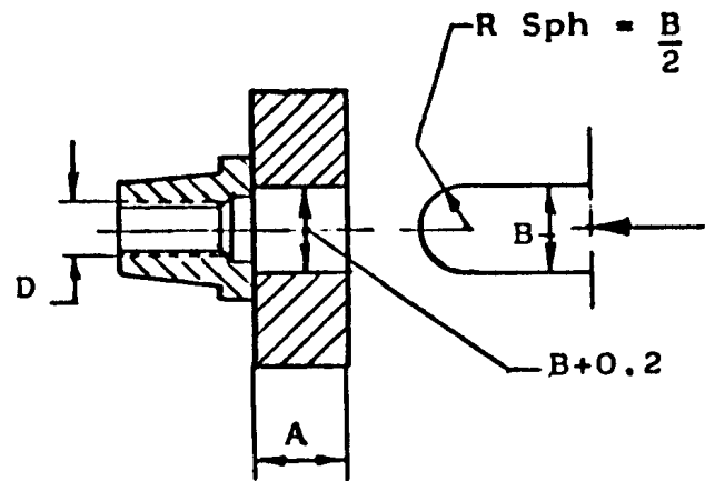
FIGURE C2 - PUSH-OUT TEST APPARATUS
