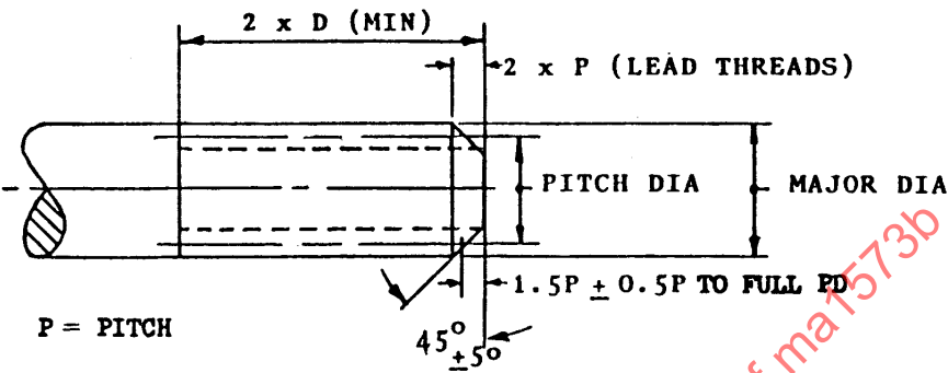
FIGURE E2 - MINIMUM MANDREL
