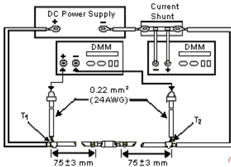
FIGURE 2 - CURRENT RESISTANCE TEST SET-UP
