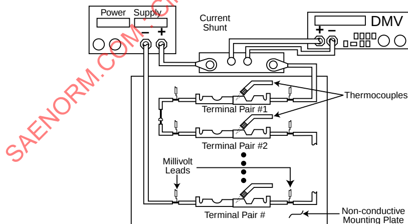
FIGURE 3 - SET-UP FOR MAXIMUM TEST CURRENT
