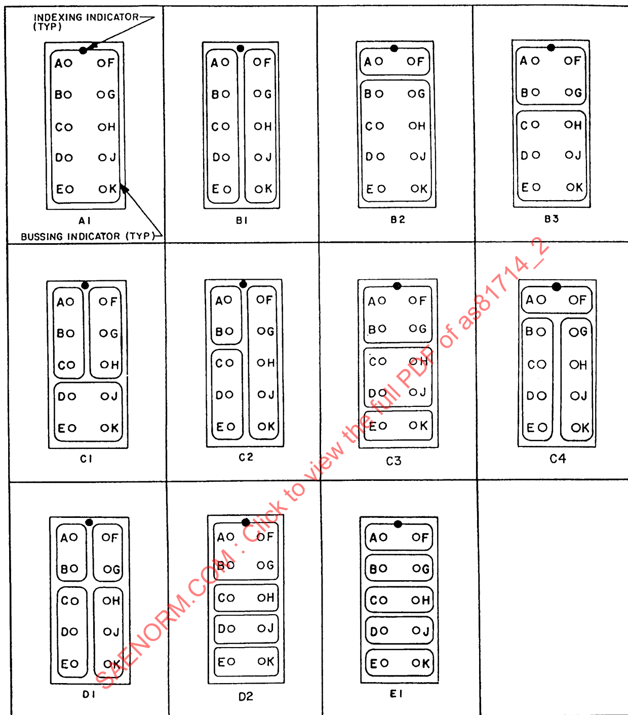
FIGURE 1. BUSSING ARRANGEMENTS.
