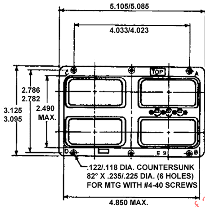
FIGURE 2 – CONNECTOR CONFIGURATIONS AND DIMENSIONS
