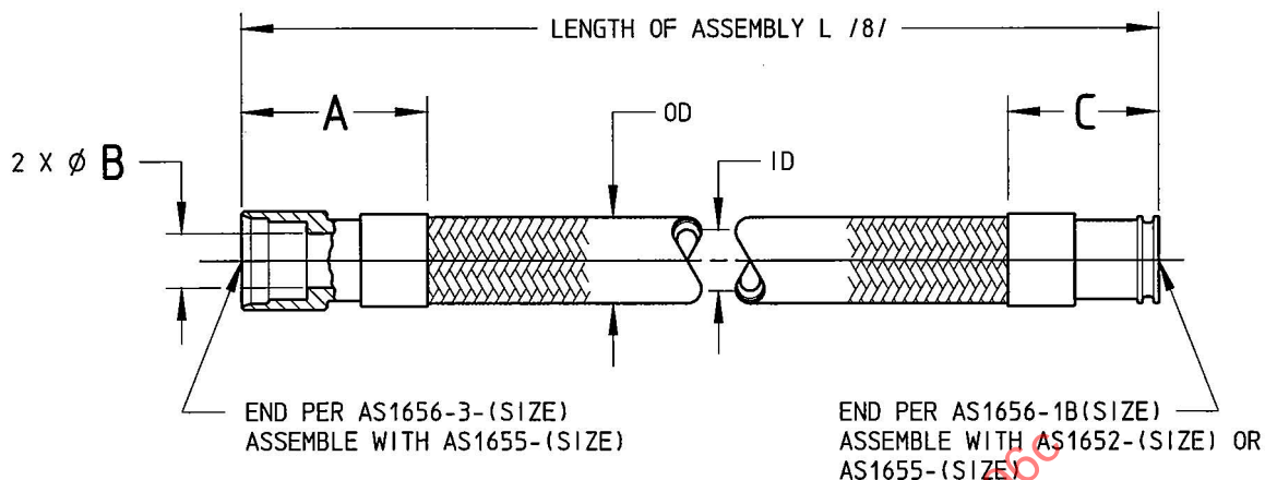
FIGURE 1 - HOSE ASSEMBLY
