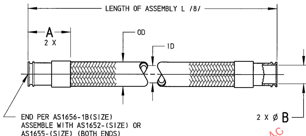
FIGURE 1 - HOSE ASSEMBLY
