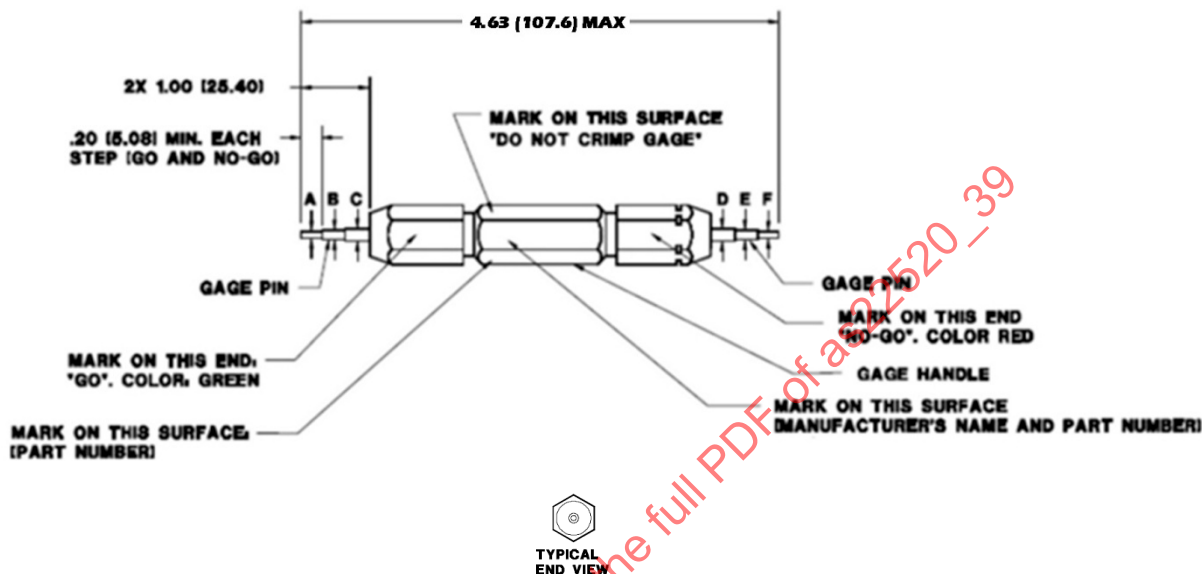
FIGURE 1 – AS22520/39-01 GAGE FOR AS22520/37-01 AND AS22520/44-01 CRIMPING TOOLS
