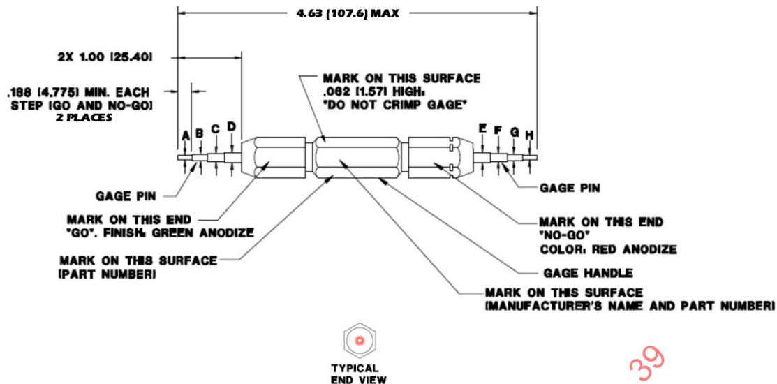
FIGURE 2 – AS22520/39-02 GAGE FOR AS22520/38-01 CRIMPING TOOL
