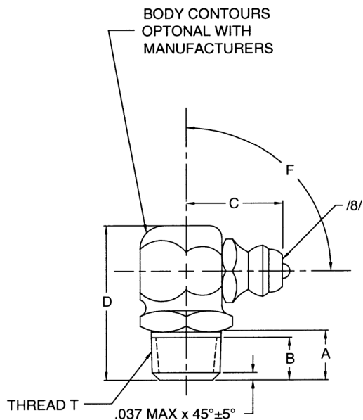
FIGURE 3 - FITTING, ELBOW 90°
