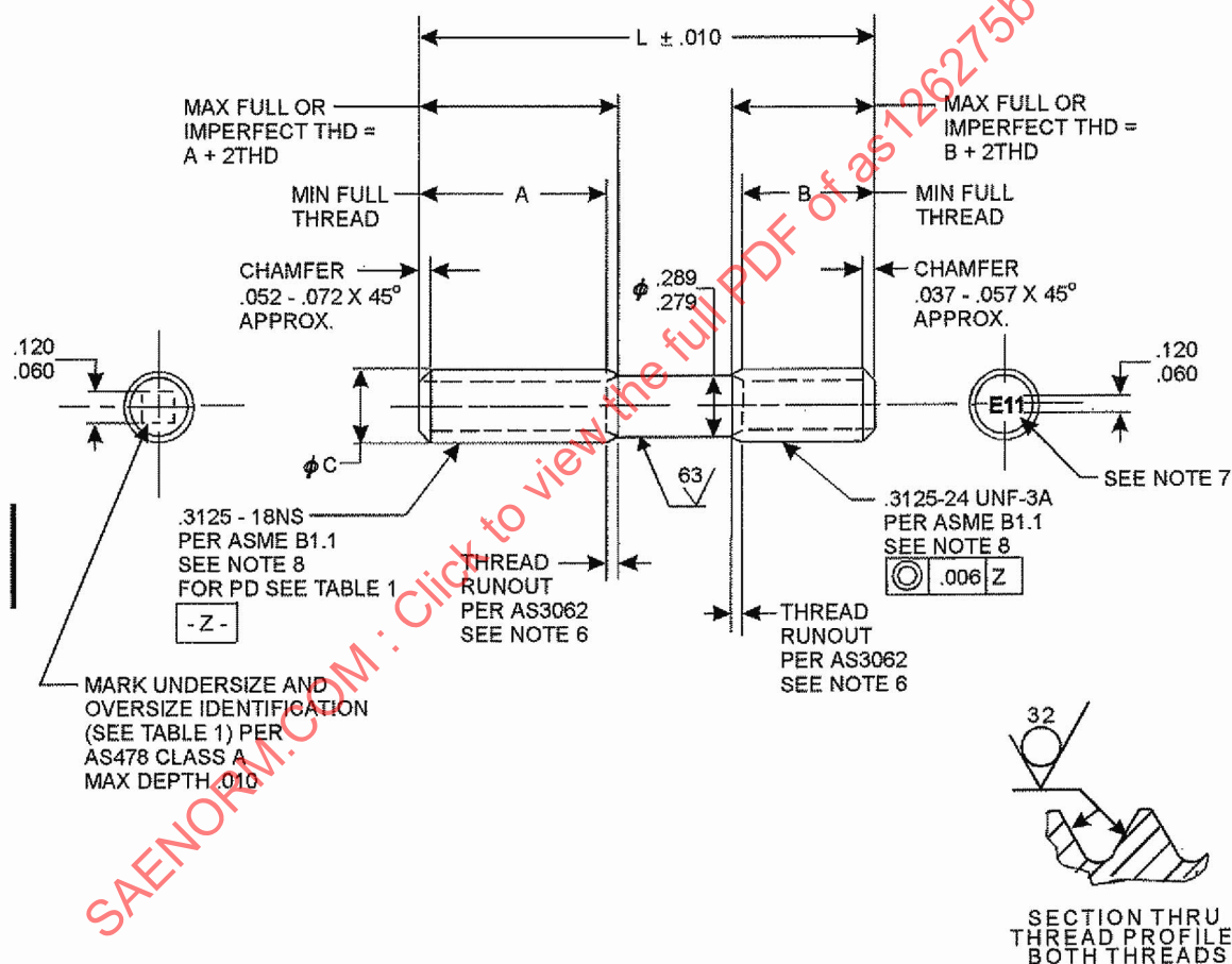
FIGURE 1 - STUD
