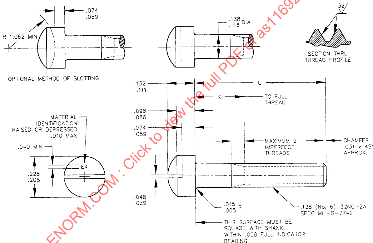
FIGURE 1 – SCREW
