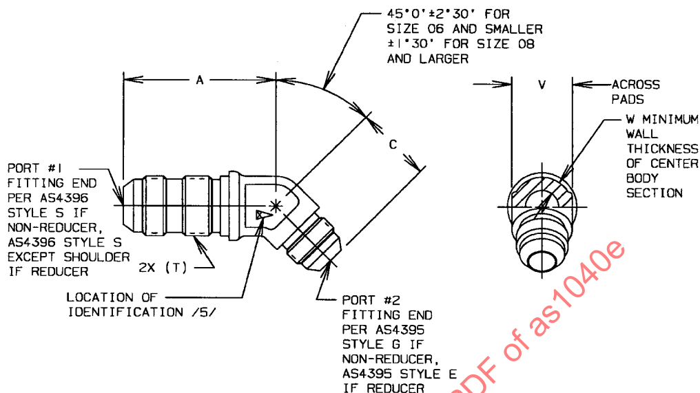
FIGURE 1 - FITTING, ELBOW, 45°, BULKHEAD END FOR OPTIONAL USE IN PORT PORT #2 SHOWN AS REDUCER
