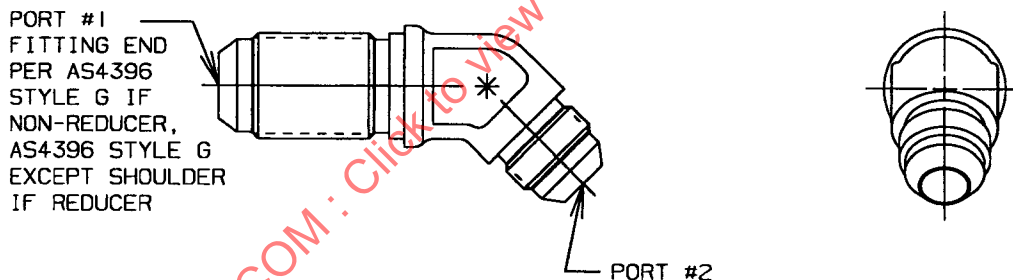
FIGURE 2 - FITTING, ELBOW, 45°, BULKHEAD END NOT FOR USE IN PORT PORT #2 SHOWN AS REDUCER SAME AS FIGURE 1 EXCEPT AS SHOWN /20/
