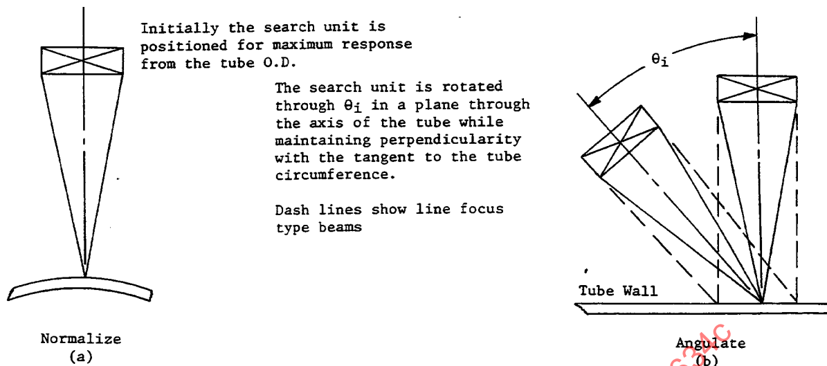
Figure 5 - Axial angulation
