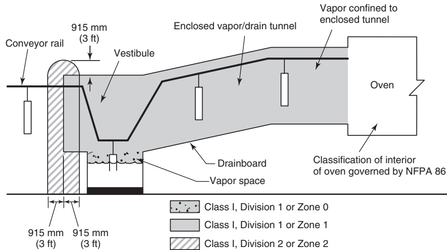
Figure 516.3(D)(7) Electrical Area Classification Around an Enclosed Dipping or Coating Process. [34:Figure 6.5]
