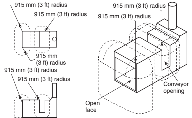
Figure 516.3(D)(2) Class I, Division 2; Class I, Zone 2; Class II, Division 2; or Zone 22 Locations Adjacent to a Closed Top, Open Face, or Open Front Spray Booth or Room.
