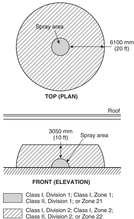
Figure 516.3(D)(1) Electrical Area Classification for Unenclosed Spray Areas. [33:Figure 6.5.1]
