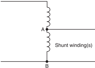
Figure 450.4(A) Autotransformer.
