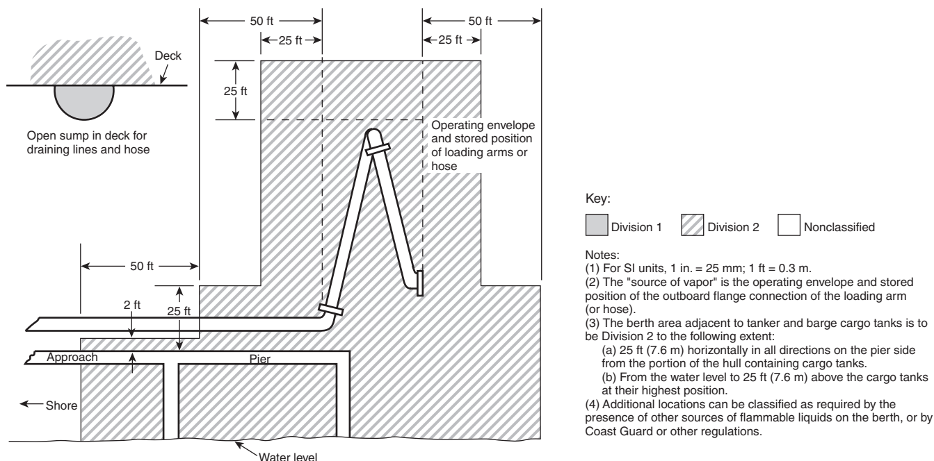
Figure 515.3 Marine Terminal Handling Flammable Liquids. [30:Figure 29.3.22]
