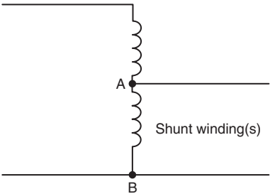
Figure 450.4 Autotransformer.
