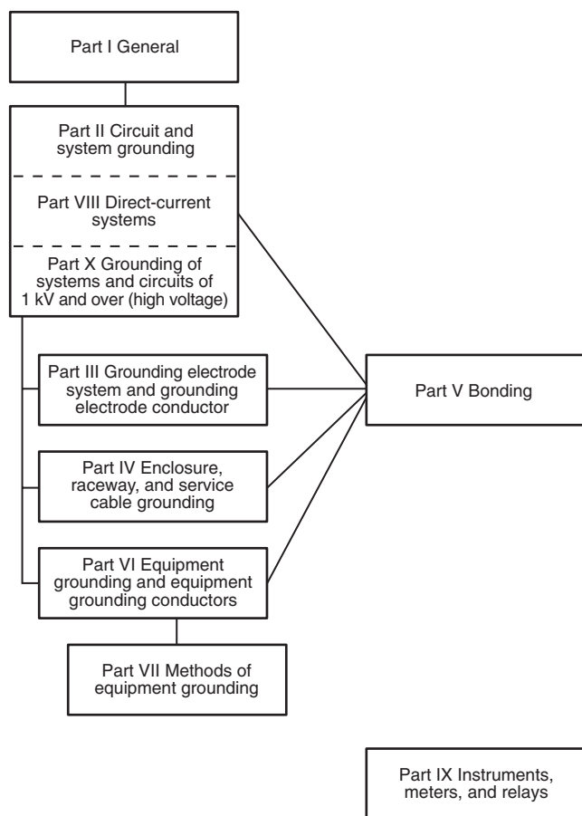
Figure 250.4 Grounding.
