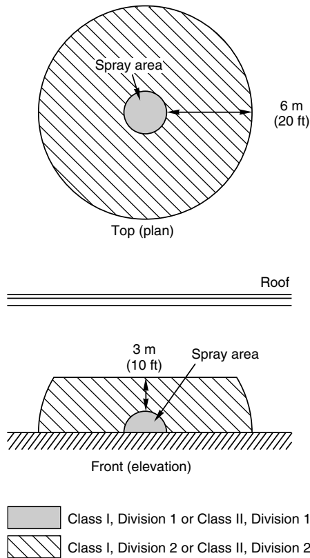
Figure 516.3(B)(1) Electrical area classification for open spray areas. [NFPA 33, Figure 4.3.1]
