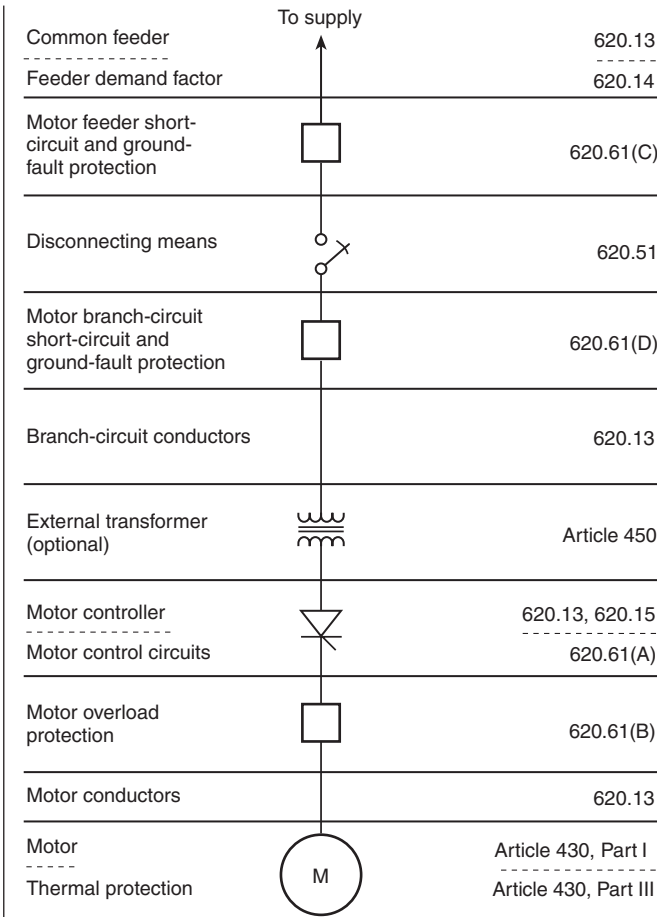
Figure 620.13 Single-line diagram.
