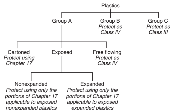
FIGURE 17.1.2.1 Decision Tree.
