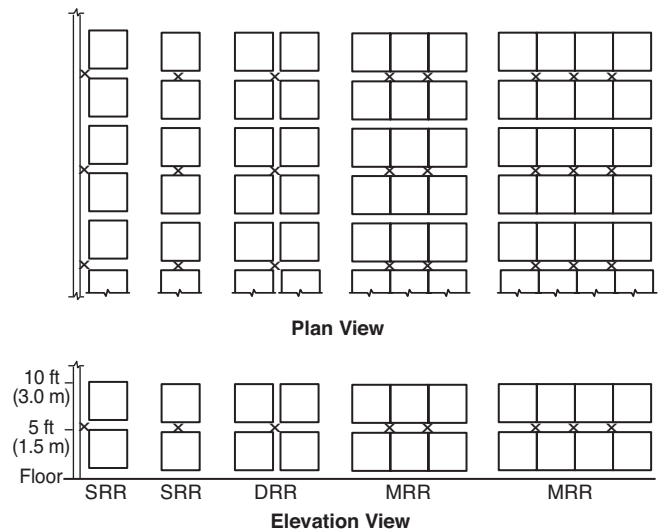
FIGURE 17.2.1.2.1(f) Storage 25 ft (7.6 m) in Height with 5 ft to 10 ft (1.5 m to 3.0 m) Clearance to Ceiling. (See Note 2.)
