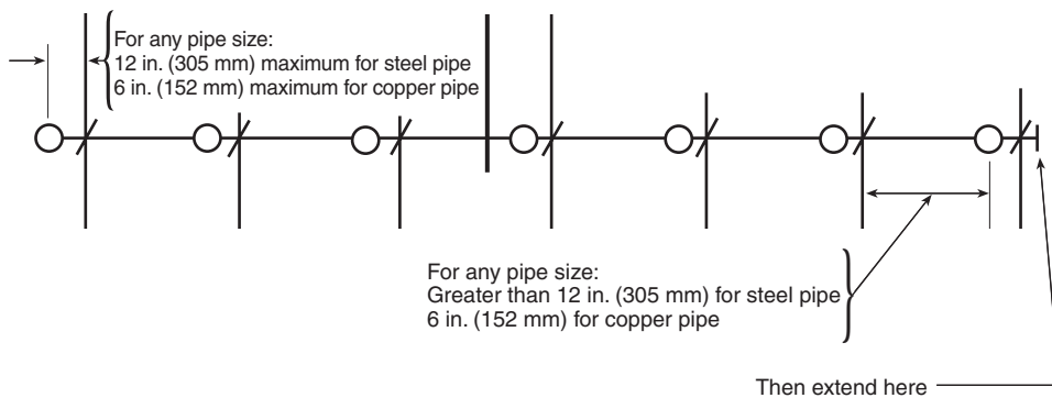
FIGURE A.9.2.3.4(a) Distance from Sprinkler to Hanger Where Maximum Pressure Exceeds 100 psi (6.9 bar) and Branch Line Above Ceiling Supplies Pendent Sprinklers Below Ceiling.
