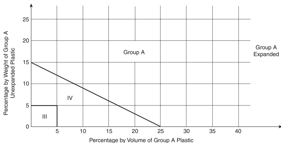
FIGURE 5.6.3.3(a) Commodities Containing a Mixture of Expanded and Unexpanded Group A Plastics.
