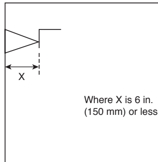
FIGURE A.8.7.4.1.2.1 Sidewall Sprinkler Deflector Measurement From Walls.
