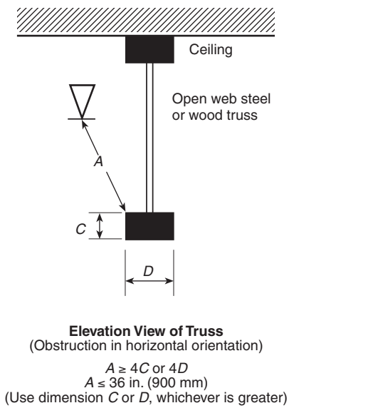
FIGURE 8.8.5.2.1.3(b) Minimum Distance from an Obstruction in the Horizontal Orientation (Extended Coverage Upright and Pendent Spray Sprinkler).
