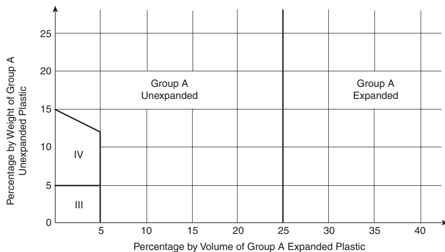
FIGURE 5.6.3.3(b) Exposed Commodities Containing a Mixture of Expanded and Unexpanded Group A Plastics.
