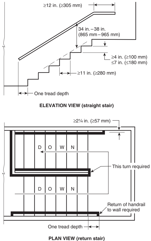
FIGURE A.7.2.2.4.4 Handrail Details.
