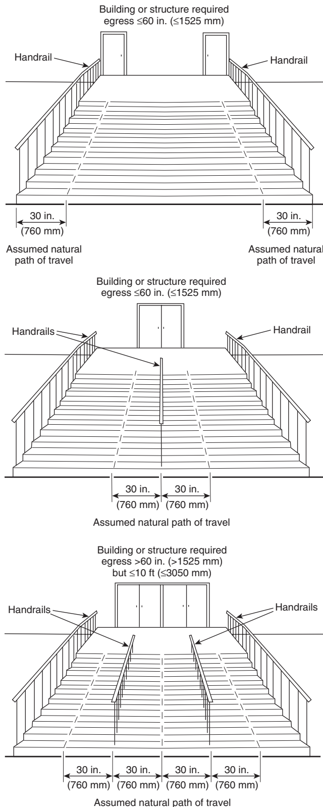
FIGURE A.7.2.2.4.4 Handrail Details.
