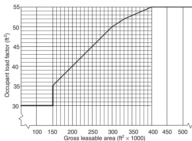
FIGURE 7.3.1.2(b) Mall Building Occupant Load Factors.
