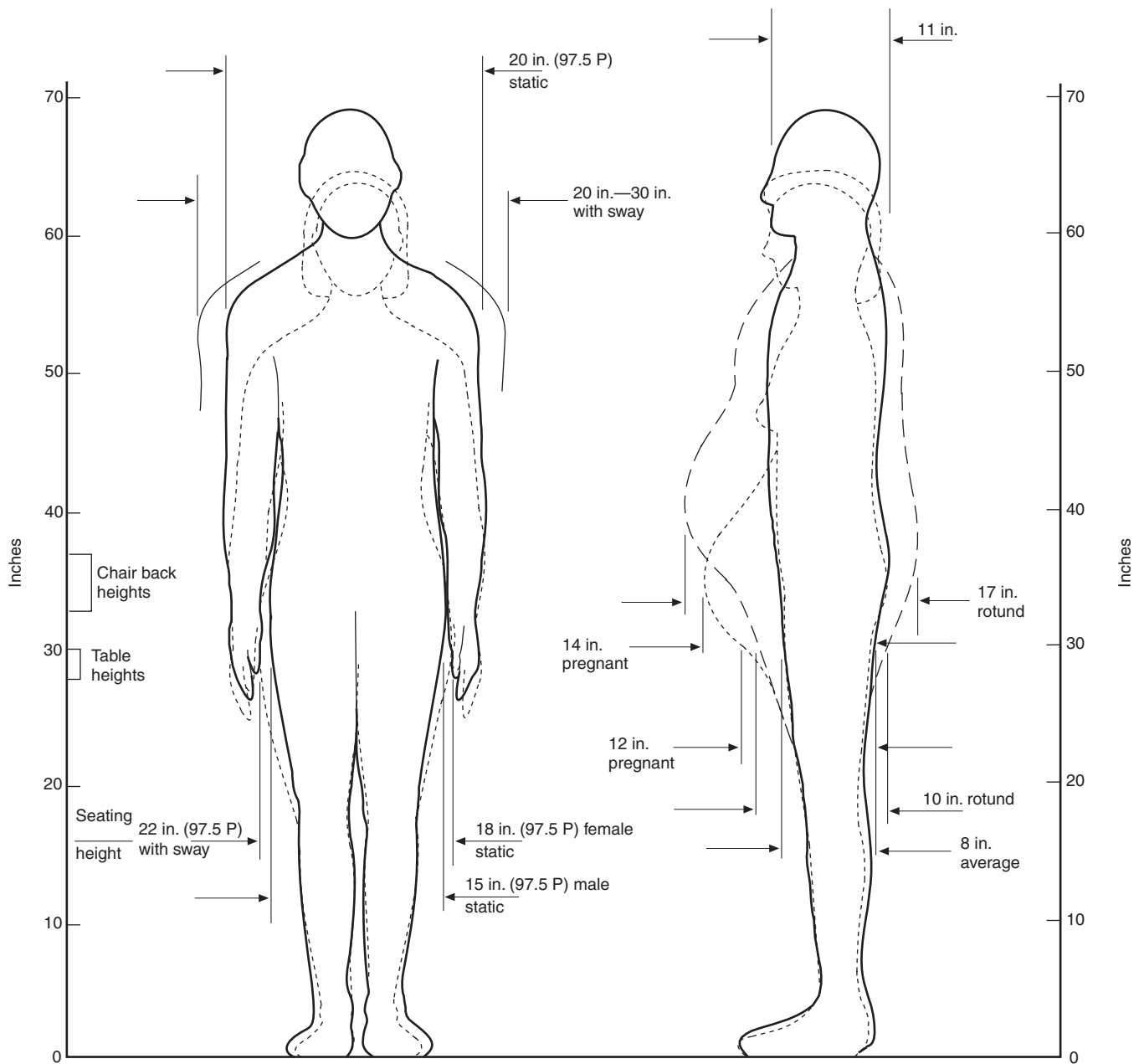
FIGURE A.7.3.4.1.1(b) Anthropometric Data (in in.) for Adults; Male and Female Figures of Average, 50th Percentile, Size, Some Dimensions Apply to Very Large, 97.5 Percentile (97.5 P), Adults.
