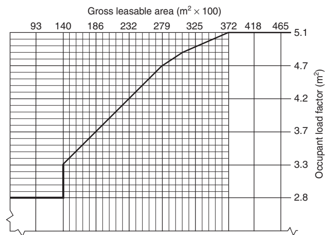
FIGURE 7.3.1.2(a) Mall Building Occupant Load Factors.
