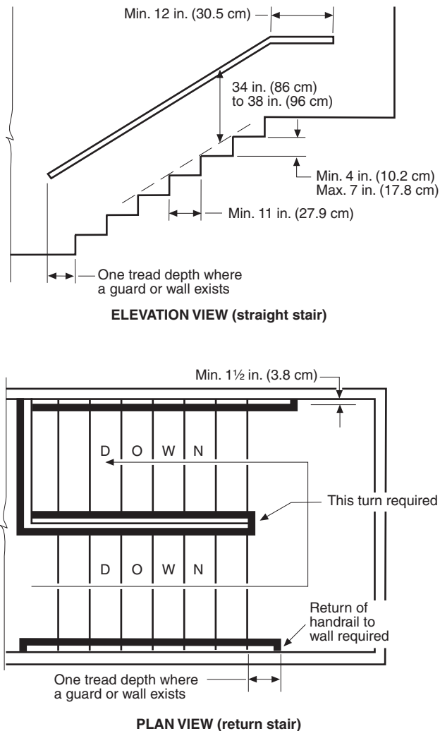
FIGURE A.7.2.2.4.5 Handrail details.
