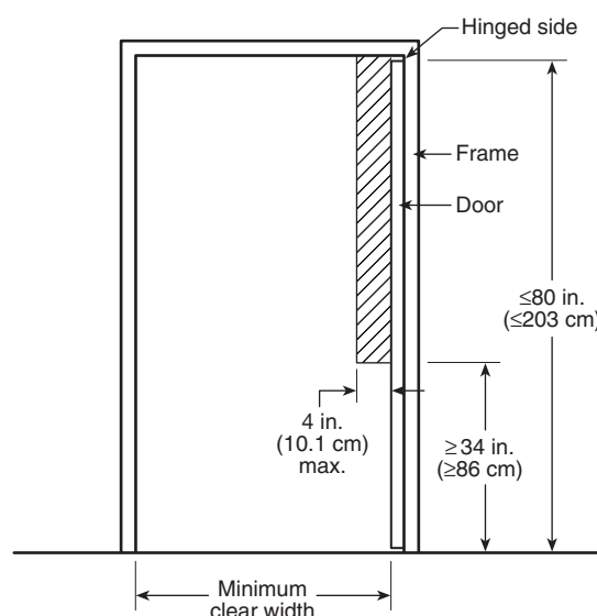
FIGURE A.7.2.1.2.2(b) Minimum clear width with permitted obstructions.
