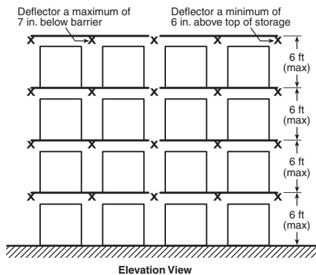
FIGURE 66.16.2.1(a) Single-Row Rack Sprinkler Layout for Design Scheme “B” — Sprinklers in Center of Rack. [30: Figure 16.6.2.1(a)]
