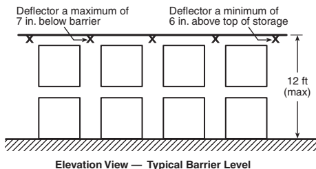
FIGURE 66.16.6.1.1(c) Multiple-Row Rack Sprinkler Layout for Design Scheme “A.” [30: Figure 16.6.1.1(c)]
