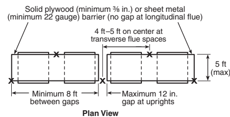
FIGURE 66.16.2.1(a) Single-Row Rack Sprinkler Layout for Design Scheme “B” — Sprinklers in Center of Rack. [30: Figure 16.6.2.1(a)]
