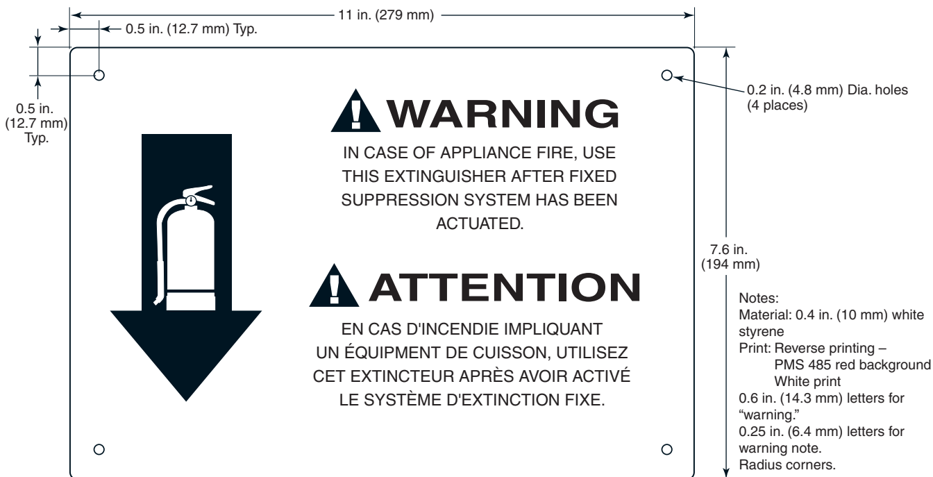
FIGURE A.13.6.2.5.3(b) Typical Class K Placard in English and French. [10:Figure A.5.5.5.3(b)]
