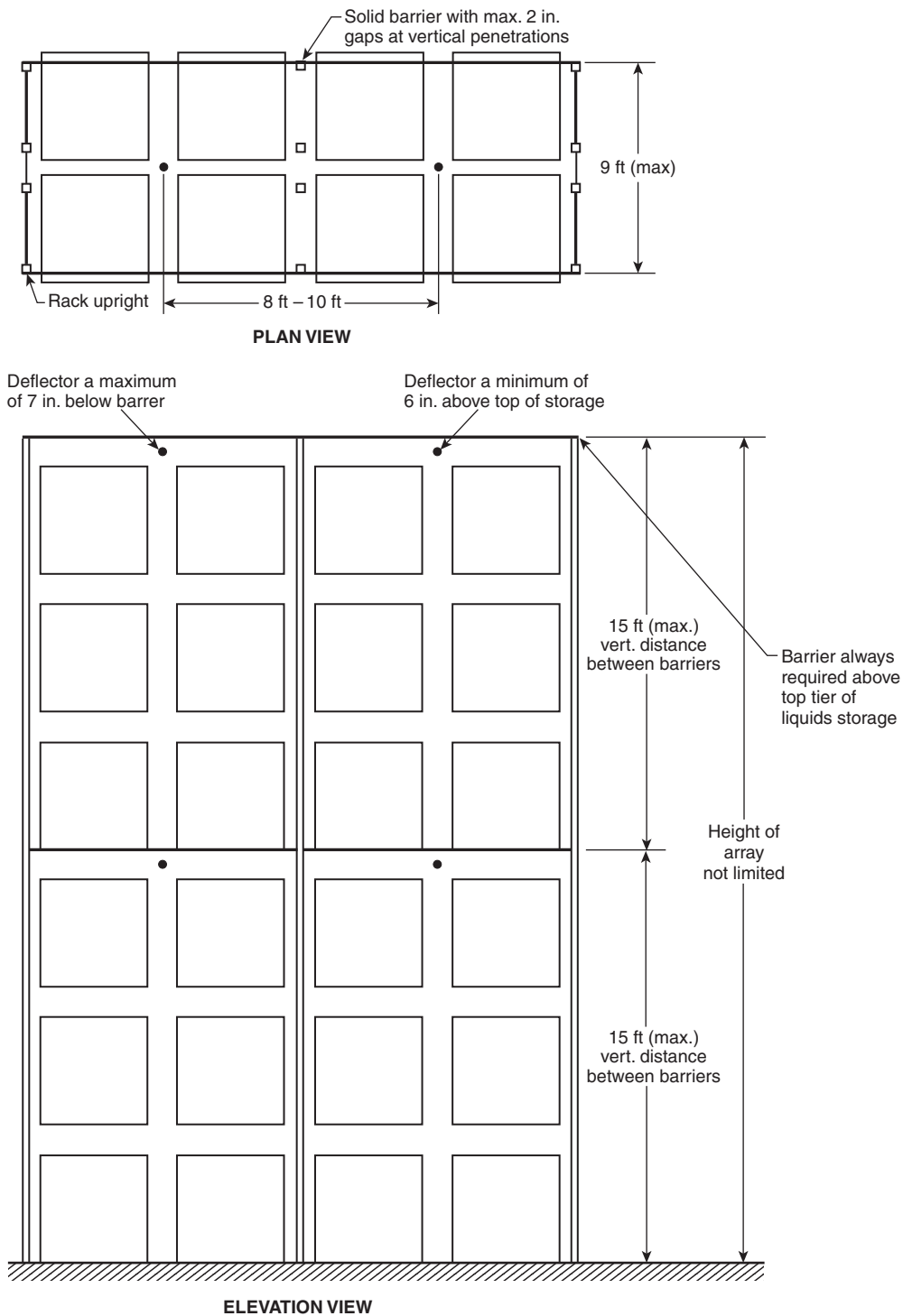
FIGURE 66.16.4.1(b) Double-Row Rack Sprinkler Layout for Design Scheme “E.” [30:16.6.4.1(b)]
