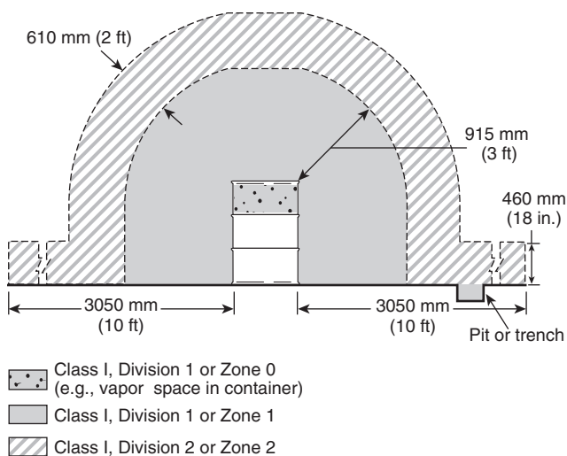
FIGURE 43.1.4.4.5.2 Electrical Area Classification for Class I Liquid Operations Around Open Containers, Supply Containers, Waste Containers, Spray Gun Cleaners, and Solvent Distillation Units. [33:Figure 6.5.5.2]
