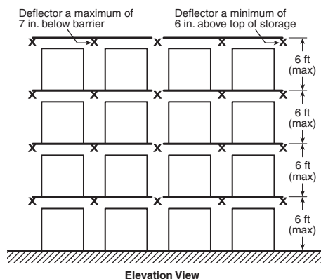
FIGURE 66.16.2.1(b) Single-Row Rack Sprinkler Layout for Design Scheme “B” — Sprinklers on Face of Rack. [30: Figure 16.6.2.1(b)]
