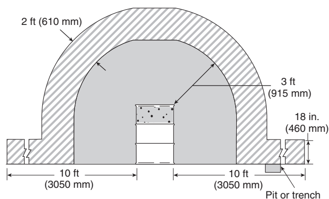
FIGURE 43.1.4.4.4 Class I, Division 2; Class I, Zone 2; Class II, Division 2; or Zone 22 Locations Adjacent to an Enclosed Spray Booth or Spray Room. [33:Figure 6.5.4]
