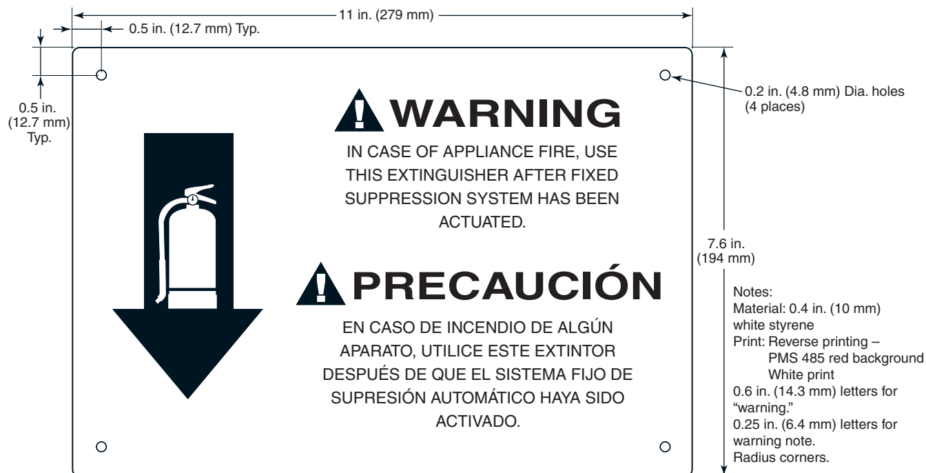
FIGURE A.13.6.7.4.5.3(a) Typical Class K Placard in English and Spanish. [10:Figure A.5.5.5.3(a)]
