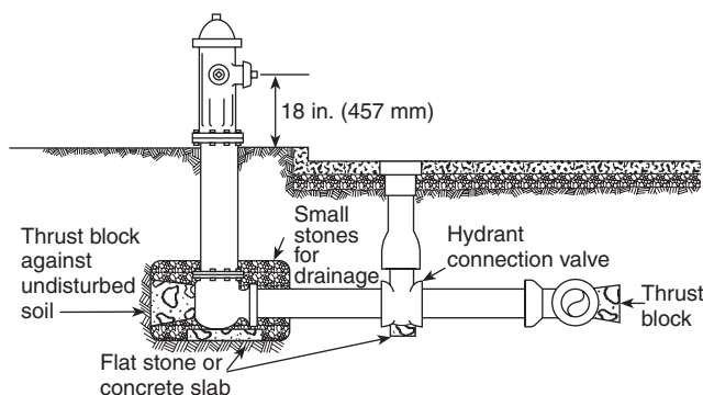
FIGURE A.3.3.122(a) Typical Fire Hydrant Connection. [25:Figure A.3.3.10(a)]
