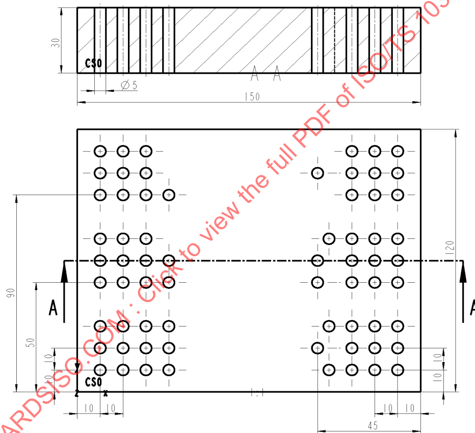
Figure 15 - Rectangular_pattern
