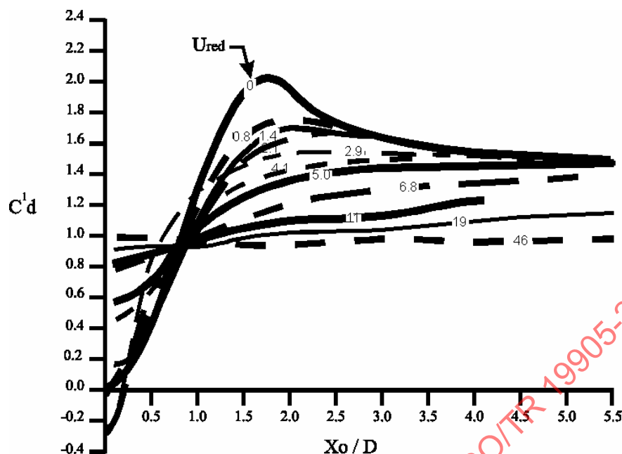
Figure TR.7.3.3.2-1 — Oscillating drag coefficient vs. motion amplitude to diameter ratio X_0/D for given reduced velocities [7-45]
