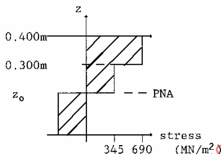
Figure TR.A.12.3-2 — Fully plastic stress distribution
