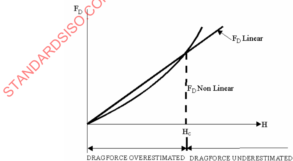
Figure TR.7.3.3.3-3 — Linearization with respect to wave height [7-54]
