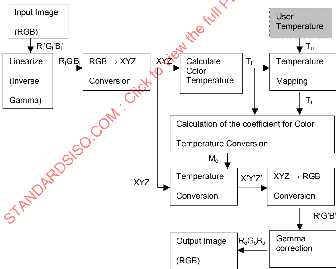
Figure AMD1-1 — Block diagram for the color temperature conversion
