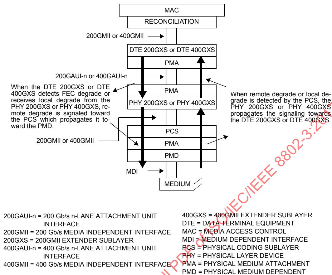
Figure 116-8—Remote Degrade signaling with Extender Sublayer
