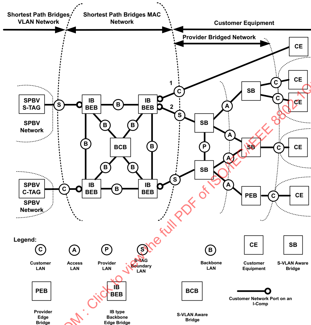
Figure 27-7—SPT Bridge Network using SPBM example
