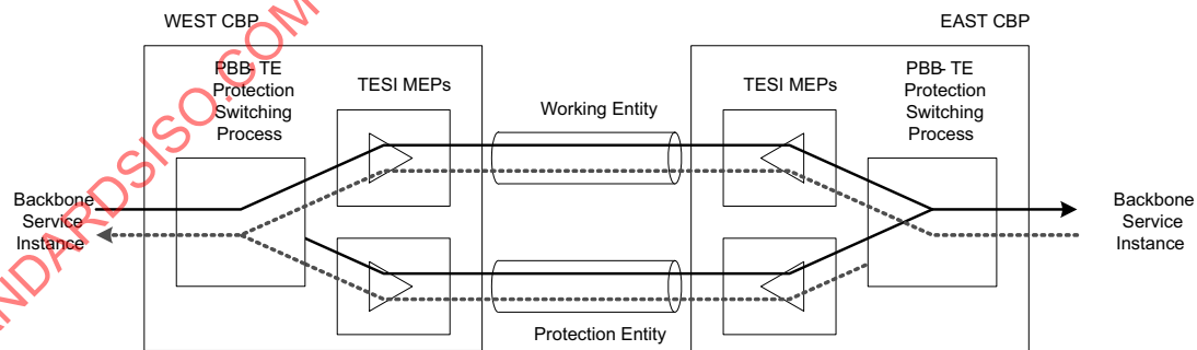
Figure 26-11—Protection switching architecture
