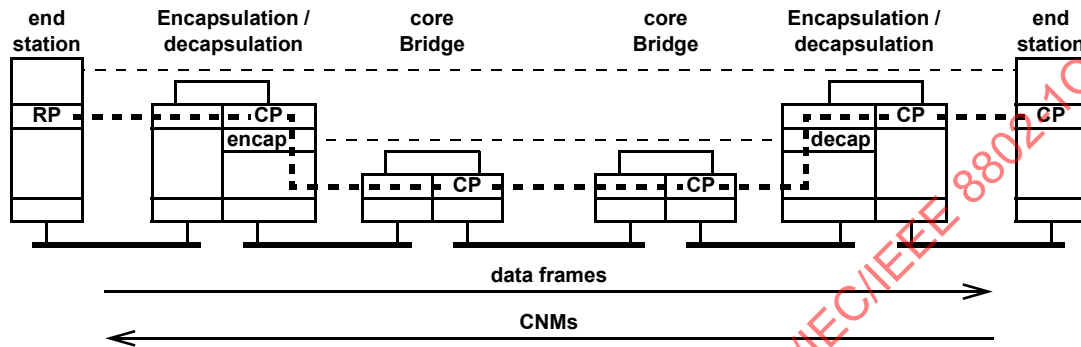
Figure 32-3—CP-RP peering in any hierarchical Bridged Network
