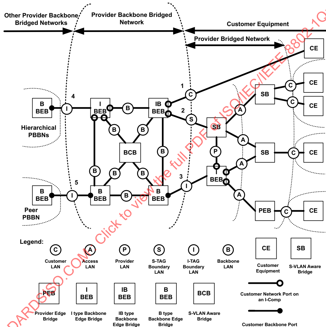
Figure 26-1—PBBN example
