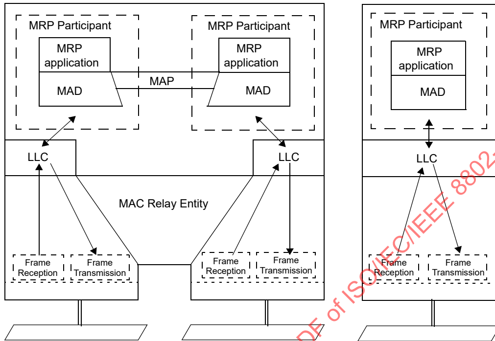
Figure 10-4—MRP architecture
