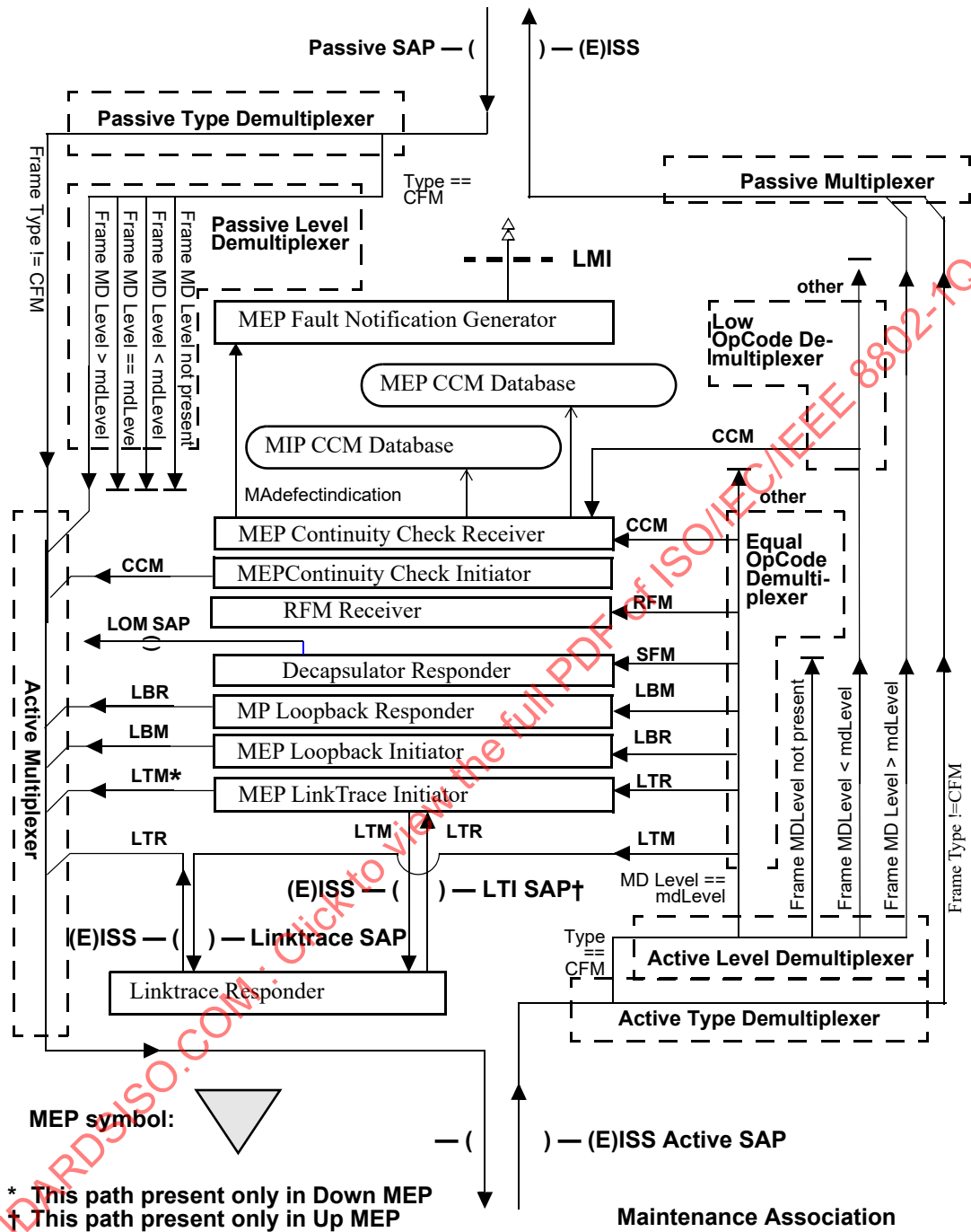
Figure 19-2—MA Endpoint (MEP)
