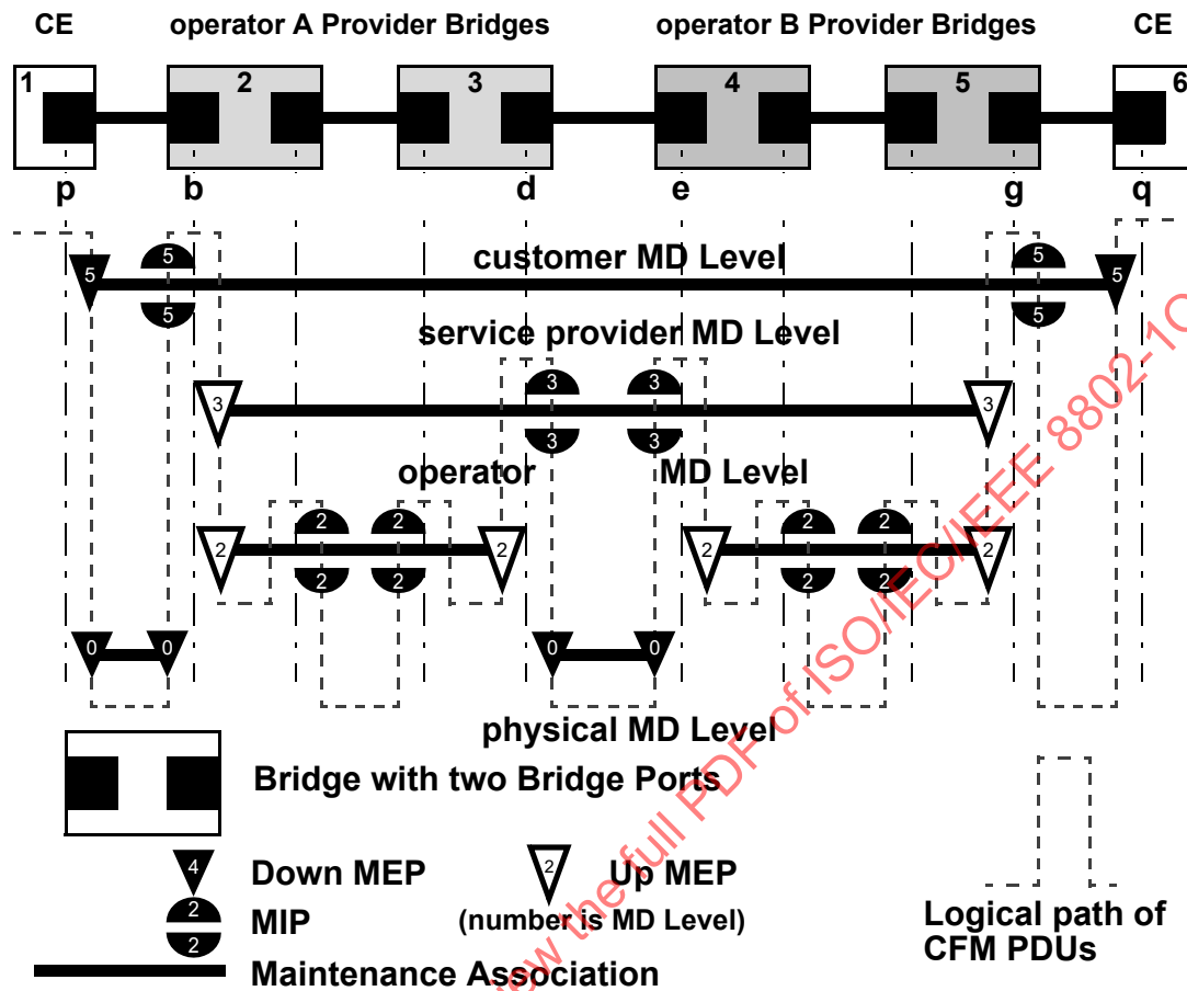
Figure 18-7—MEPs, MIPs, and MD Levels
