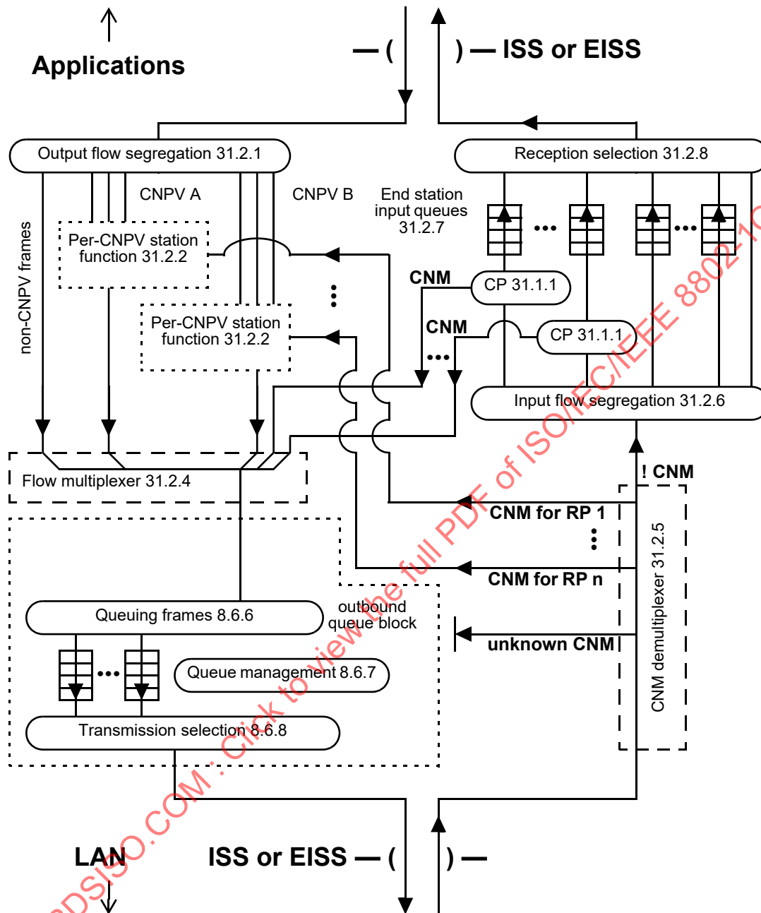
Figure 31-2—Congestion-aware queue functions in an end station
