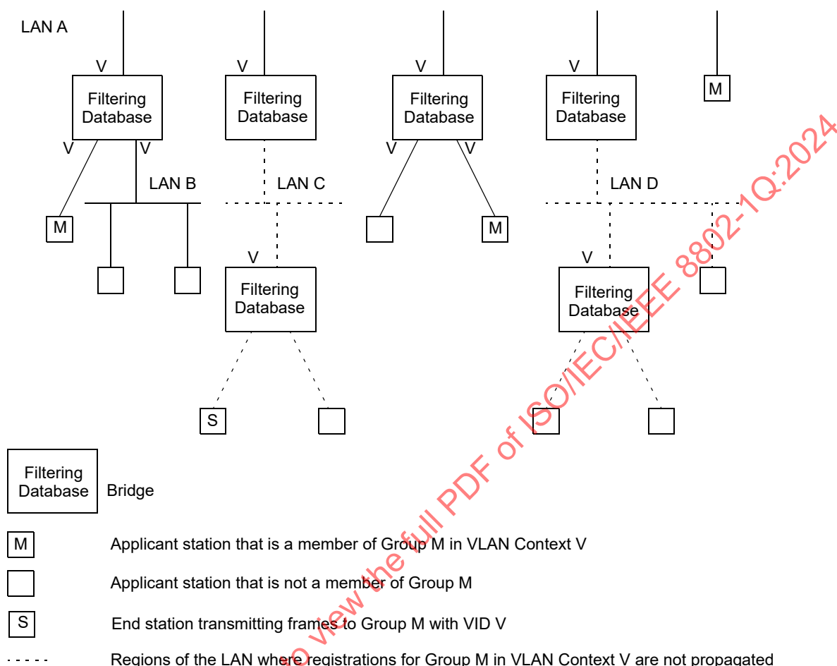
Figure 10-8—Example of MMRP propagation in a VLAN Context
