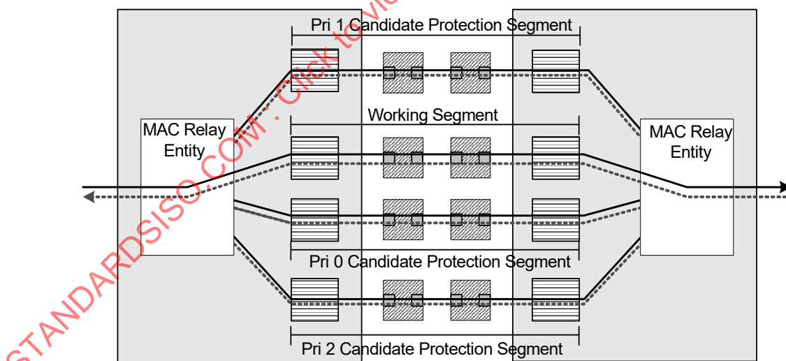
Figure 26-23—M:1 IPS
