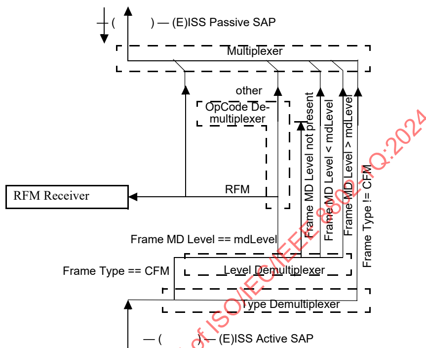
Figure 29-5—RFM Receiver on a non-MP
