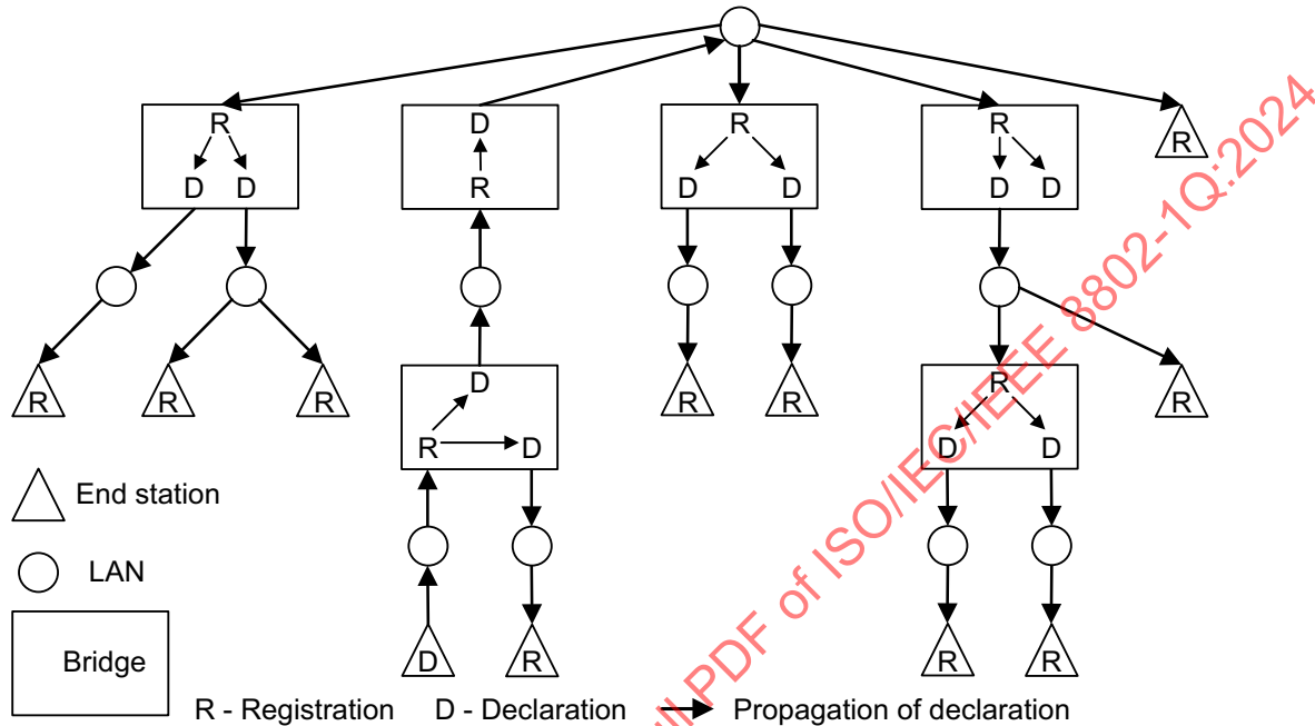
Figure 10-1—Example—Attribute value propagation from one station
