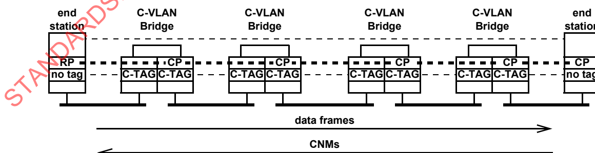
Figure 30-5—CP–RP peering in VLAN Bridged Network
