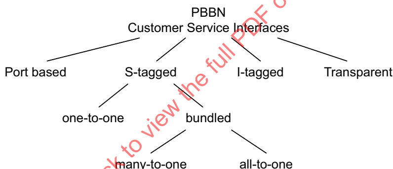
Figure 25-3—Customer service interface types
