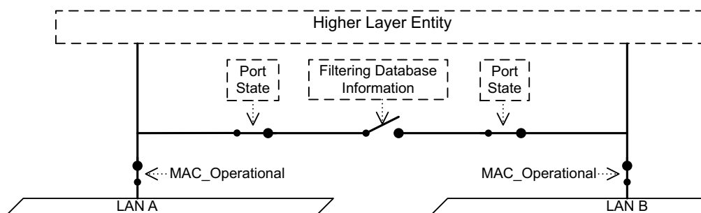
Figure 8-24—Per-Port points of attachment
