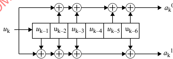
Figure 22-3—LECIM DSSS PHY convolutional encoder
