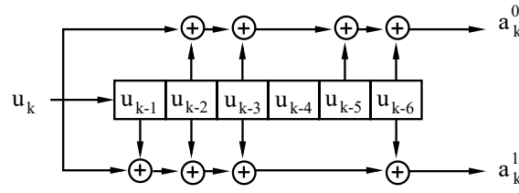
Figure 21-10—Convolutional encoder
