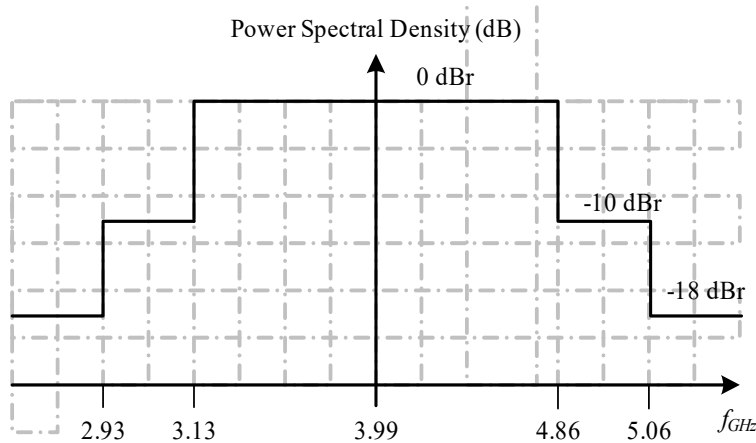
Figure 15-14—Transmit spectrum mask for band 4
