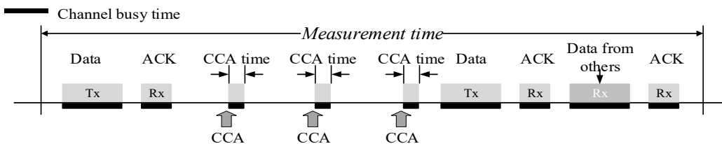
Figure 6-82—Channel Utilization
