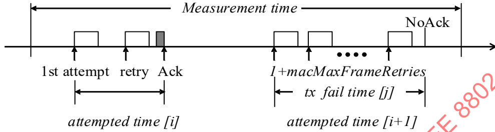
Figure 6-79— maxTxFailTime
