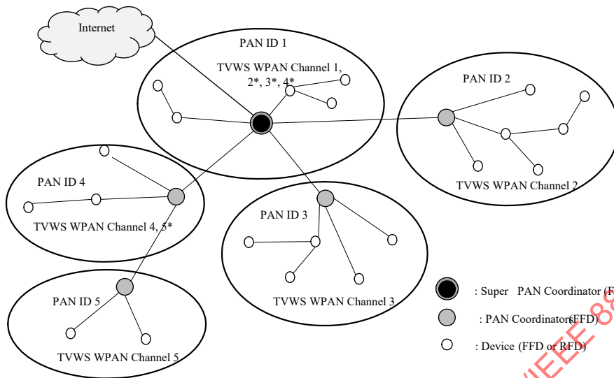
Figure 5-3—Example of TVWS multichannel cluster tree PAN
