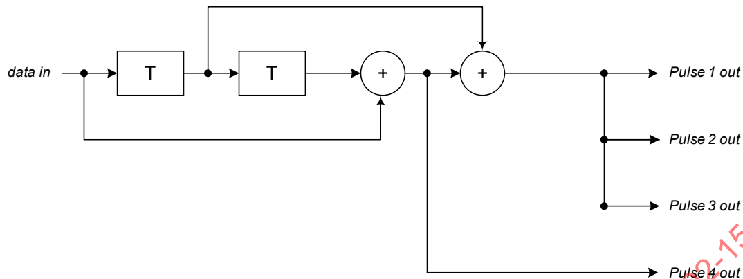
Figure 18-2—Extended mode LRP UWB PHY transmitter convolution code
