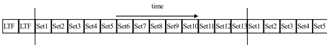
Figure 20-10—Pilot tone sets for Option 1
