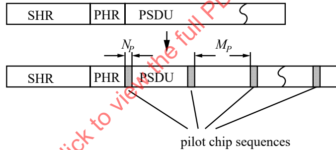
Figure 21-16—PSDU pilot insertion
