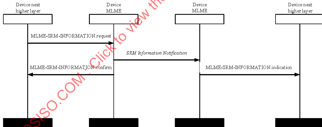
Figure 6-87—SRM Report flow
