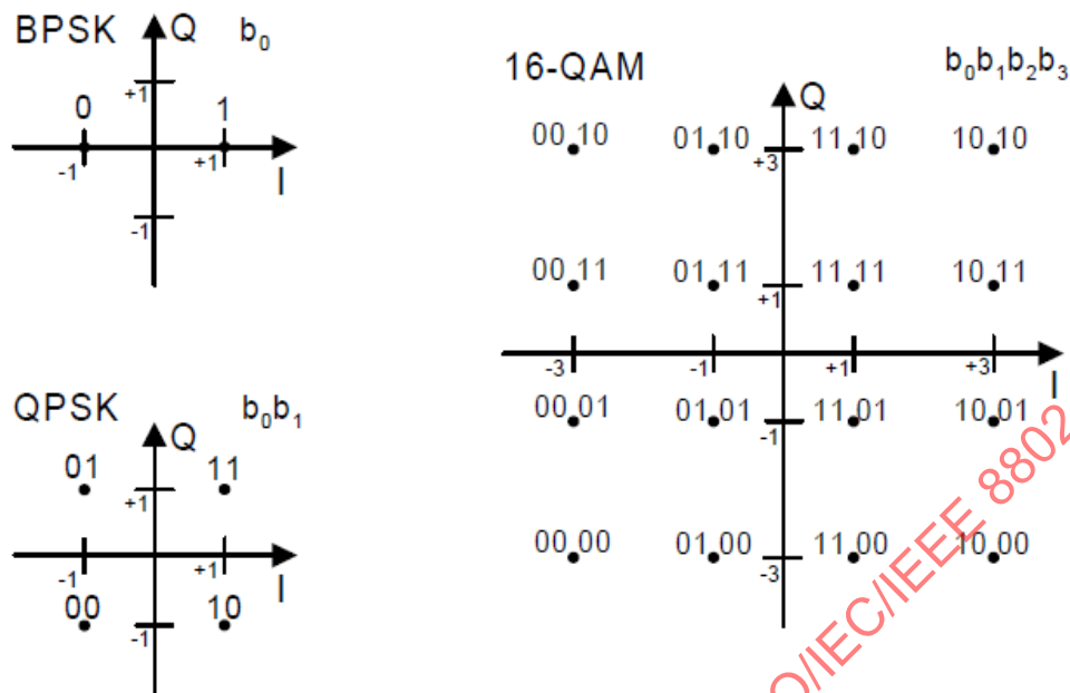
Figure 20-7—Bit-to-symbol mapping for SUN OFDM
