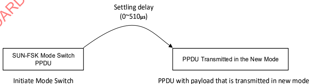
Figure 19-16—Transmitting sequence between SUN FSK mode switch PPDU and the new mode PPDU
