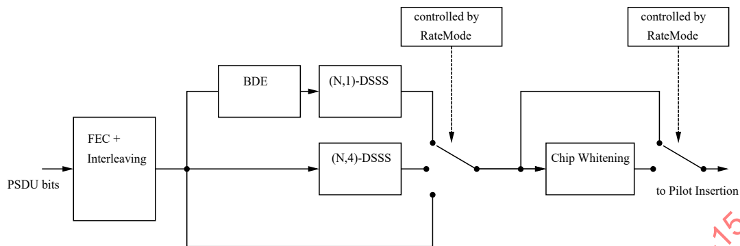
Figure 21-8—PSDU processing for DSSS
