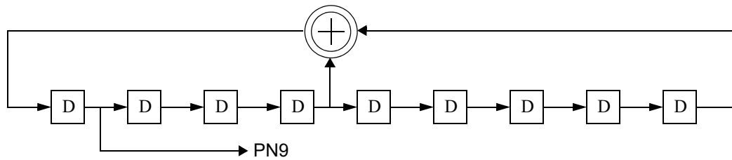
Figure 16-2—Schematic of the PN generator
