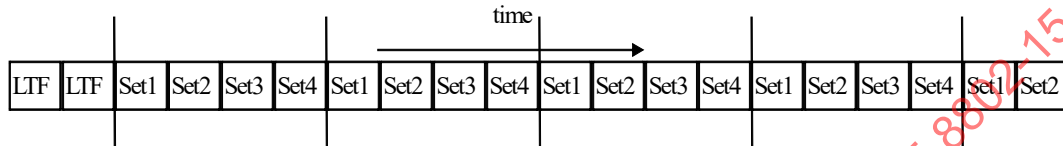
Figure 20-12—Pilot tone sets for Option 4
