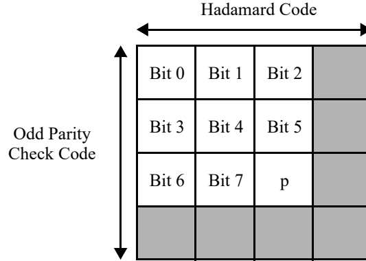
Figure 21-14—Structure of turbo product codeword
