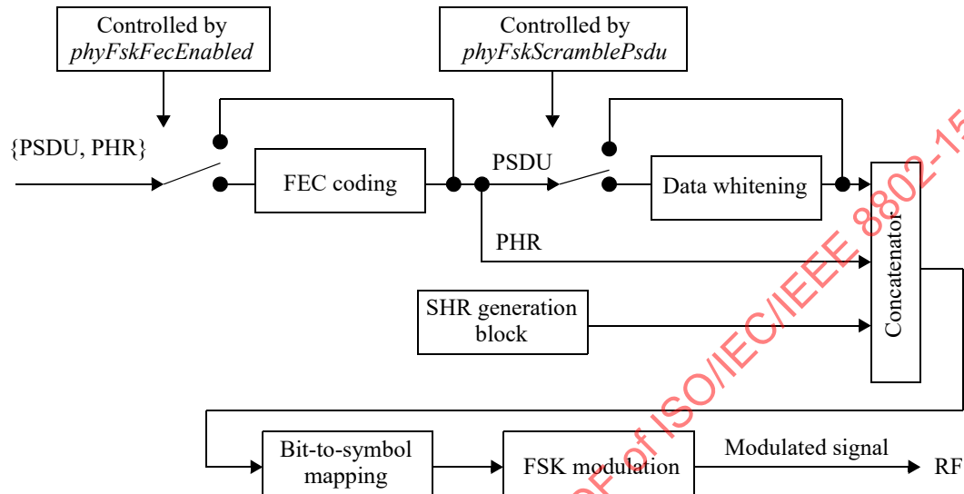
Figure 19-7—SUN FSK reference modulator
