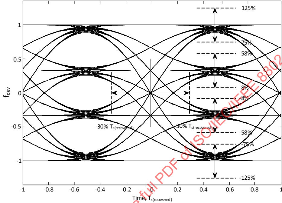
Figure 19-9—Eye diagram for 4-FSK
