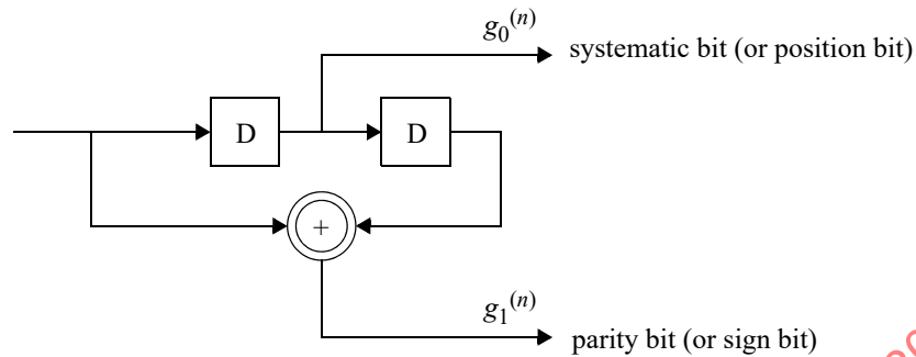
Figure 15-11—Systematic convolutional encoder
