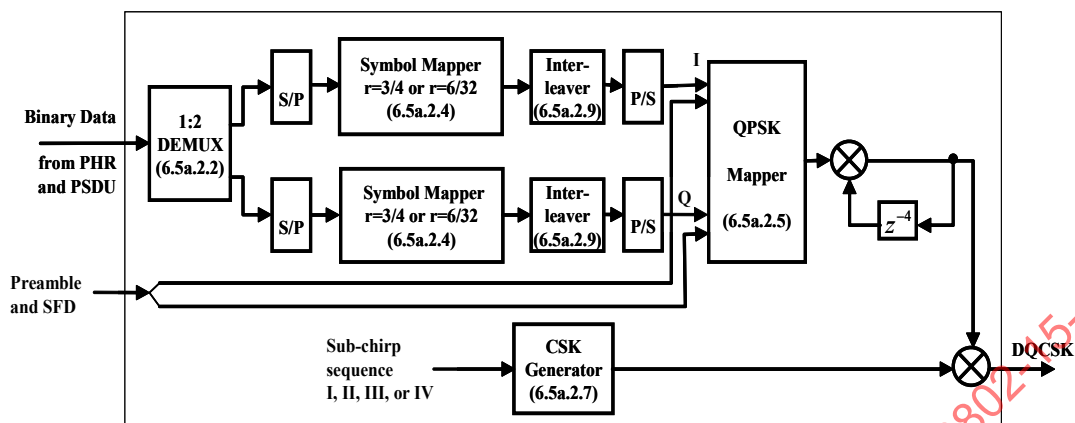
Figure 14-4—Differential bi-orthogonal quaternary-chirp-shift-keying modulator and spreading ( r = 3/4 for 8-ary 1 Mb/s, r = 3/16 for 64-ary 250 kb/s)
