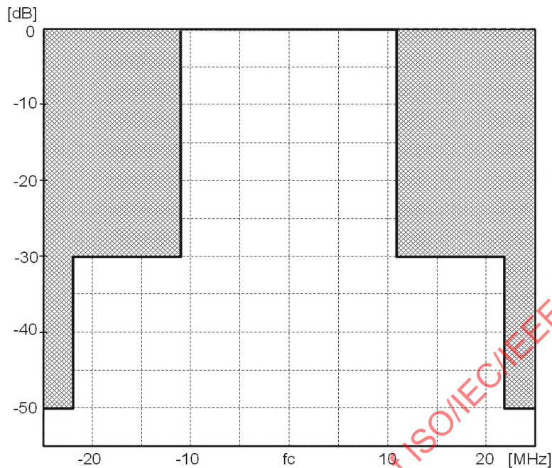
Figure 14-8—Transmit PSD mask
