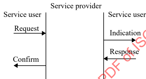
Figure 5-9—Service primitives
