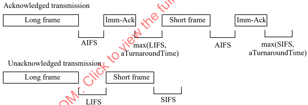
Figure 6-4—IFS usage
