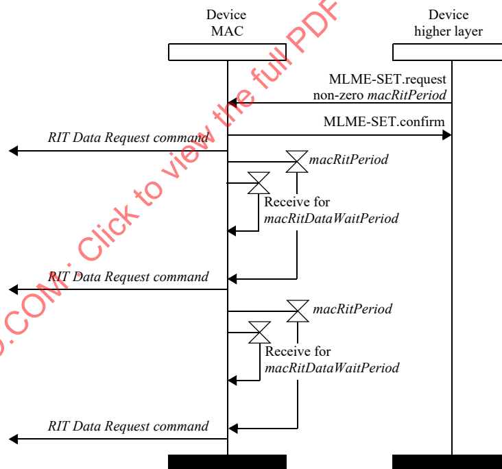
Figure 6-67—Message sequence chart for starting RIT mode
