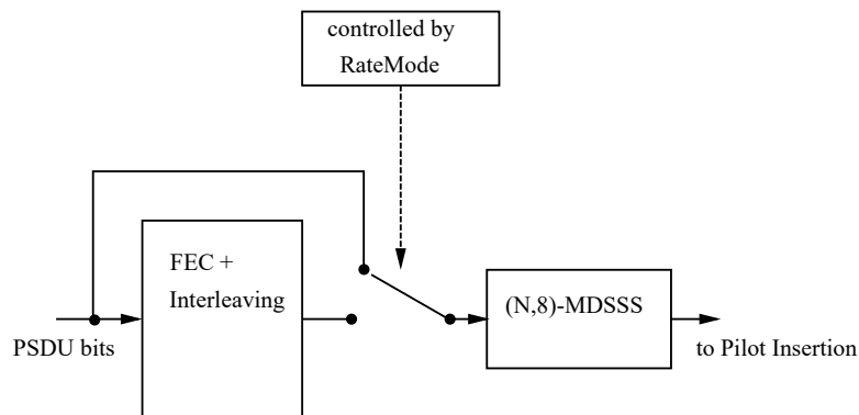
Figure 21-9—PSDU processing for MDSSS
