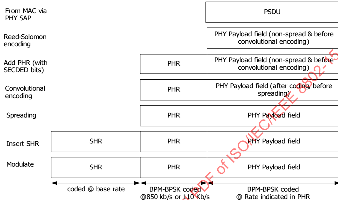
Figure 15-2—HRP UWB PPDU encoding process
