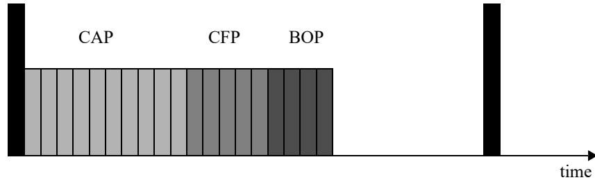
Figure 5-6—TMCTP superframe extension
