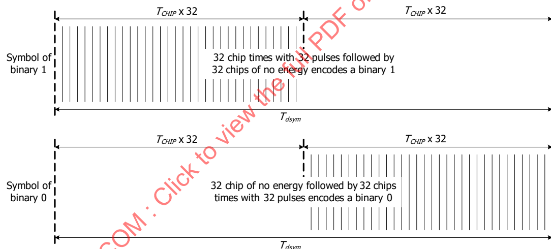
Figure 18-4—Long-range mode LRP UWB PHY symbol structure
