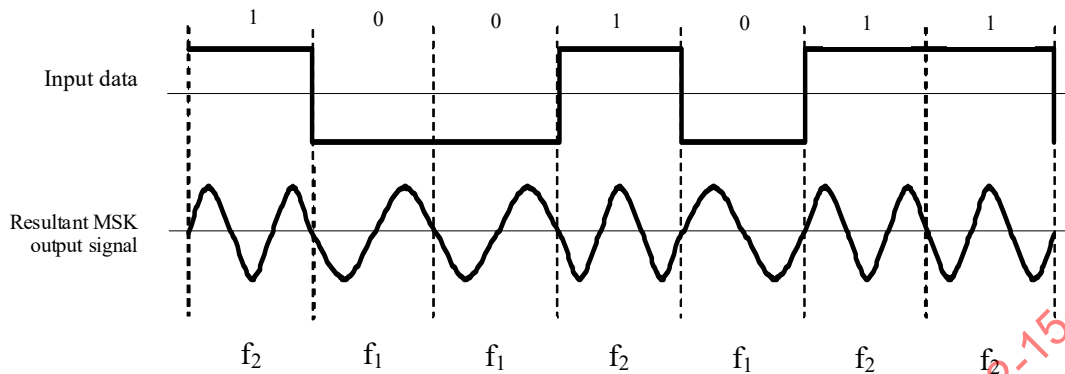
Figure 17-4—Example signal using MSK modulation in the time domain
