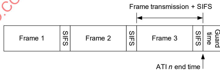
Figure 6-37—SIFS and guard time at the end of an ATI—no Ack requested
