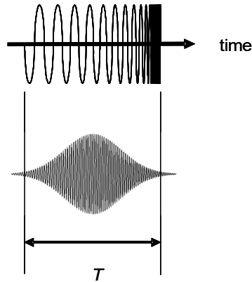
Figure 15-15—Graphical view of a CoU pulse
