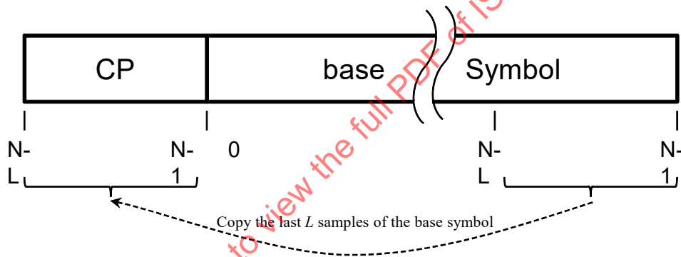
Figure 20-13—Cyclic prefix (CP)
