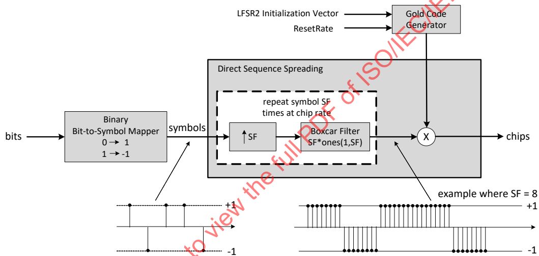
Figure 22-4—Bit-to-chip diagram for LECIM DSSS PHY
