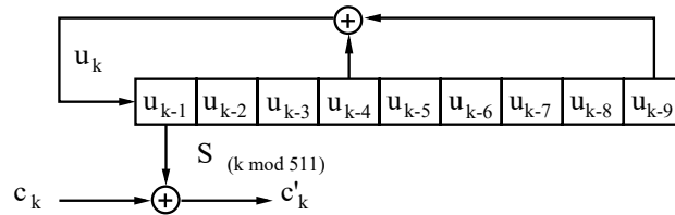
Figure 21-15—Chip whitening
