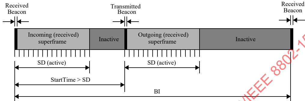
Figure 6-2—The relationship between incoming and outgoing beacons
