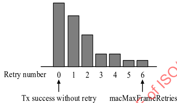
Figure 6-81—Retry Histogram
