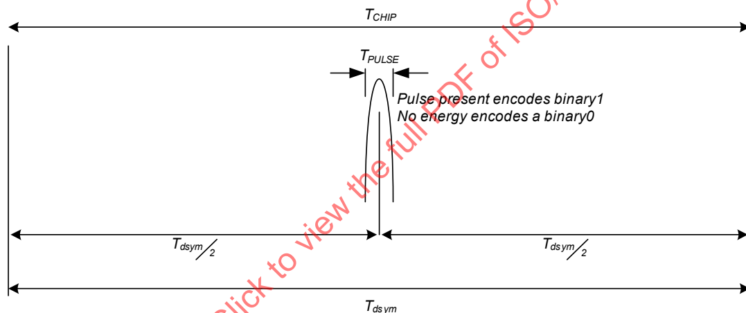
Figure 18-1—Base mode LRP UWB PHY symbol structure
