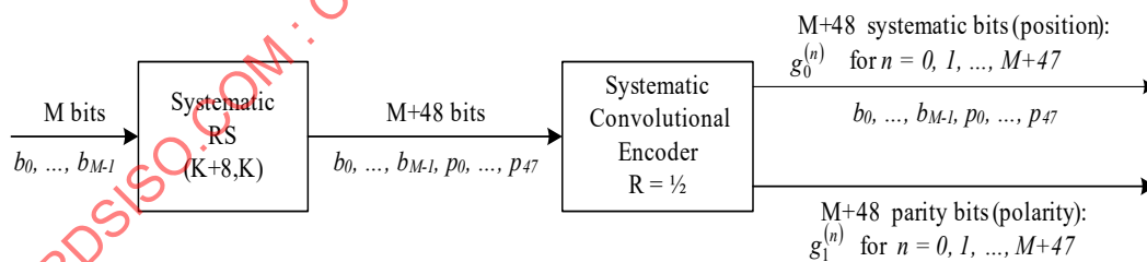
Figure 15-10—FEC encoding process
