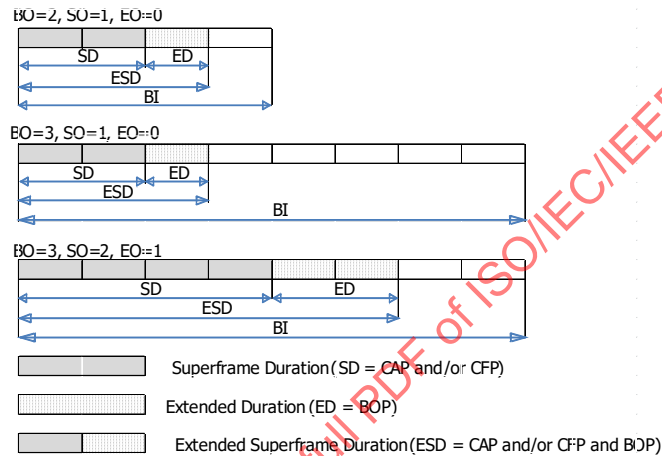
Figure 6-11—An example of the TMCTP superframe structure
