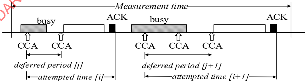
Figure 6-80— macDeferredTxTime
