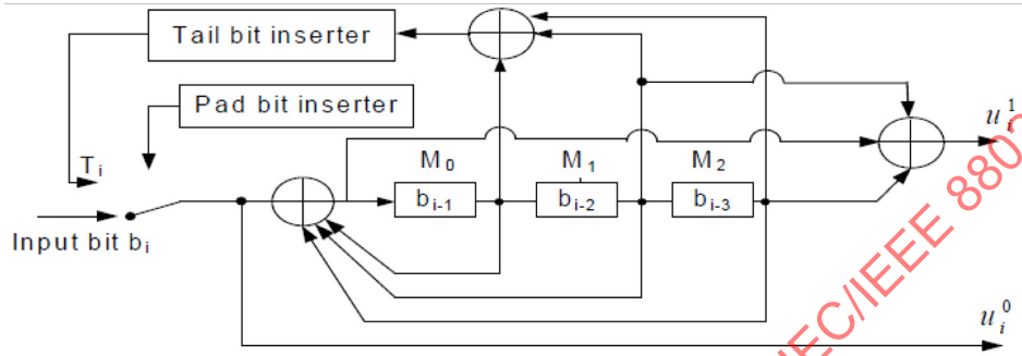
Figure 19-13—The recursive and systematic code (RSC) encoder
