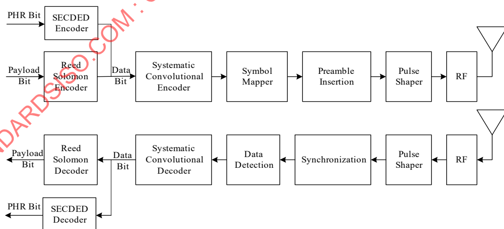
Figure 15-1—HRP UWB PHY signal flow
