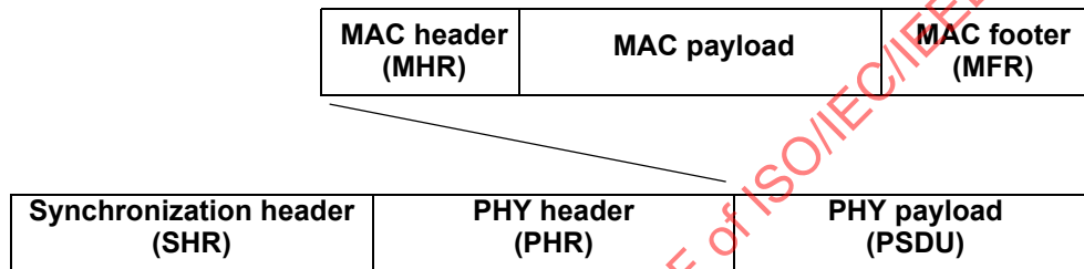
Figure 5-7—Schematic view of the PPDU
