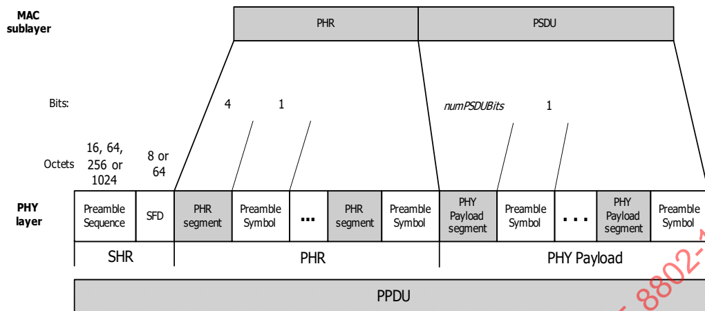
Figure 15-17—Illustration of the modified frame structure with multiplexed preamble
