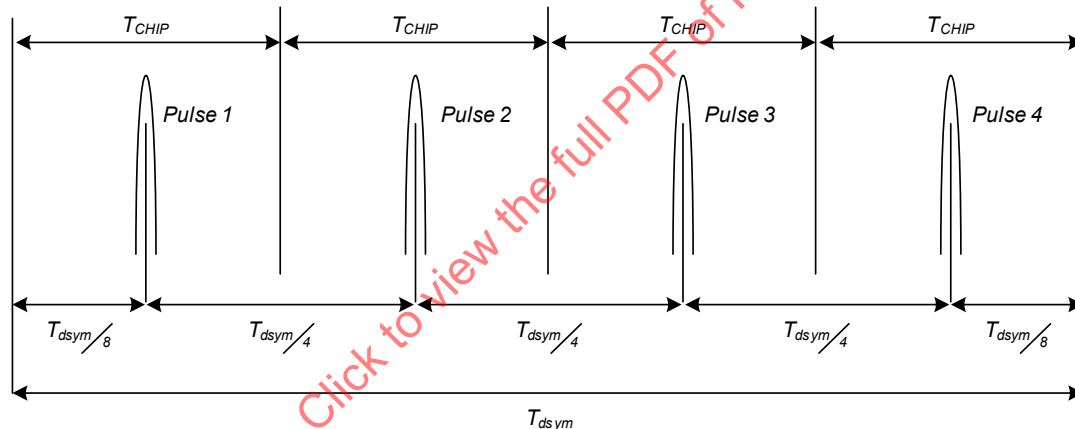
Figure 18-3—Extended mode LRP UWB PHY symbol structure
