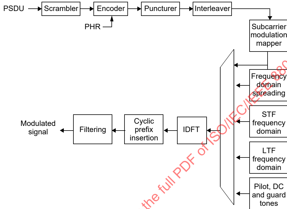
Figure 20-6—Reference modulator diagram for SUN OFDM
