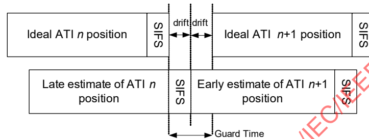
Figure 6-36—Guard time
