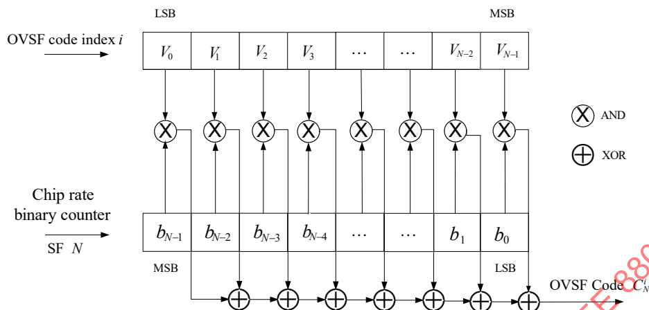
Figure 22-7—Logical level architecture of OVFS code generator for LECIM DSSS PHY
