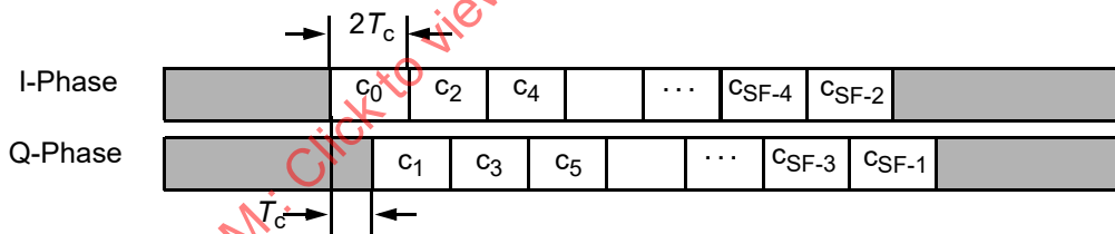
Figure 22-9—O-QPSK chip modulation
