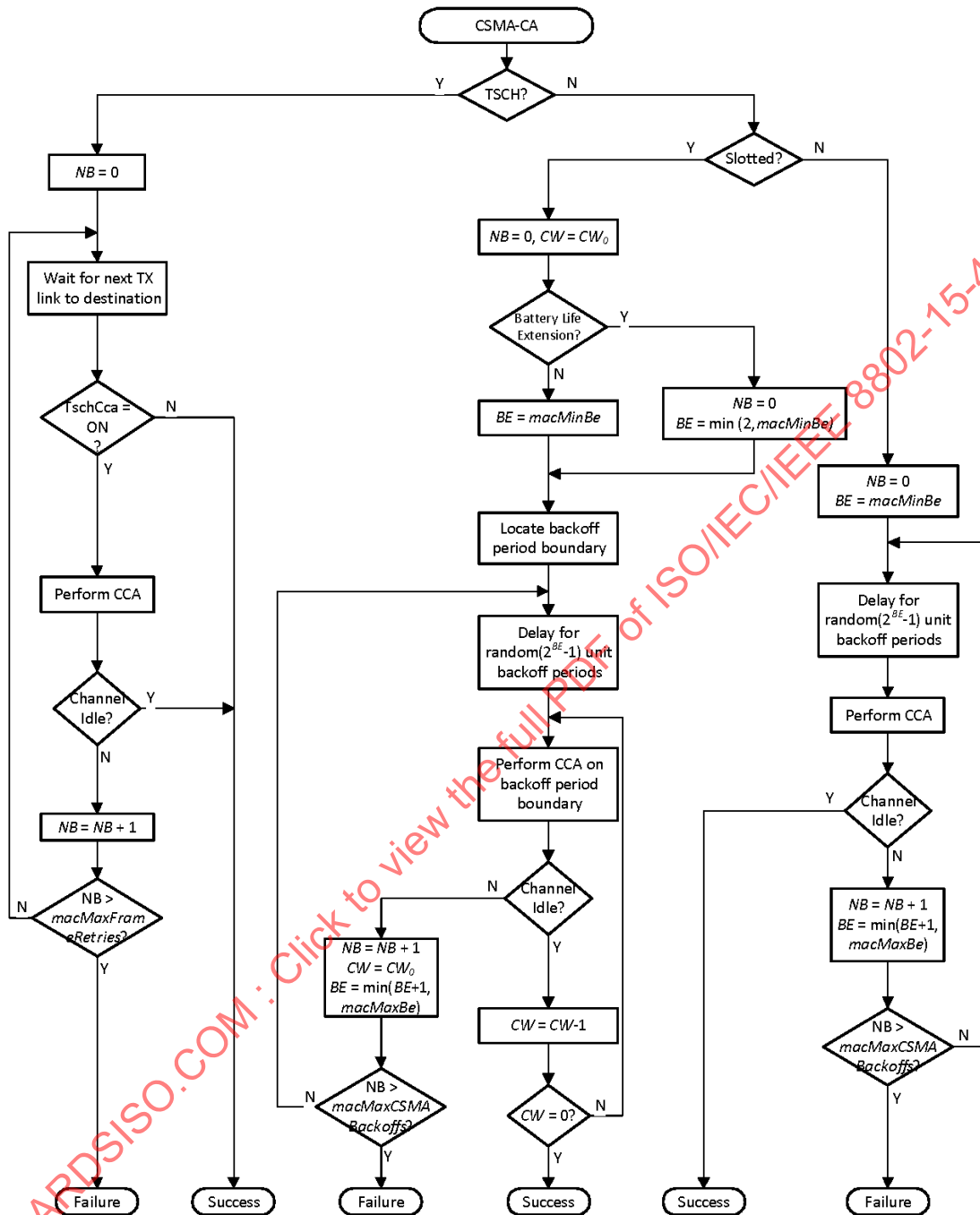
Figure 6-5—CSMA-CA algorithm
