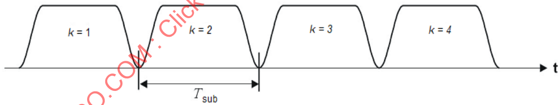
Figure 14-7—Subchirp time-domain pulse shaping
