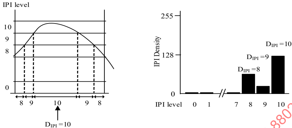
Figure 6-84—IPI Density
