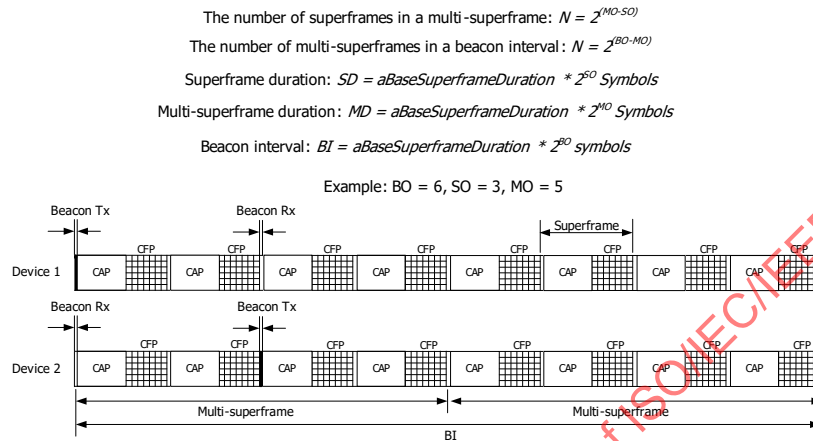
Figure 5-5—General DSME multi-superframe structure
