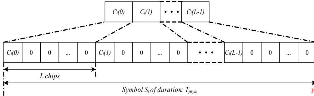
Figure 15-5—Construction of symbol S_i from code C_i
