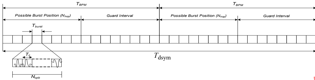
Figure 15-3—HRP UWB PHY symbol structure
