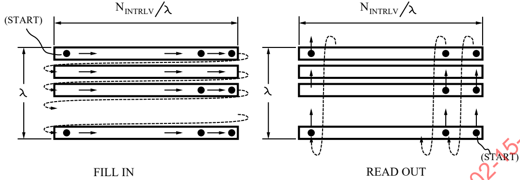
Figure 21-12—Interleaver
