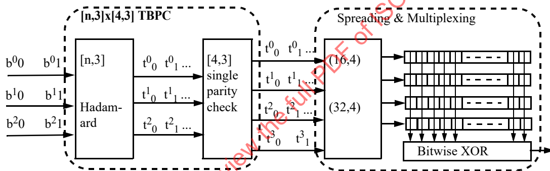
Figure 21-13—MDSSS signal flow
