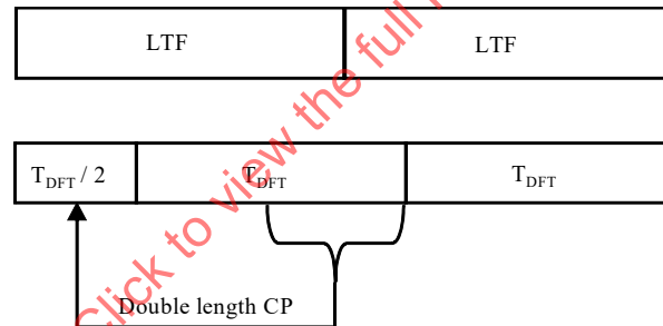
Figure 20-4—Structure of LTF for SUN OFDM
