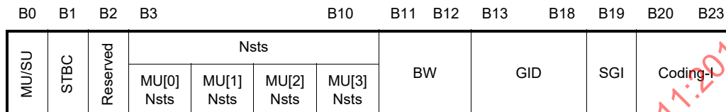
Figure 23-13—SIG-A1 structure for MU PPDU
