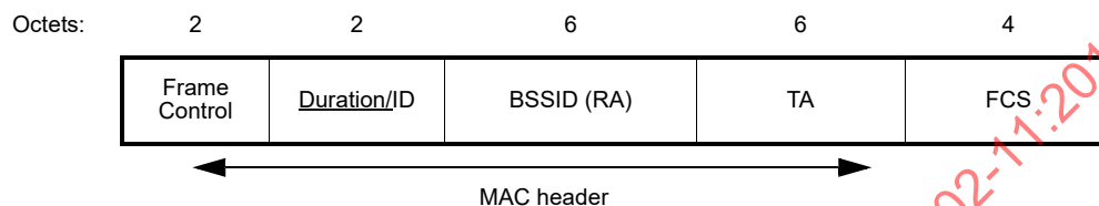
Figure 9-23—PS-Poll frame
