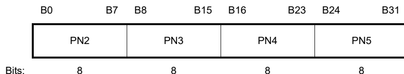
Figure 9-589cg—BPN subfield
