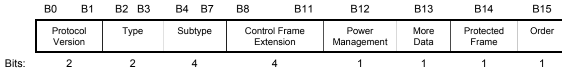
Figure 8-2a—Frame Control field when Type is equal to 1 and Subtype is equal to 6
