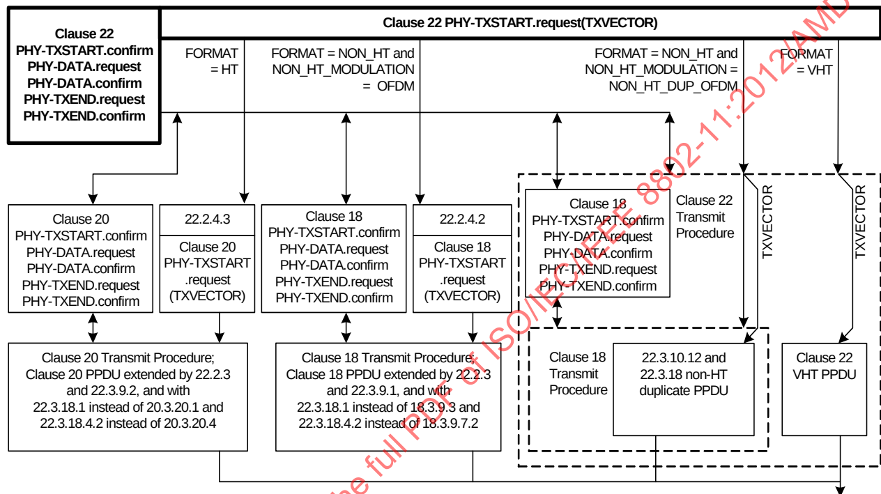
Figure 22-1— PHY interaction on transmit for various PPDU formats
