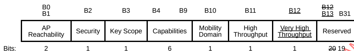
Figure 8-216—BSSID Information field
