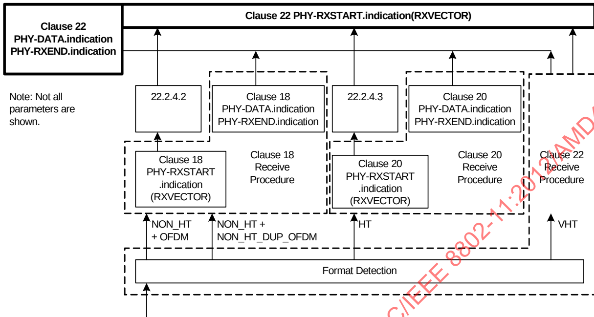
Figure 22-2—PHY interaction on receive for various PPDU formats
