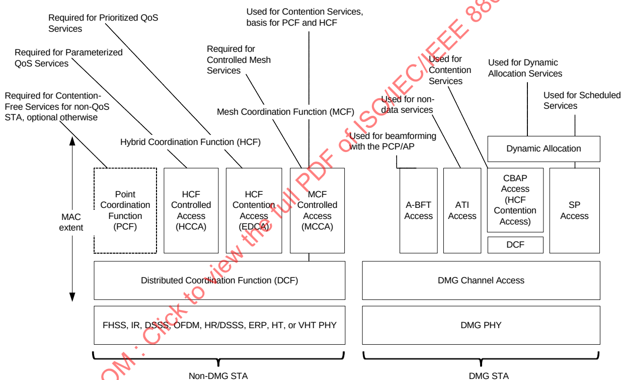
Figure 9-1—MAC architecture
