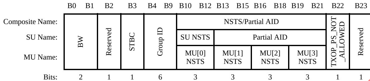
Figure 22-18—VHT-SIG-A1 structure
