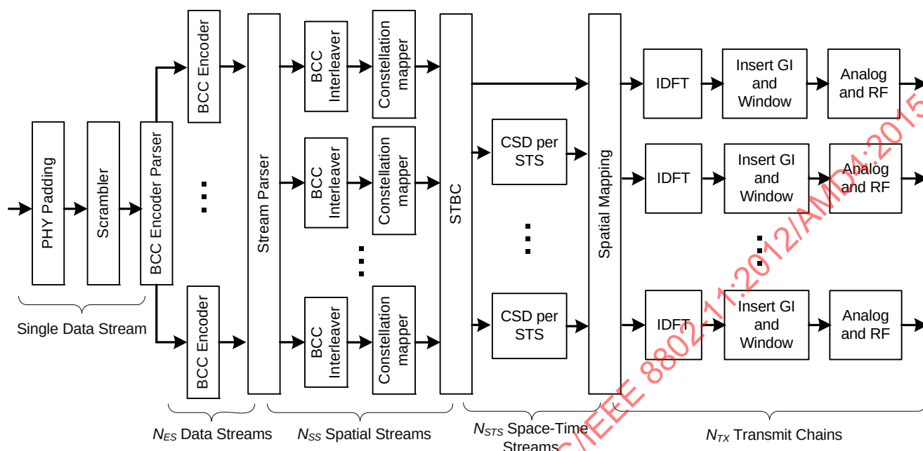
Figure 22-10—Transmitter block diagram for the Data field of a 20 MHz, 40 MHz, or 80 MHz VHT SU PPDU with BCC encoding
