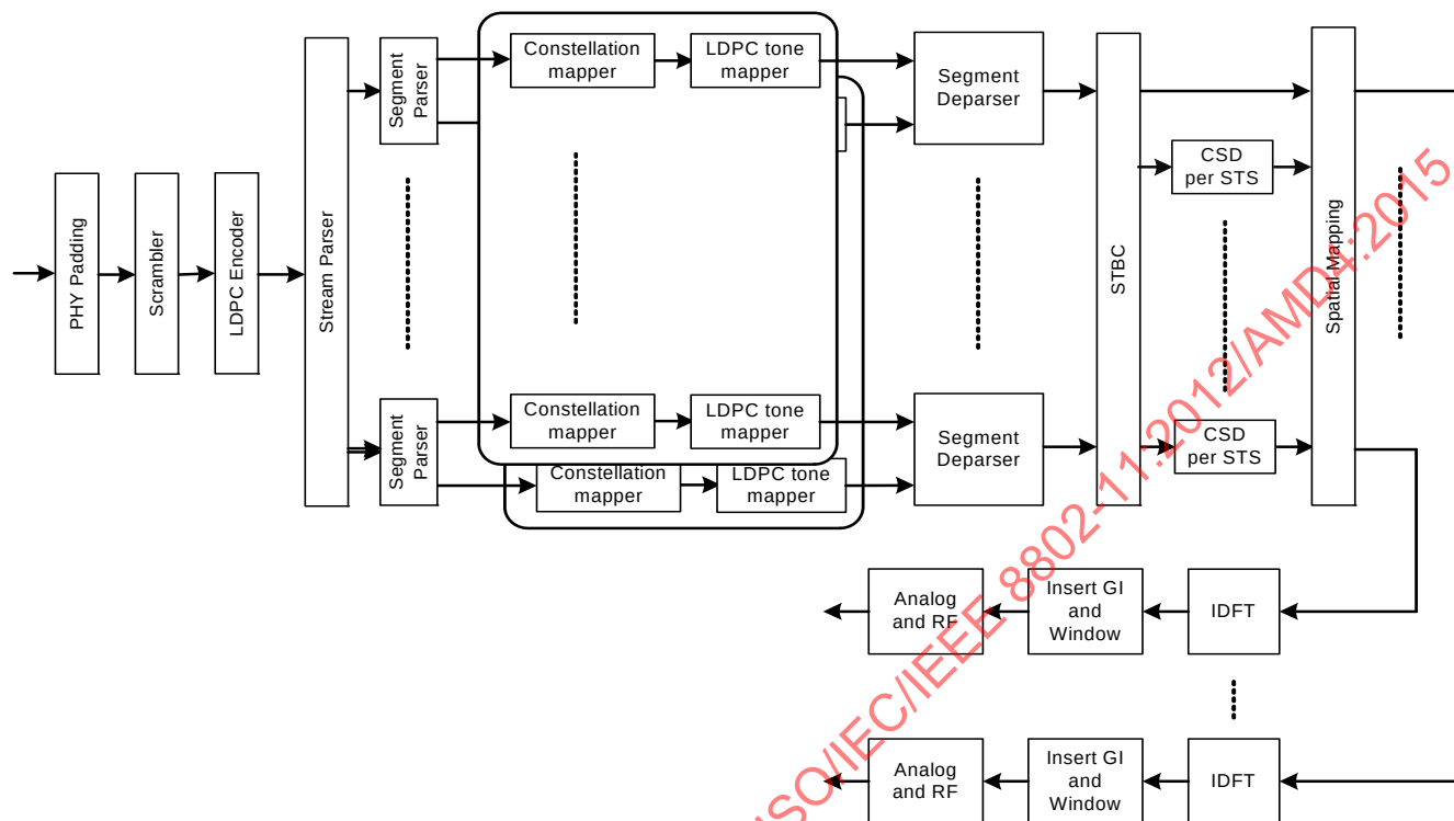
Figure 22-14—Transmitter block diagram for the Data field of a 160 MHz VHT SU PPDU with LDPC encoding
