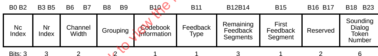
Figure 8-80d—VHT MIMO Control field
