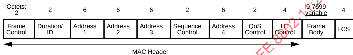
Figure 8-30—Data frame
