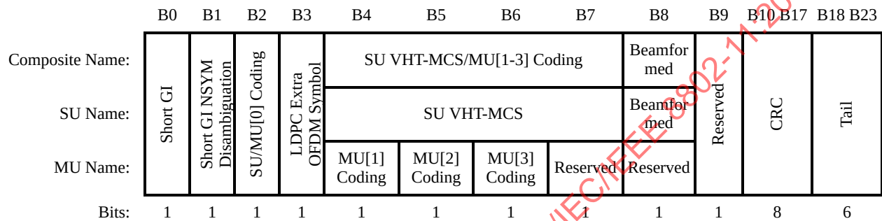
Figure 22-19—VHT-SIG-A2 structure
