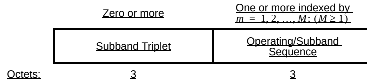
Figure 8-90c—Triplet field if dot11OperatringClassRequired is true
