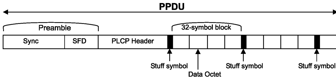
Figure 76—PLCP data whitener format
