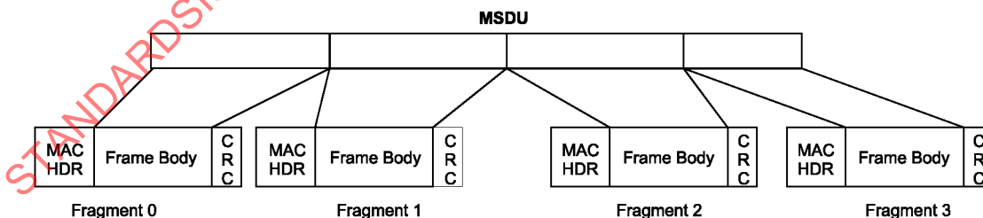
Figure 52—Fragmentation
