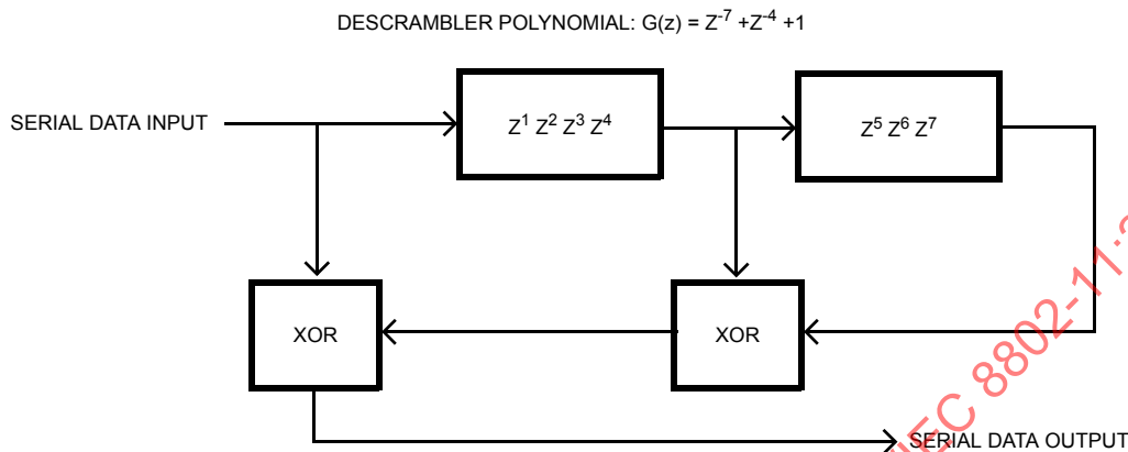
Figure 136—Data descrambler
