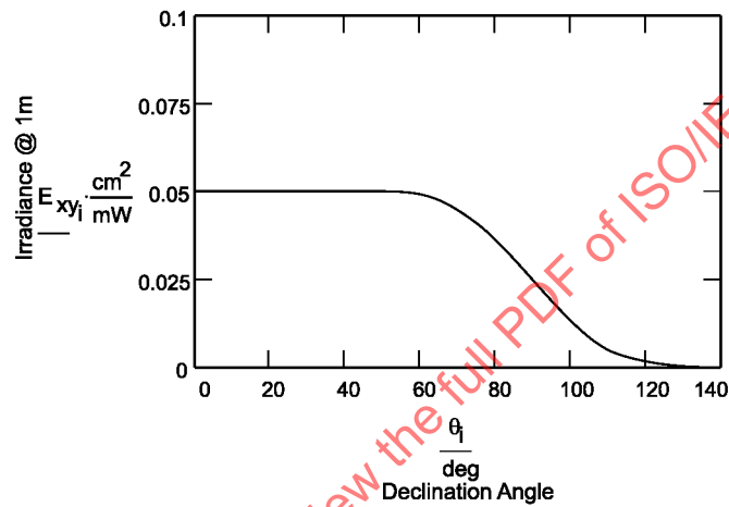
Figure 108—Emitter radiation pattern mask 2
