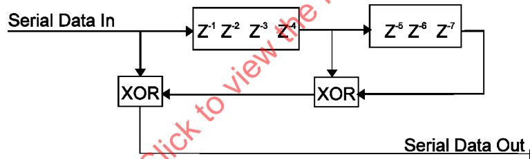
Figure 94—Data descrambler
