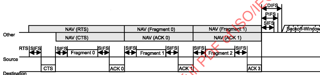
Figure 59—RTS/CTS with fragmented MSDU
