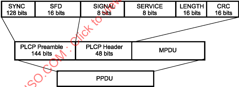
Figure 90—PLCP frame format
