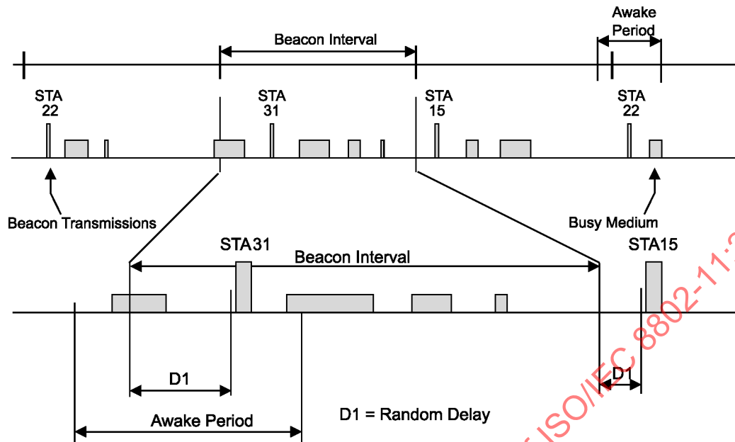
Figure 69—Beacon transmission in an IBSS
