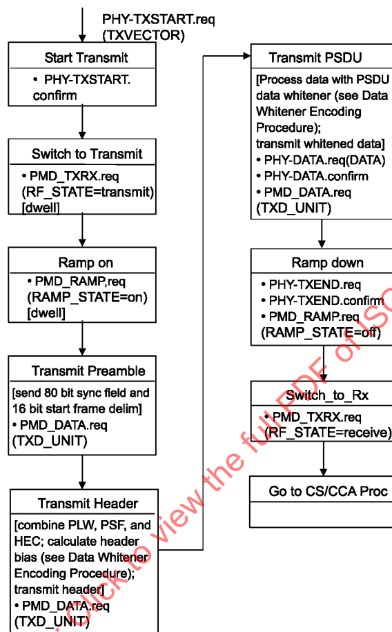
Figure 78—Transmit state machine
