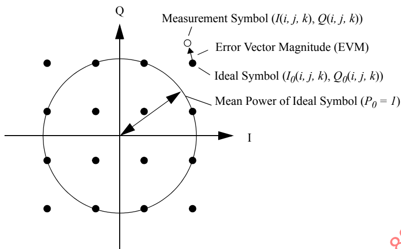
Figure 125—Constellation error
