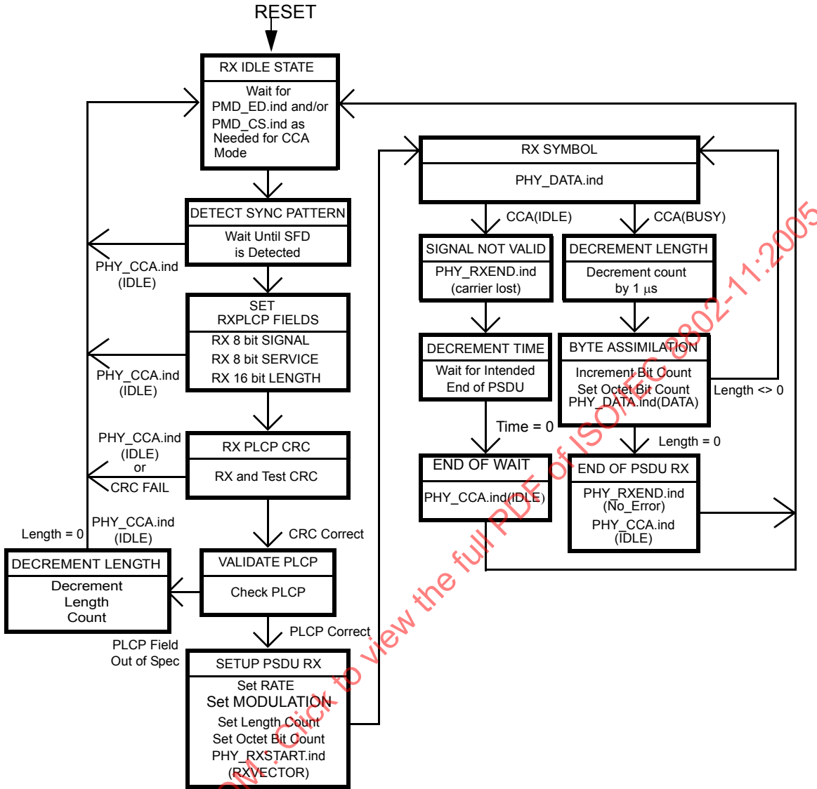
Figure 140—PLCP receive state machine
