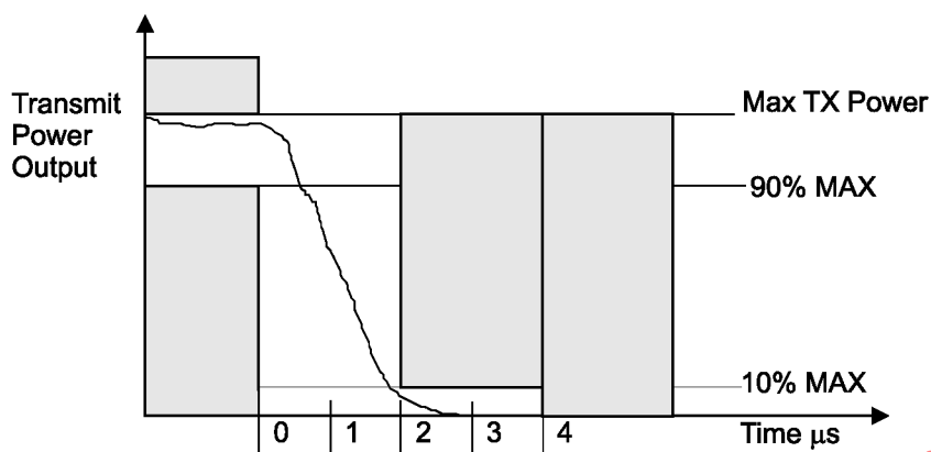
Figure 102—Transmit power-down ramp
