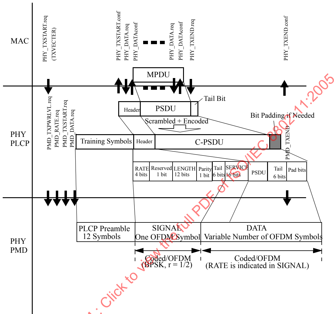
Figure 126—Transmit PLCP
