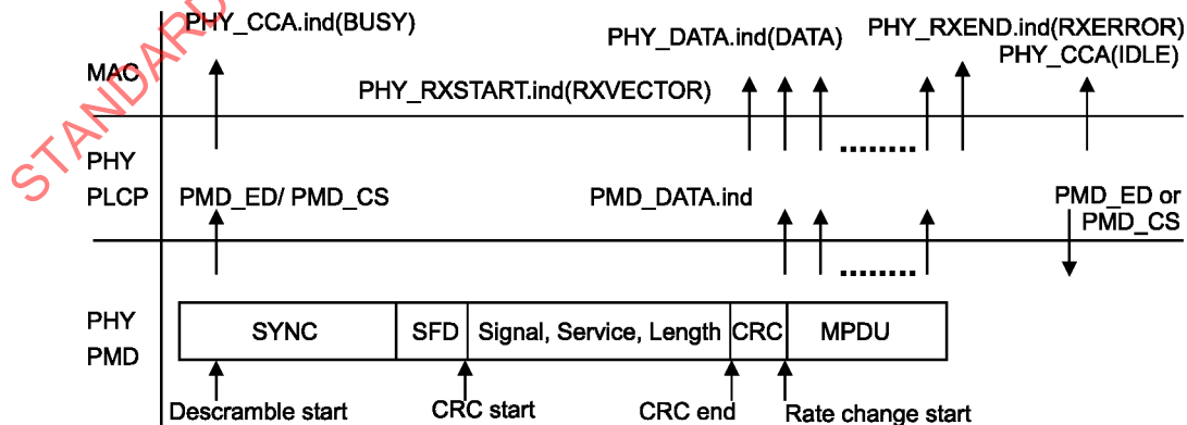
Figure 97—Receive PLCP
