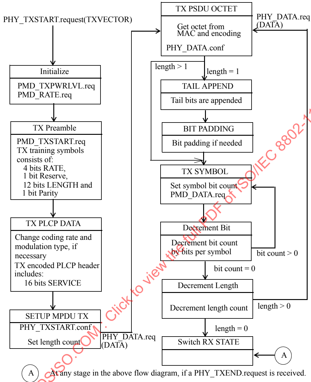
Figure 127—PLCP transmit state machine
