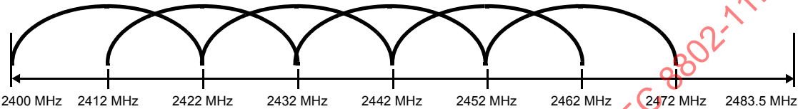
Figure 146—North American channel selection—overlapping
