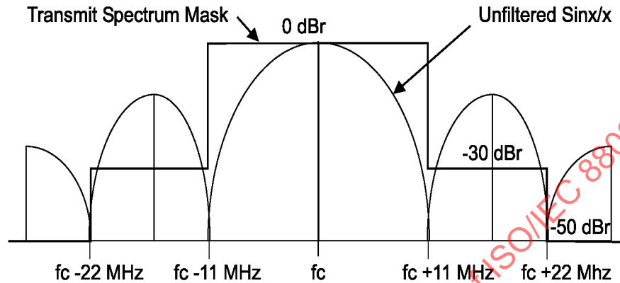
Figure 149—Transmit spectrum mask
