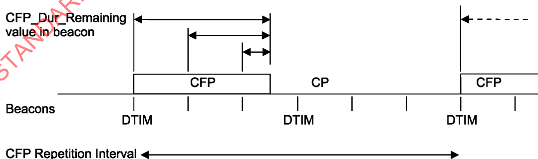
Figure 64—Beacons and CFPs
