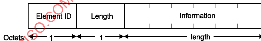
Figure 34—Element format
