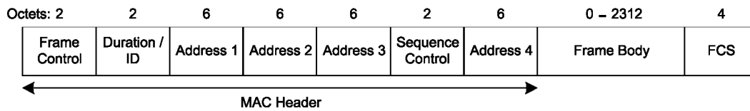
Figure 22—Data frame
