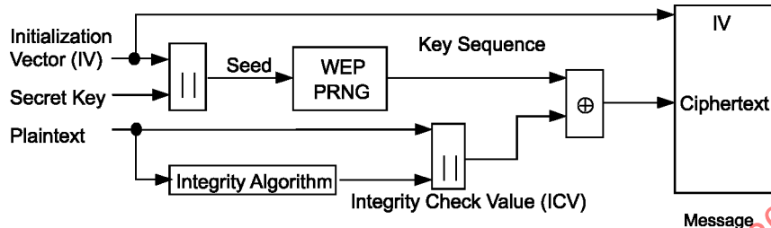
Figure 48—WEP encipherment block diagram
