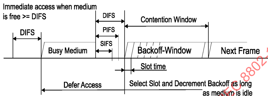
Figure 55—Basic access method
