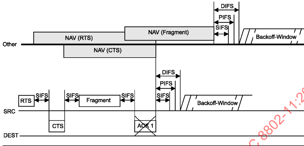
Figure 60—RTS/CTS with transmitter priority and missed acknowledgment
