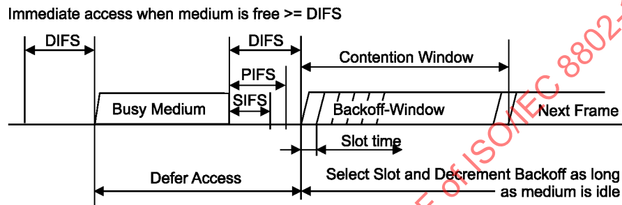
Figure 53—Some IFS relationships
