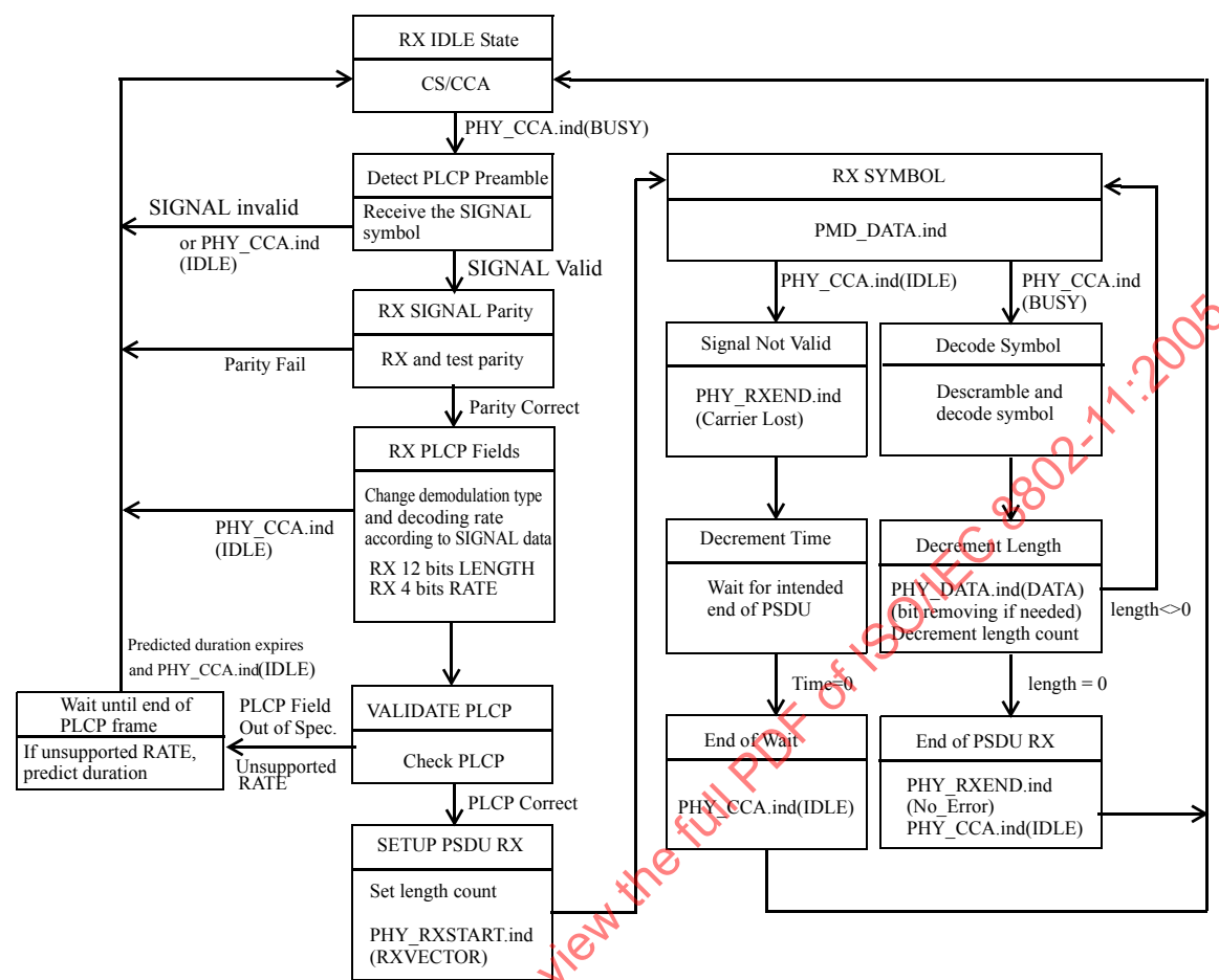
Figure 129—PLCP receive state machine
