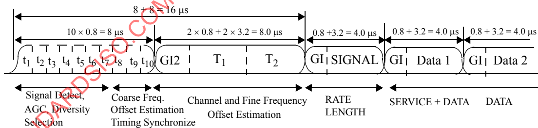
Figure 114—OFDM training structure
