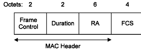
Figure 17—CTS frame
