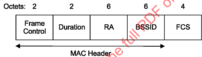
Figure 20—CF-End frame
