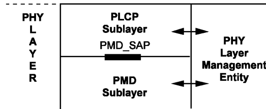
Figure 87—PMD layer reference model
