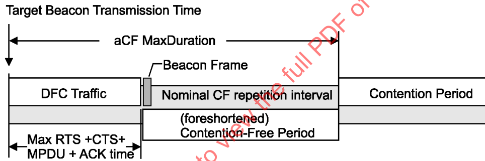
Figure 65—Example of delayed beacon and foreshortened CFP
