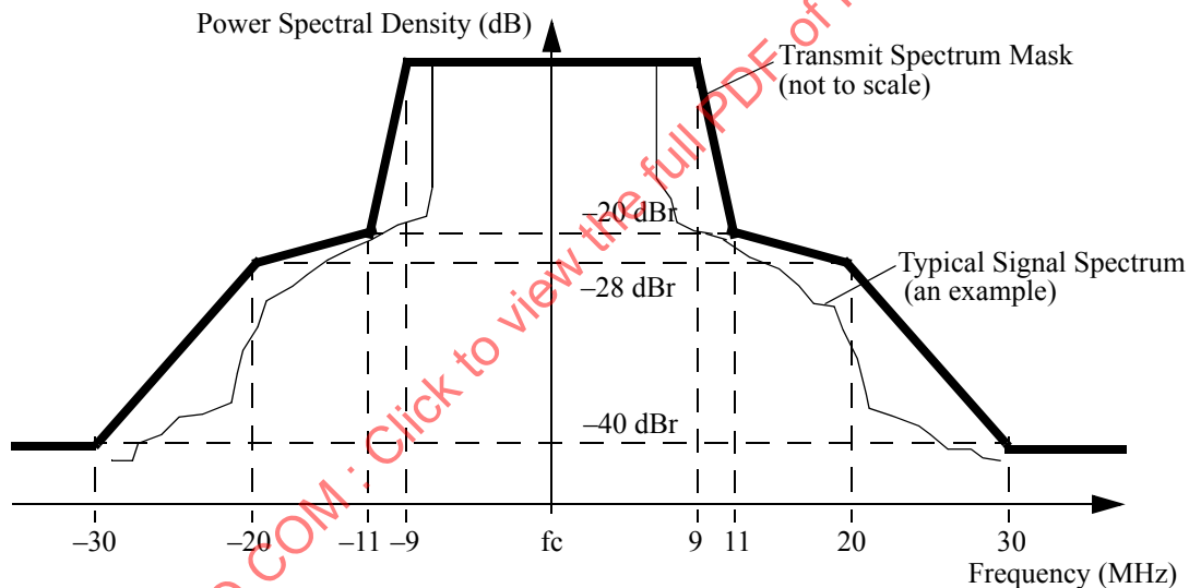
Figure 124—Transmit spectrum mask
