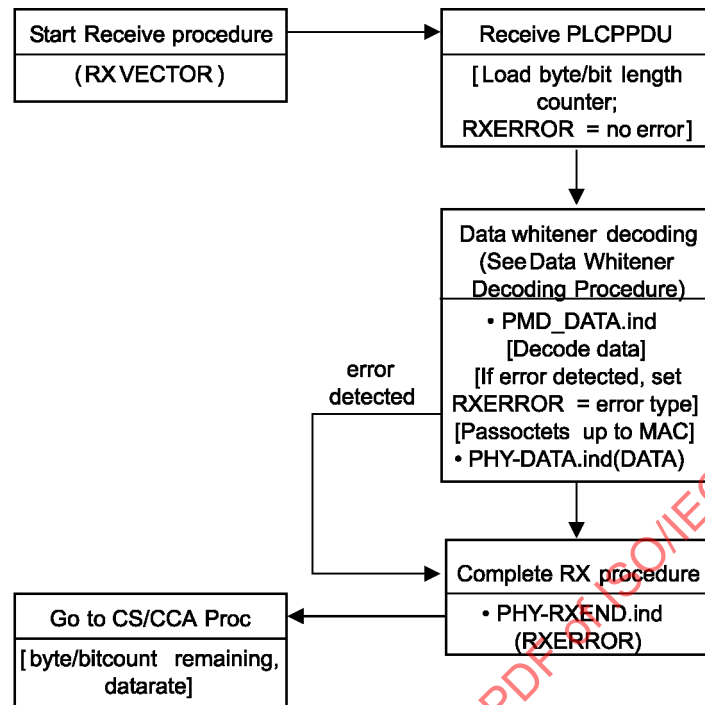
Figure 83—Receive state machine
