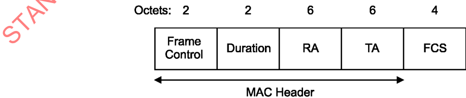
Figure 16—RTS frame
