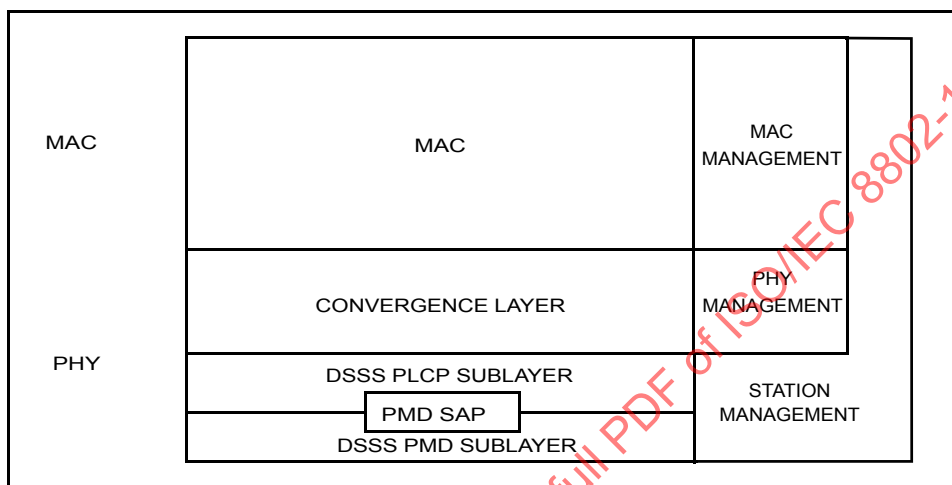
Figure 141—Layer reference model
