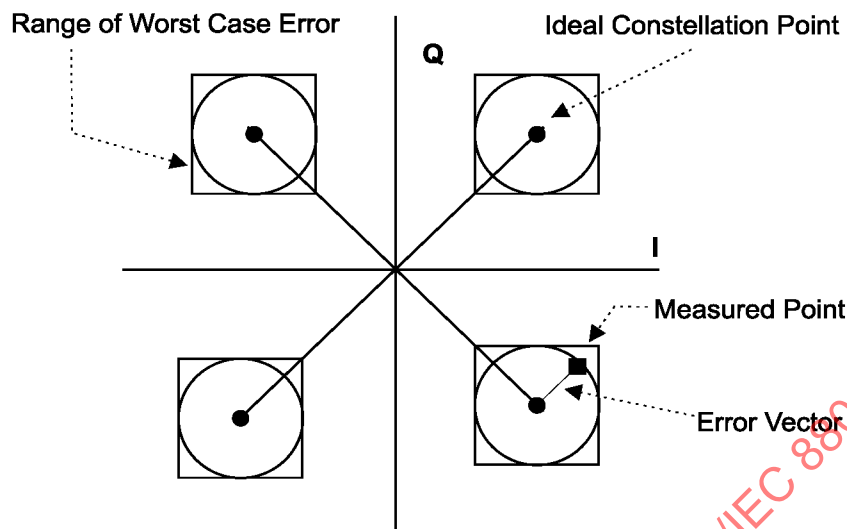
Figure 152—Modulation accuracy measurement example
