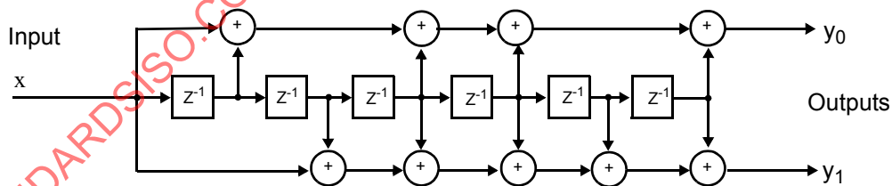
Figure 143—PBCC convolutional encoder
