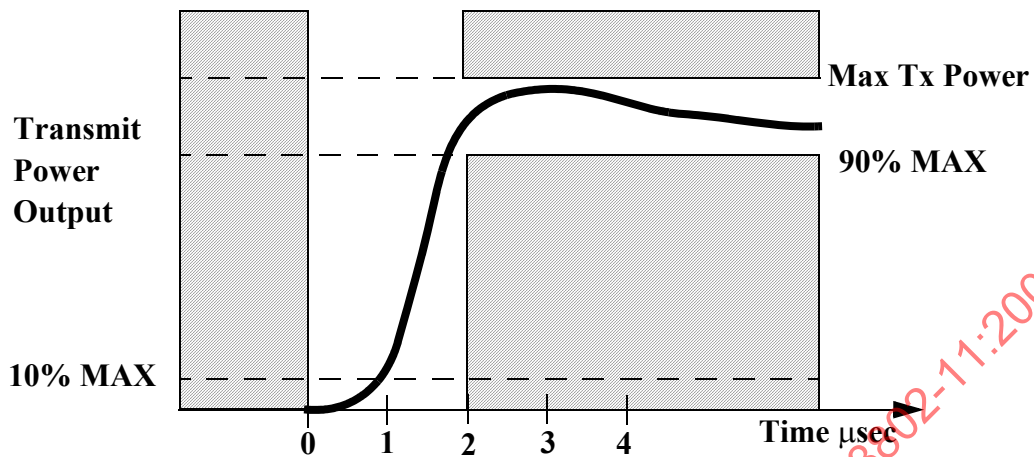
Figure 150—Transmit power-on ramp
