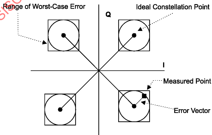
Figure 103—Modulation accuracy measurement example
