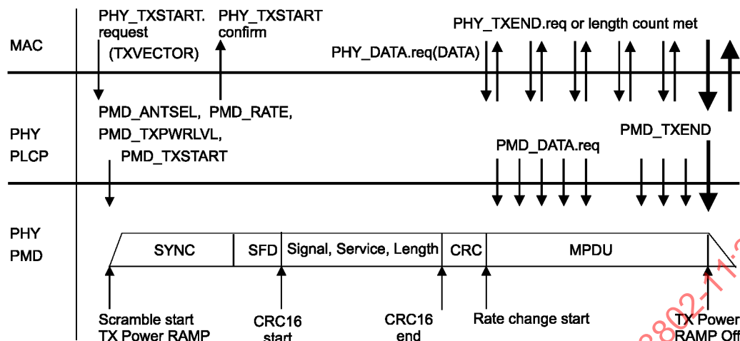
Figure 95—Transmit PLCP
