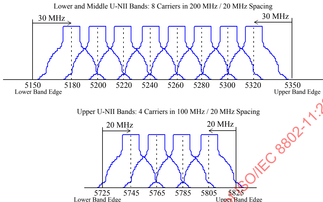
Figure 123—OFDM PHY frequency channel plan for the United States
