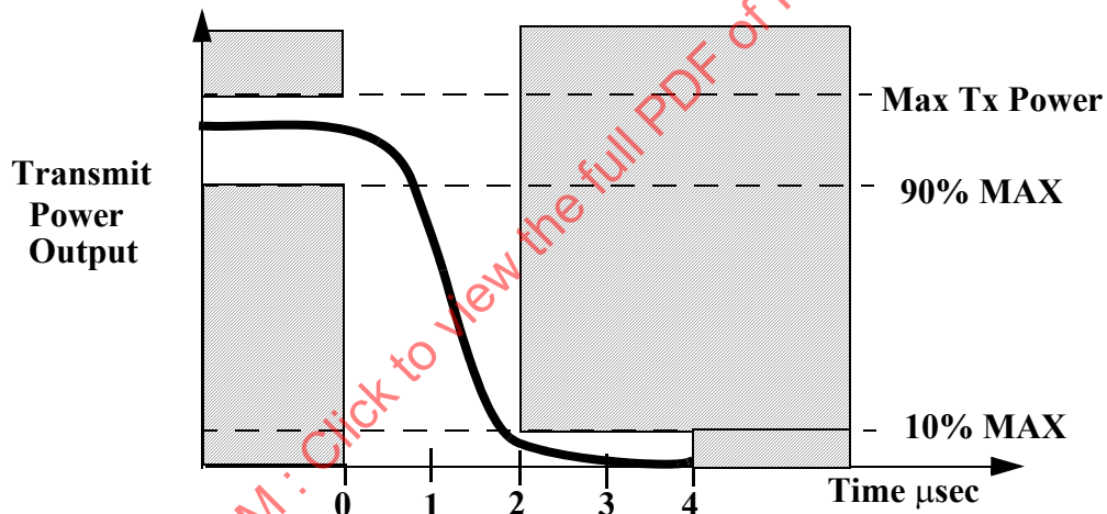
Figure 151—Transmit power-down ramp
