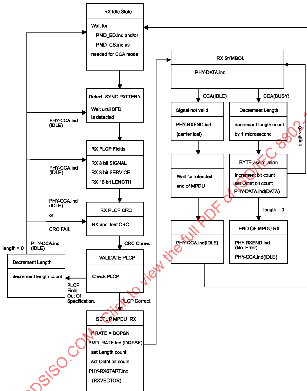
Figure 98—PLCP receive state machine
