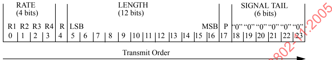
Figure 115—SIGNAL field bit assignment
