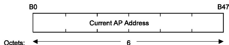
Figure 28—Current AP Address fixed field
