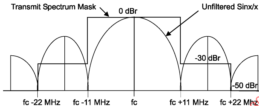
Figure 100—Transmit spectrum mask
