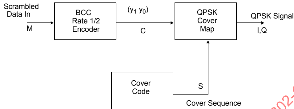
Figure 142—PBCC modulator scheme
