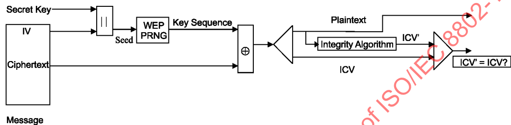
Figure 49—WEP decipherment block diagram
