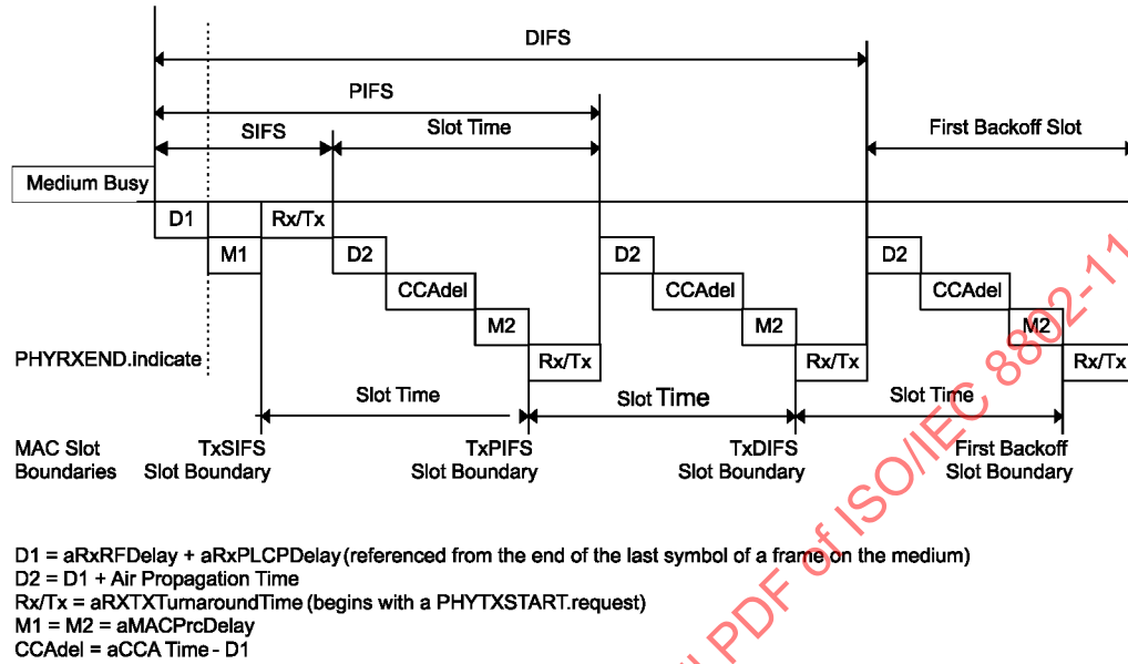
Figure 62—DCF timing relationships
