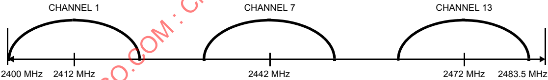
Figure 147—European channel selection—nonoverlapping
