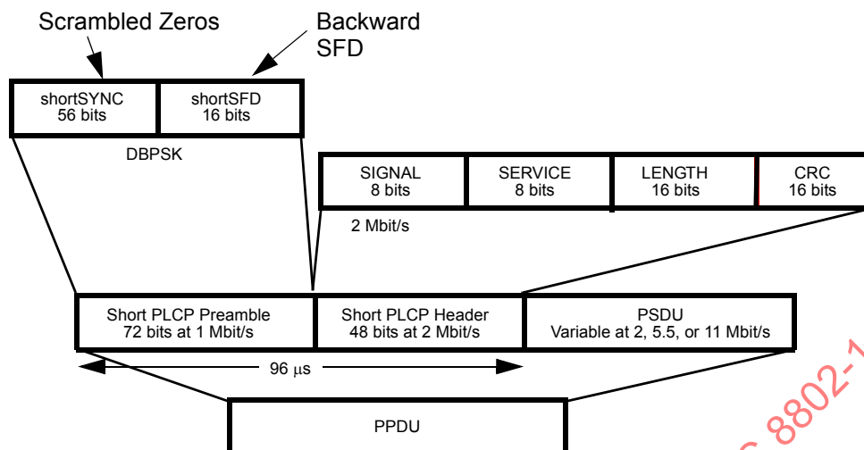
Figure 132—Short PPDU format
