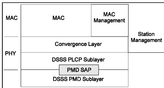
Figure 99—PMD layer reference model
