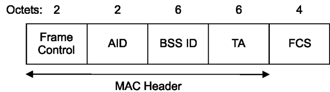
Figure 19—PS-Poll frame
