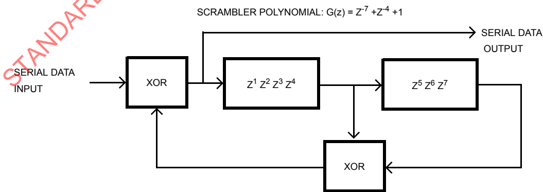
Figure 135—Data scrambler
