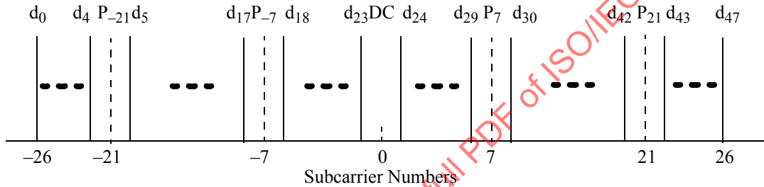
Figure 121—Subcarrier frequency allocation
