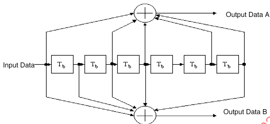
Figure 118—Convolutional encoder ( k = 7 )
