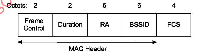
Figure 21—CF-End+CF-Ack Frame
