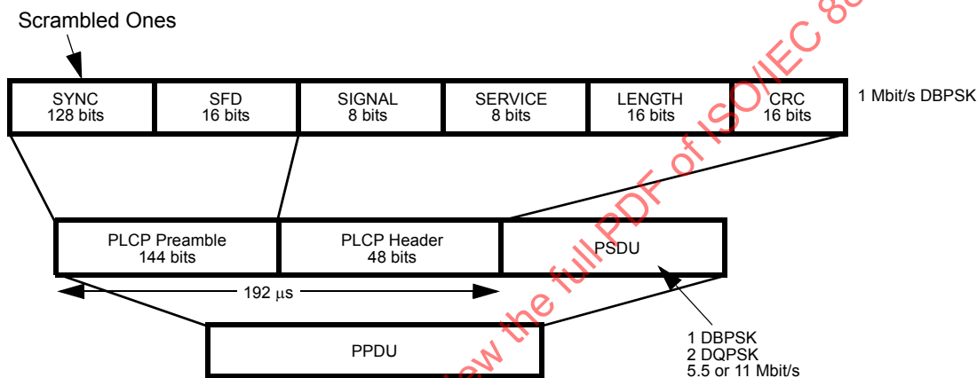
Figure 131—Long PPDU format
