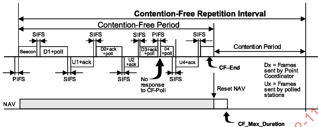
Figure 66—Example of PCF frame transfer
