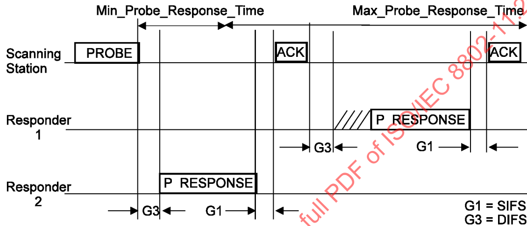
Figure 70—Probe response
