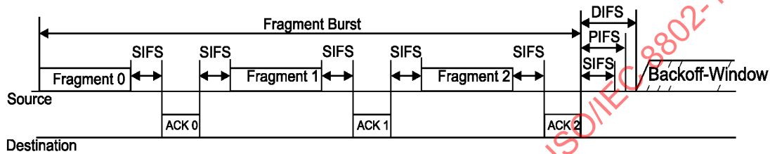
Figure 58—Transmission of a multiple-fragment MSDU using SIFS
