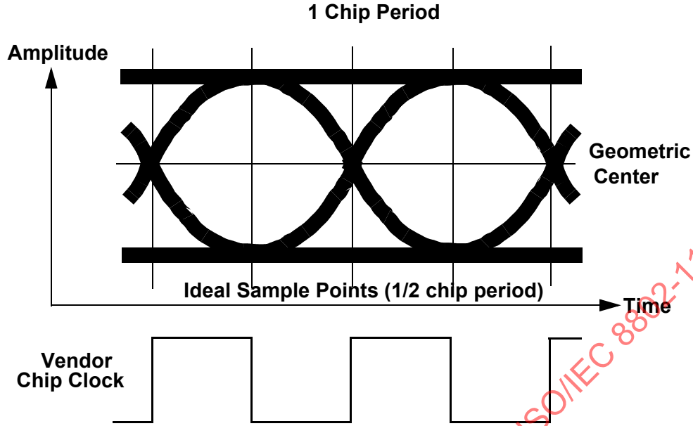
Figure 153—Chip clock alignment with baseband eye pattern
