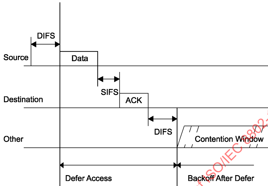
Figure 61—Directed data/ACK MPDU
