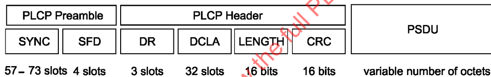
Figure 105—PPDU frame format
