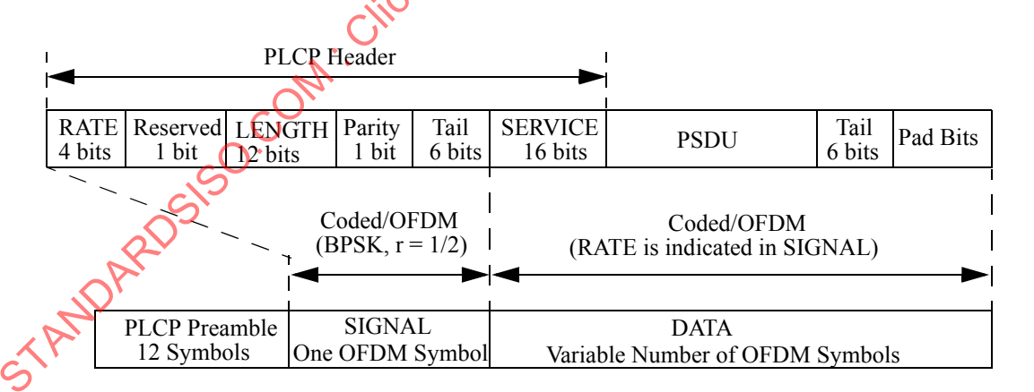
Figure 111—PPDU frame format
