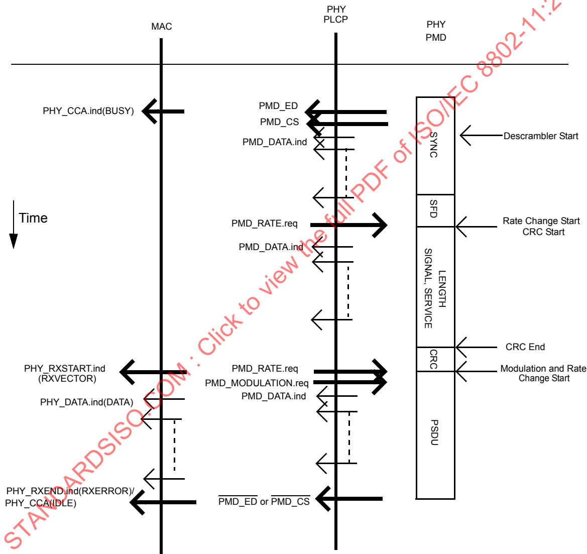
Figure 139—Receive PLCP
