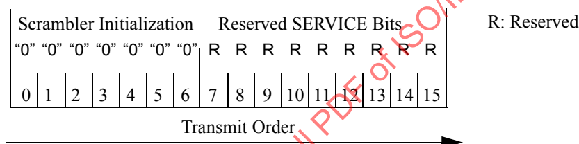
Figure 116—SERVICE field bit assignment
