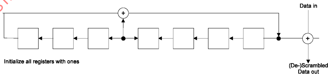
Figure 75—Frame synchronous scrambler/descrambler
