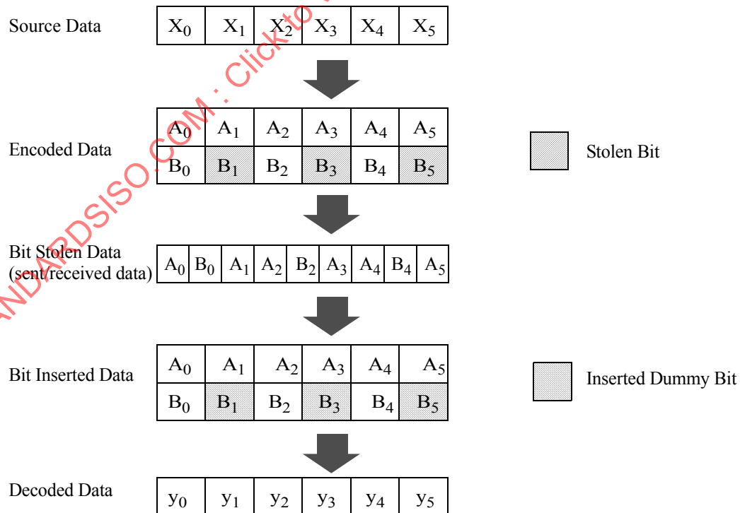
Figure 119—Example of the bit-stealing and bit-insertion procedure ( r = 3/4, 2/3 )
