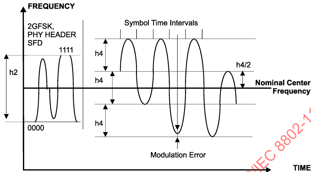
Figure 89—4GFSK transmit modulation
