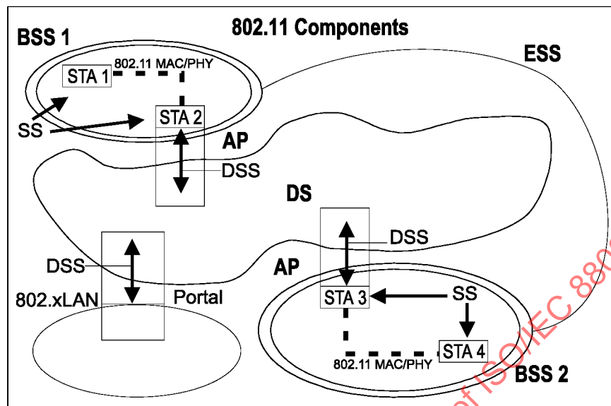
Figure 7—Complete IEEE 802.11 architecture
