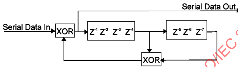
Figure 93—Data scrambler
