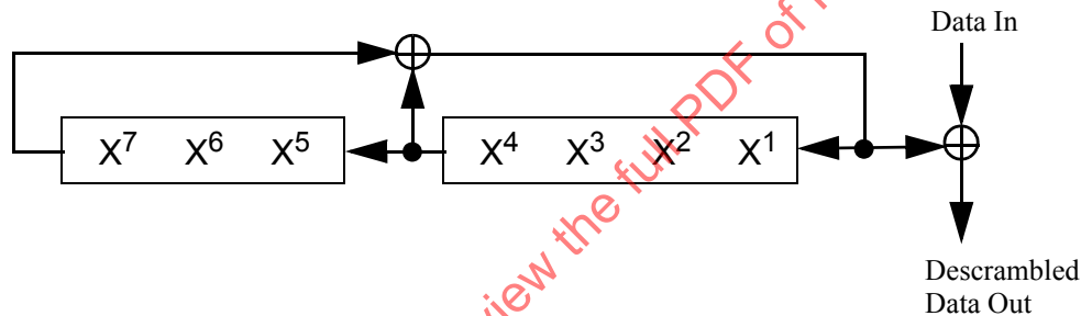
Figure 117—Data scrambler
