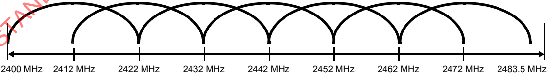
Figure 148—European channel selection—overlapping
