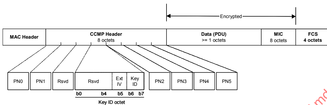
Figure 43n—Expanded CCMP MPDU
