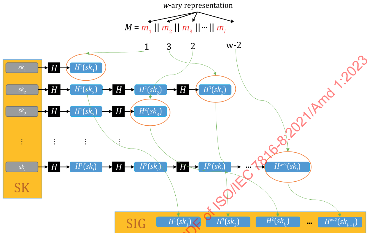
Figure F.3 — Winternitz-OTS signature principle
