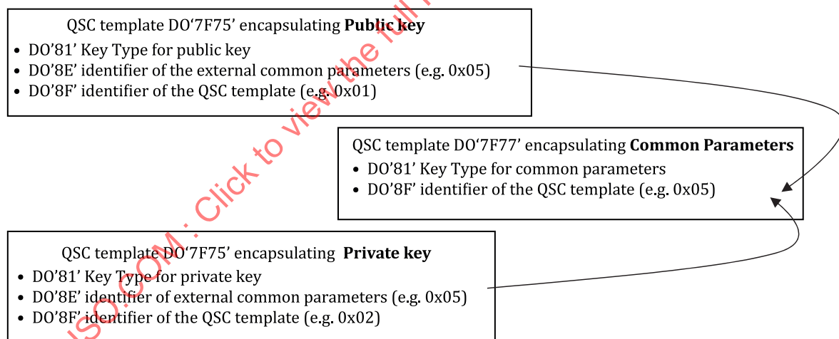
Figure AMD.1.1 — Identifier of external common parameters DO'8E' in QSC template
