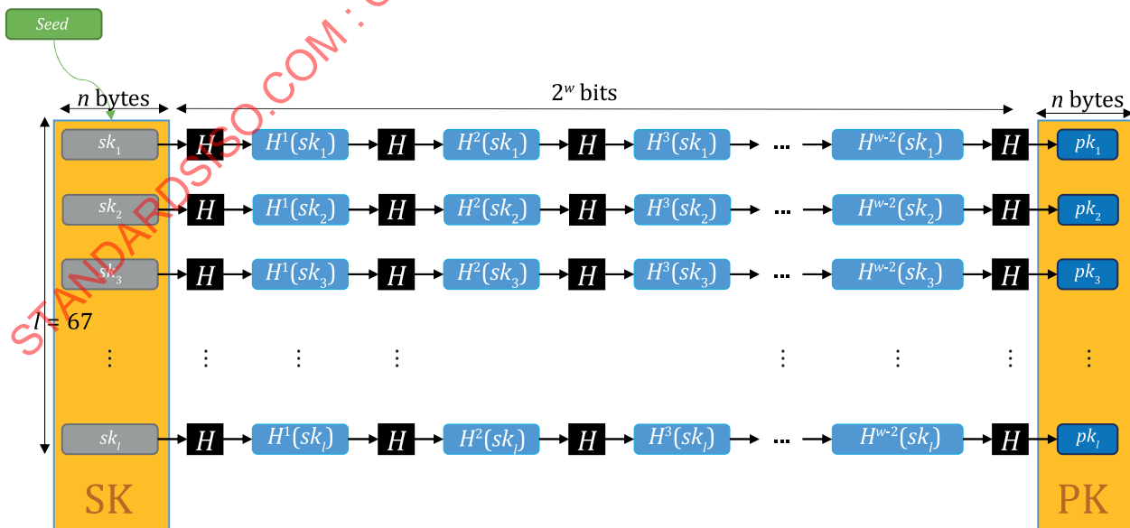
Figure F.2 — Winternitz-OTS, key generation
