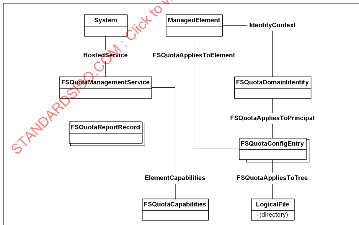
Figure 19 - Filesystem Quotas Instance Diagram
