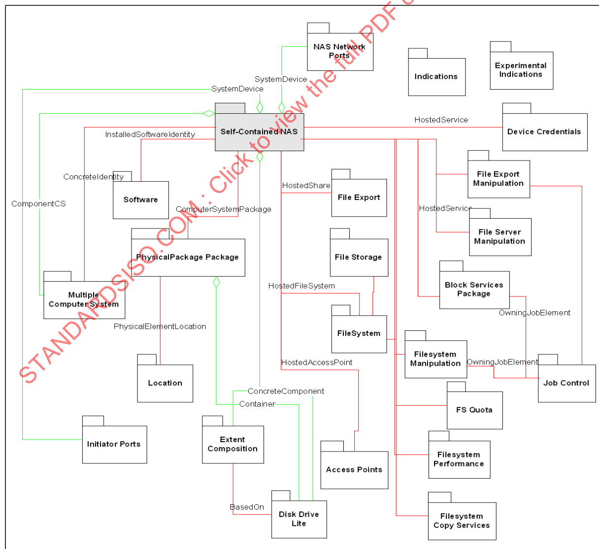
Figure 24 - Self-Contained NAS Profile and Subprofiles
