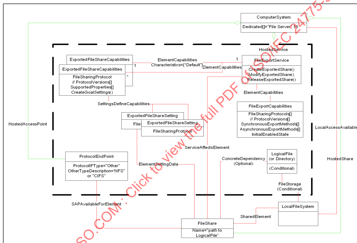
Figure 7 - Capabilities and Settings for Exported File Share Creation
