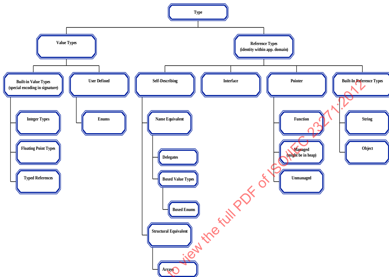
Figure 1: Type System
