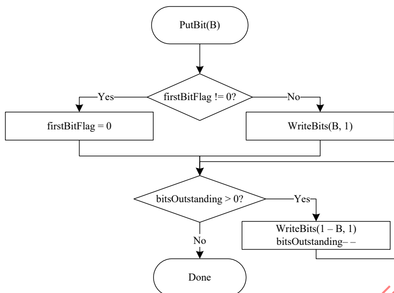
Figure 9-12 — Flowchart of PutBit(B)
