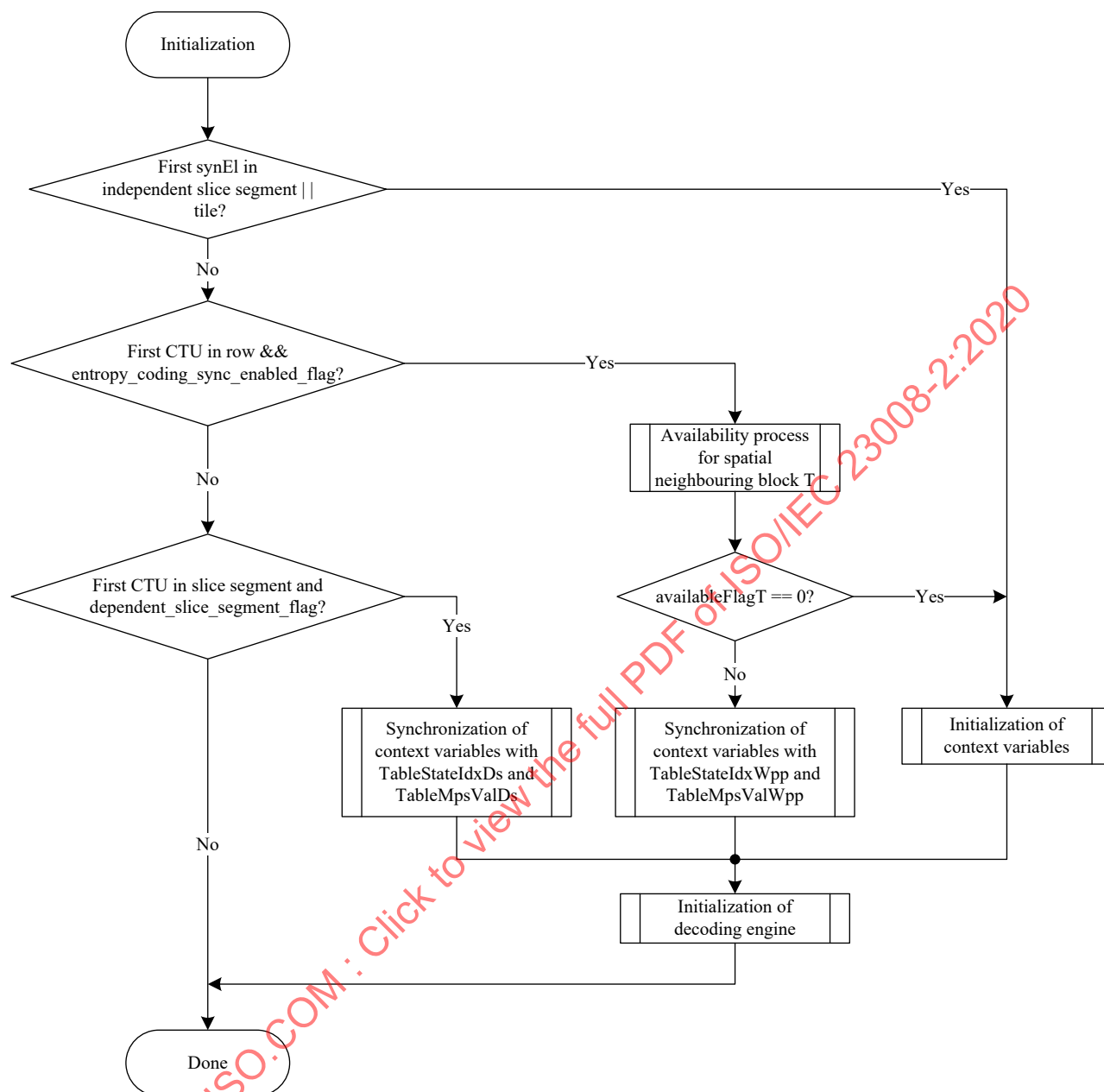
Figure 9-3 — Illustration of CABAC initialization process
