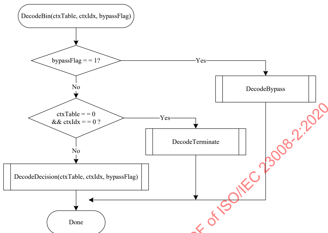
Figure 9-5 — Overview of the arithmetic decoding process for a single bin
