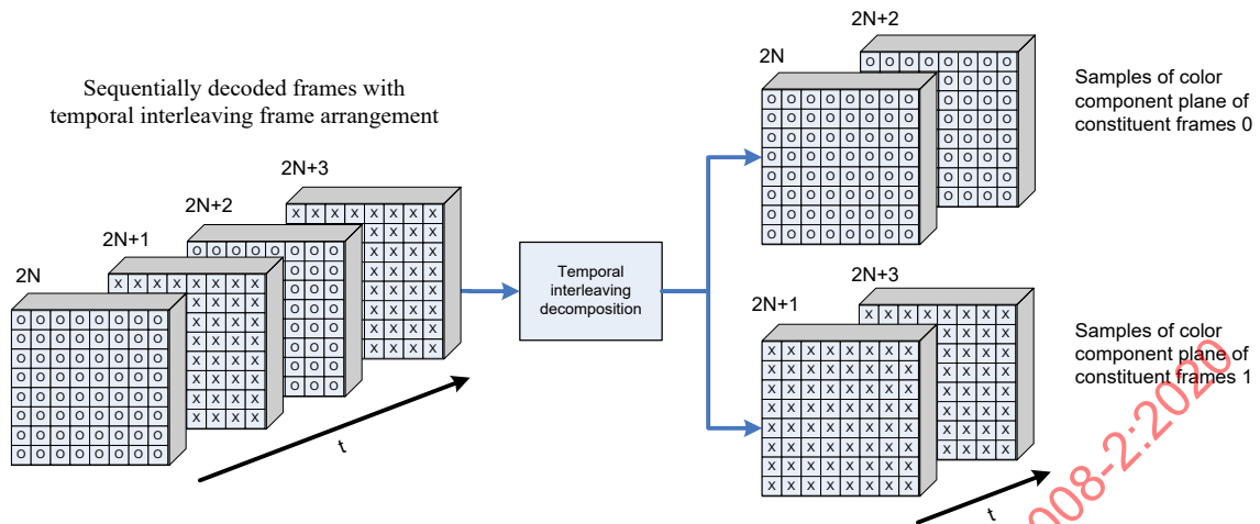
Figure D.9 — Rearrangement of a temporal interleaving frame arrangement (frame_packing_arrangement_type equal to 5)
