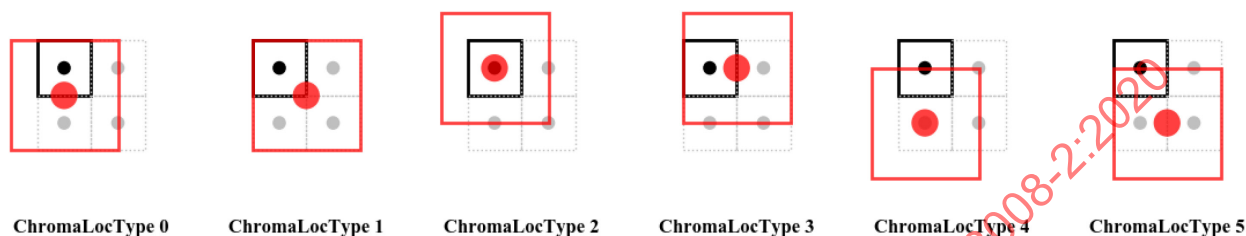
Figure E.2 – Location of the top-left chroma sample when chroma_format_idc is equal to 1 (4:2:0 chroma format) as a function of ChromaLocType
