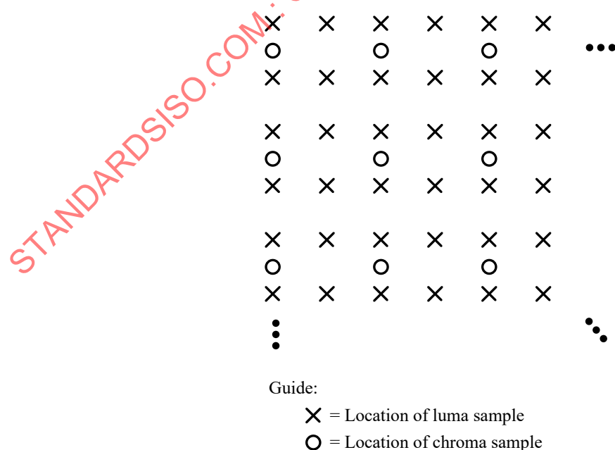
Figure 6-1 — Nominal vertical and horizontal locations of 4:2:0 luma and chroma samples in a picture
