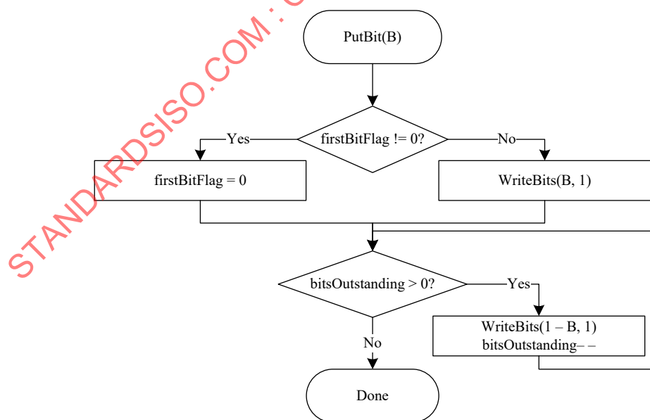
Figure 9-12 — Flowchart of PutBit(B)
