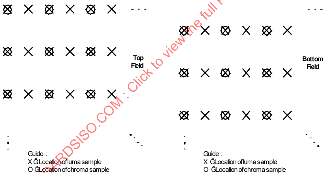
Figure D.2 — Nominal vertical and horizontal sampling locations of 4:2:2 samples in top and bottom fields
