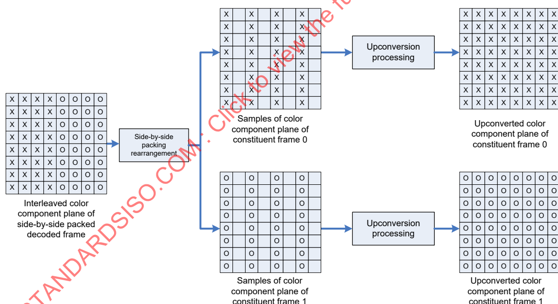
Figure D.4 — Rearrangement and upconversion of side-by-side packing arrangement with frame_packing_arrangement_type equal to 3, quincunx_sampling_flag equal to 0, and ( x, y ) equal to ( 0, 0 ) or ( 4, 8 ) for both constituent frames
