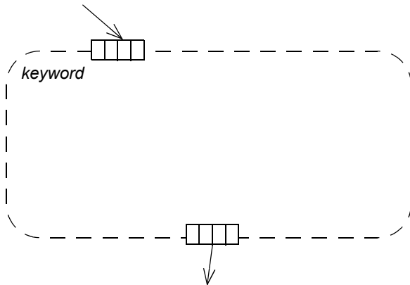
Figure 12.82 - Expansion region
