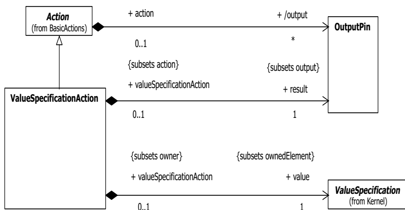
Figure 11.11 - Miscellaneous actions
