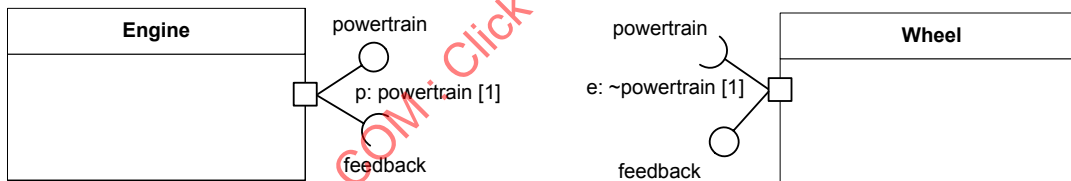
Figure 9.16 - Port notation
