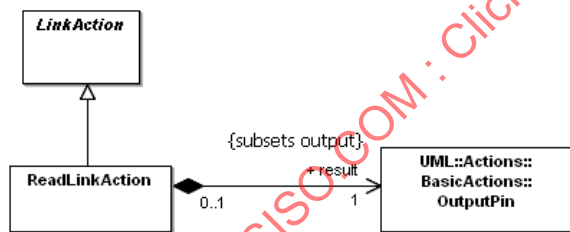
Figure 11.9 - Read link actions
