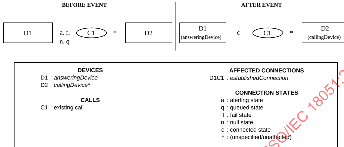
Figure 17-42 Established Event
