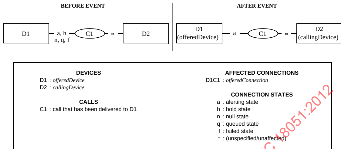
Figure 17-47 Offered Event
