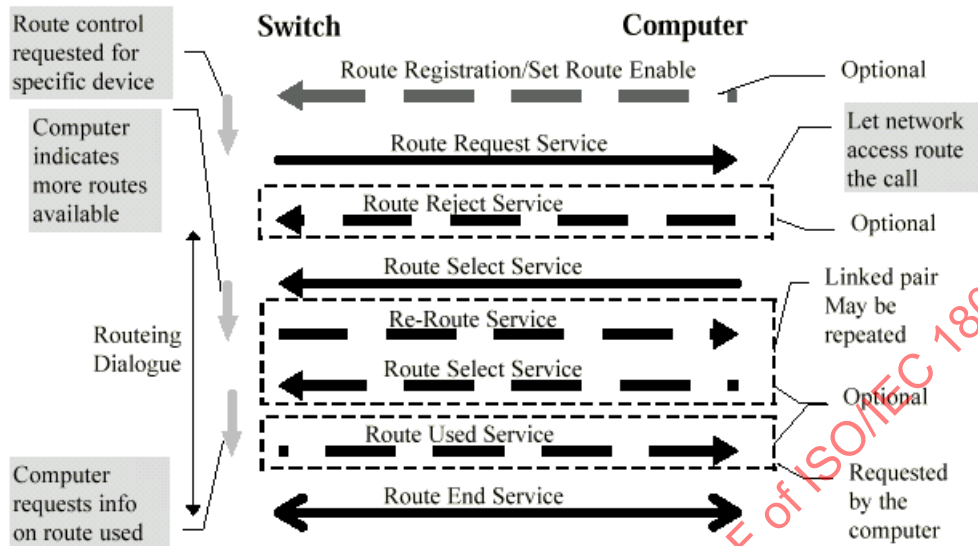
Figure 6-32 Overview of a Routing Dialogue
