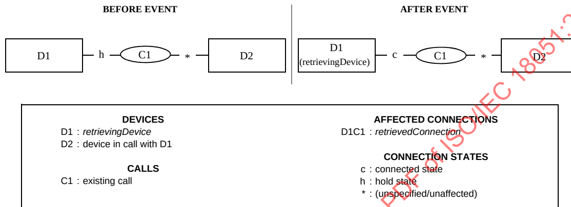
Figure 17-50 Retrieved Event
