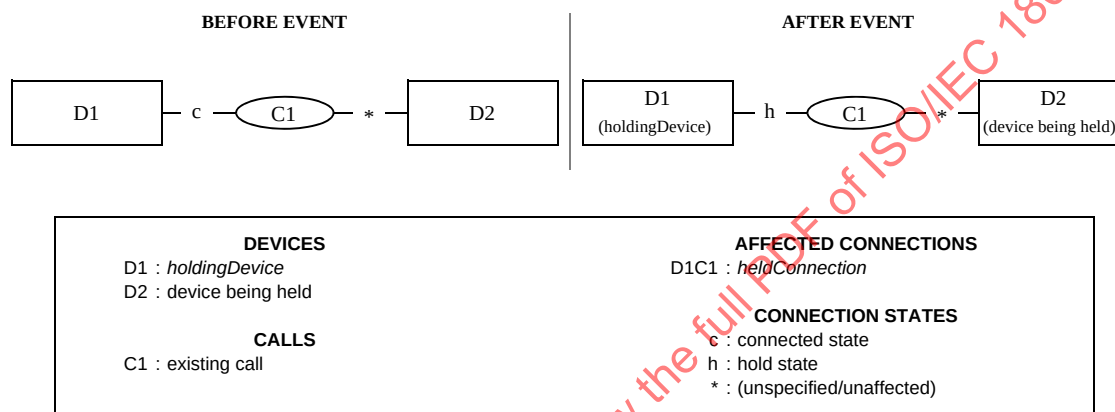
Figure 17-44 Held Event
