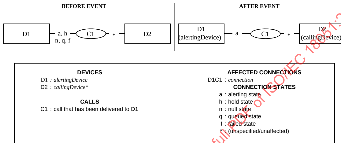
Figure 17-39 Delivered Event
