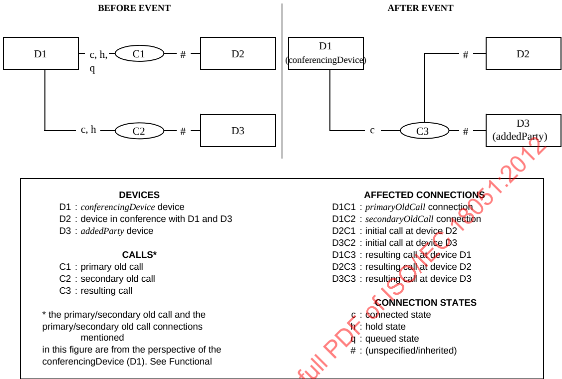
Figure 17-35 Conferenced Event—Case B: Single Step Conferencing
