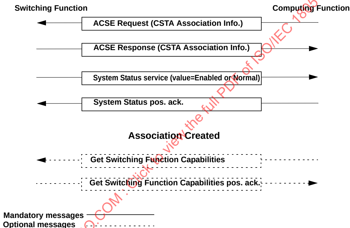
Figure 7-3 Explicit Association Created using ACSE - Initialization Sequence
