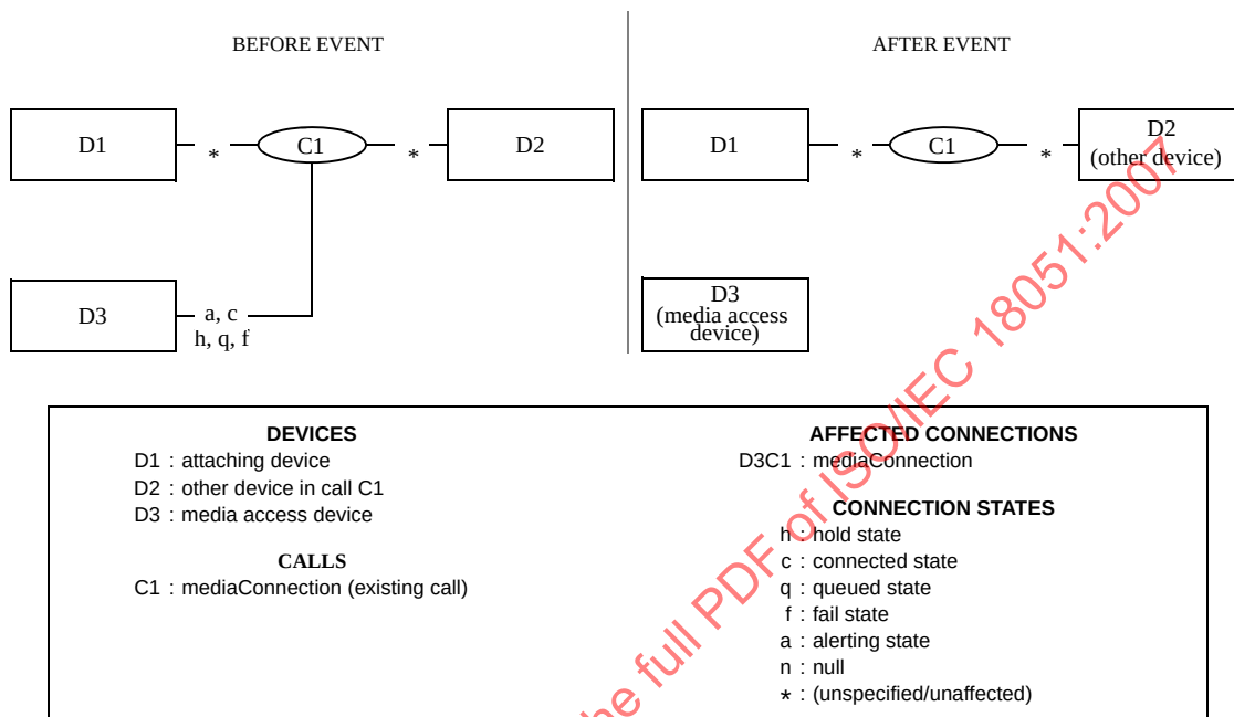
Figure 19-3 Media Detached Event (Case A)
