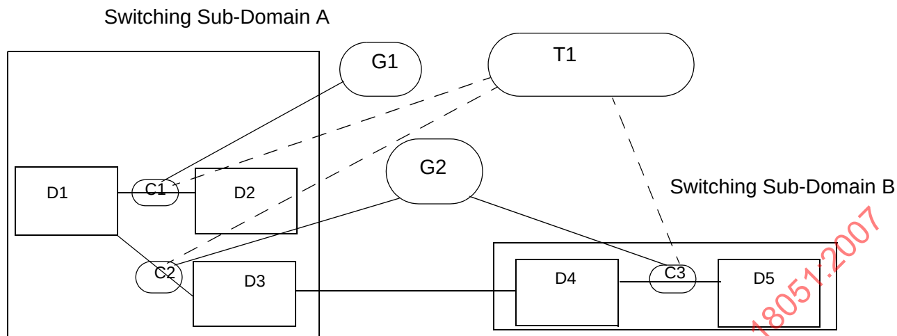
Figure 6-22 Illustration of a Call Thread
