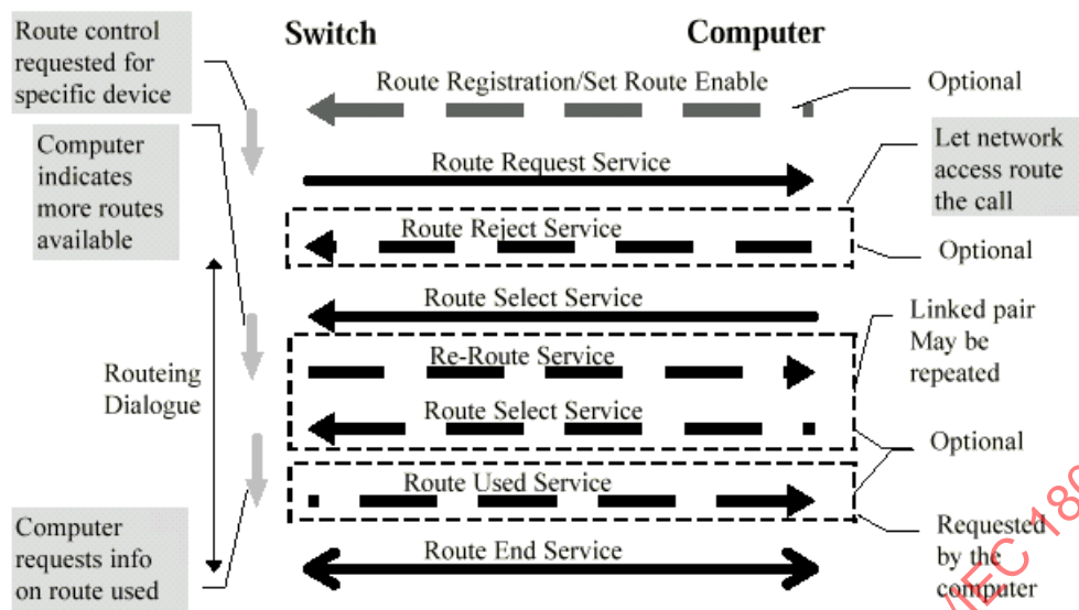
Figure 6-31 Overview of a Routing Dialogue
