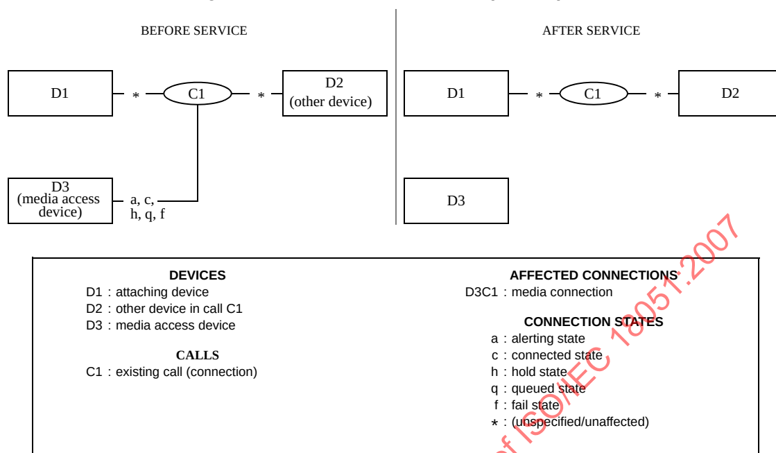
Figure 19-1 Detach Media Service (Case A)
