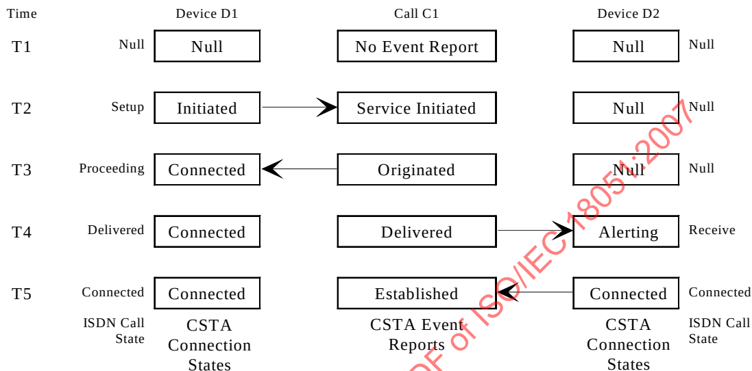
Figure 6-25 Relationship of CSTA Call Event Reports
