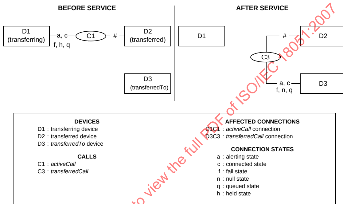
Figure 17-28 Single Step Transfer Call Service
