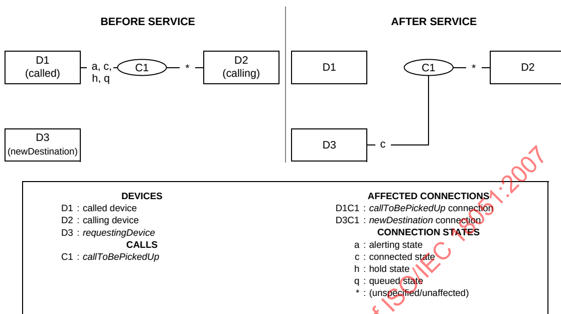
Figure 17-14 Directed Pickup Call Service
