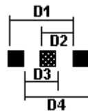
Figure 14 — Edge-to-edge measurements for finding an element centre
