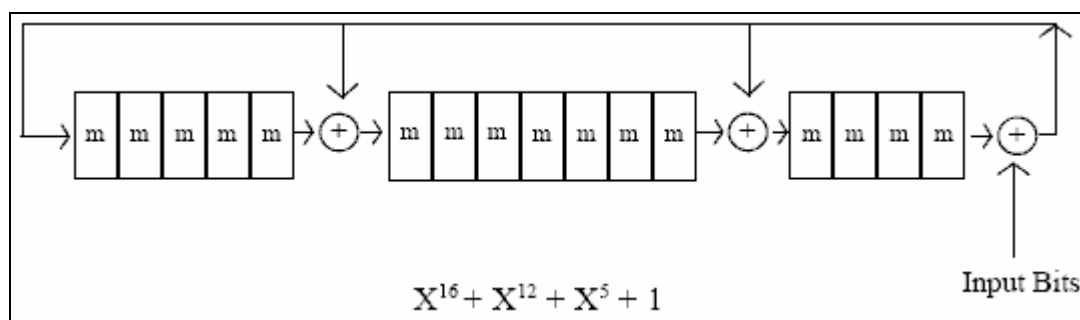
Figure J.1 — CRC algorithm schematic
