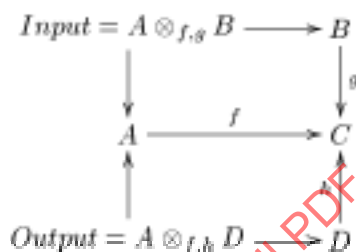
Figure 13 — Illustration of double pullback in which an input graph is mapped to a rule graph
