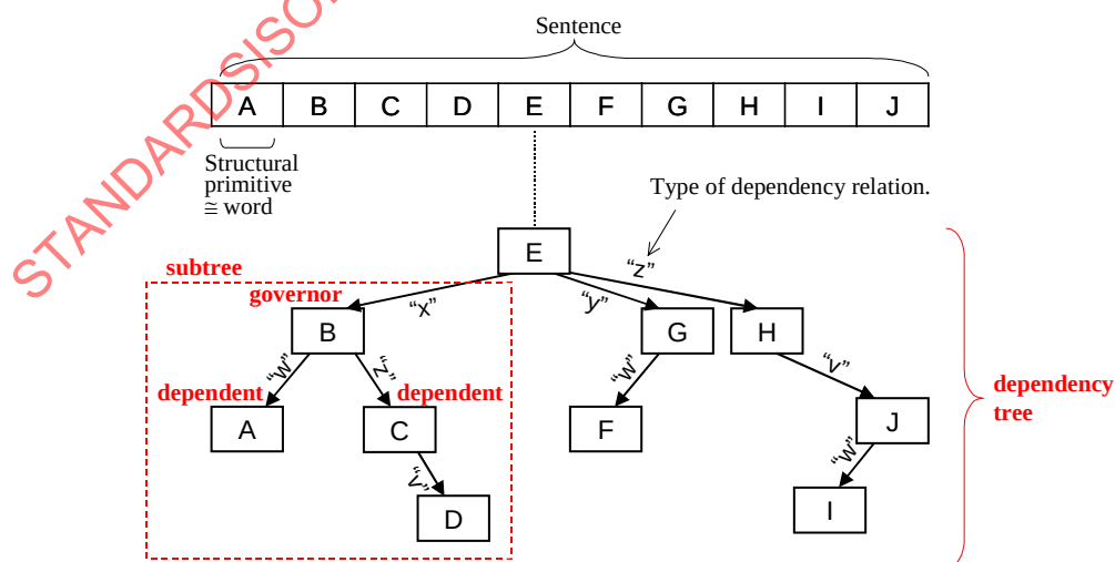
Figure 5 — Illustration of the dependency structure among the governors and dependents of a sentence
