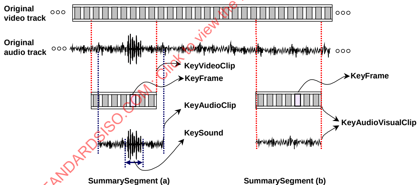
Figure 61 — Illustration of SummarySegment elements containing a KeyAudioVisualClip, KeyVideoClip, KeyAudioClip, KeyFrame and KeySound
