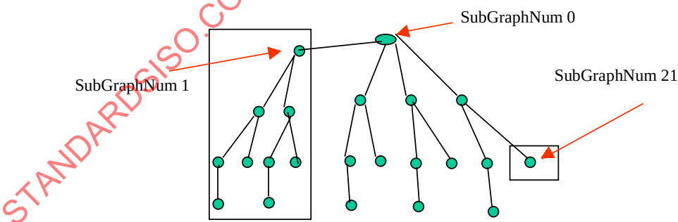
Figure 33 — Example of a scene graph mask
