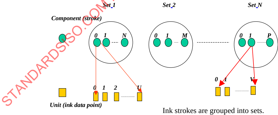
Figure 34 — Example of an ordered group mask
