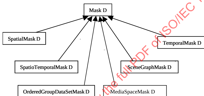
Figure 31 — Organization of segment mask description tools
