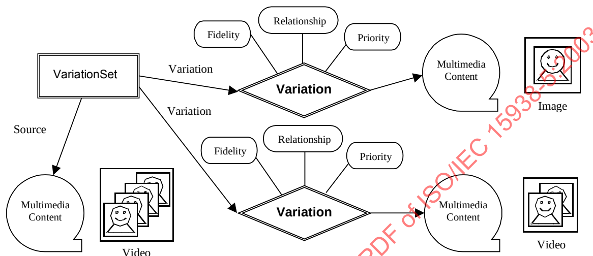
Figure 72 — Illustration of key concepts of Variation DS including VariationSet, Variation, variationFidelity, variationPriority and VariationRelationship
