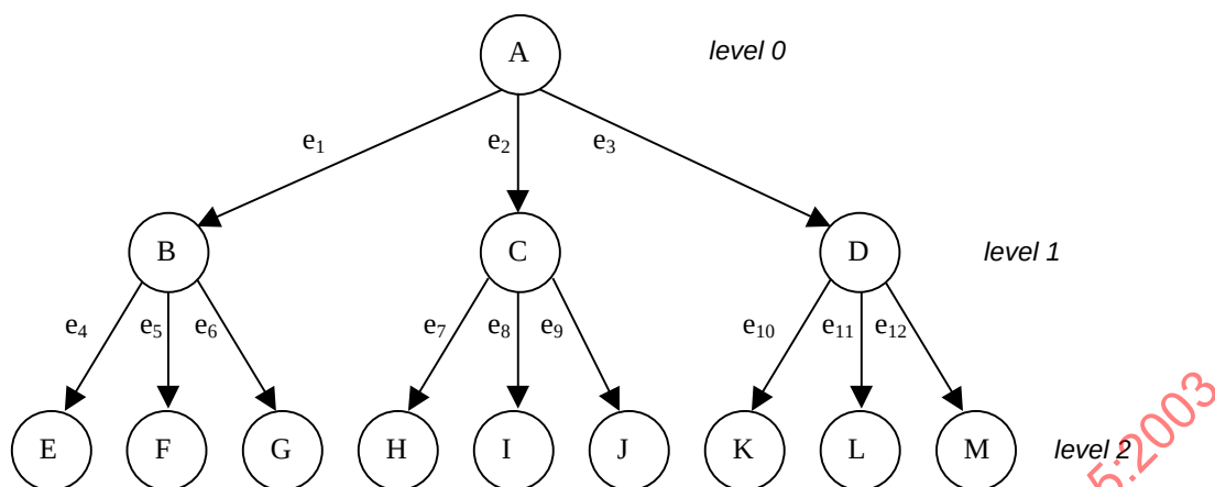
Figure 62 — An example of a key-frame hierarchy
