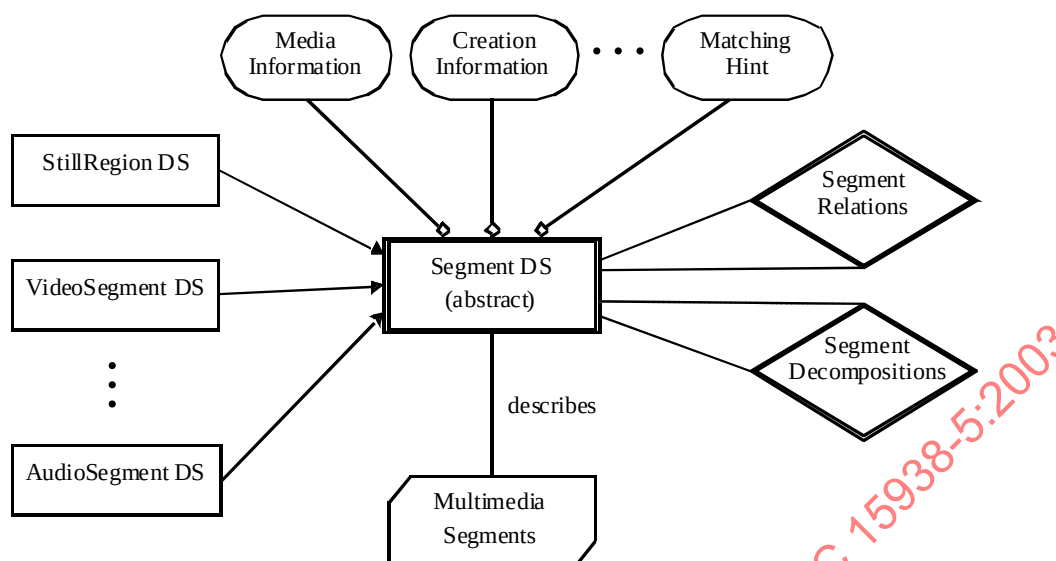
Figure 22 — Illustration of the organization of the tools for describing the structure of multimedia content
