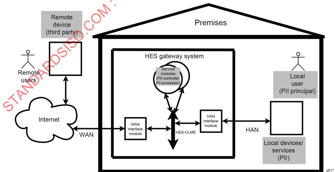
Figure A.1 – System layout for ISO/IEC 29100
