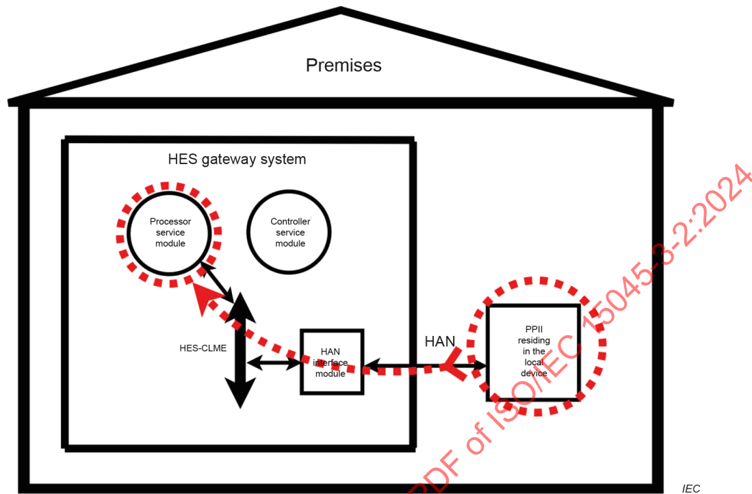
Figure B.5 – Local device or user to processor service module
