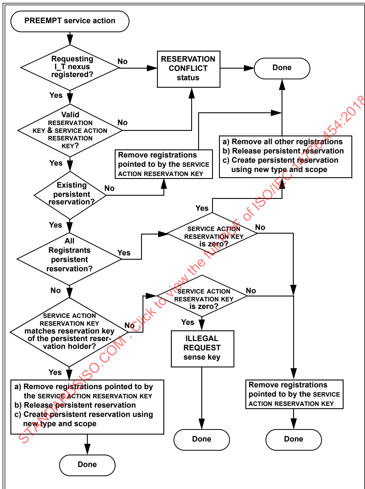
Figure 9 — Device server interpretation of PREEMPT service action
