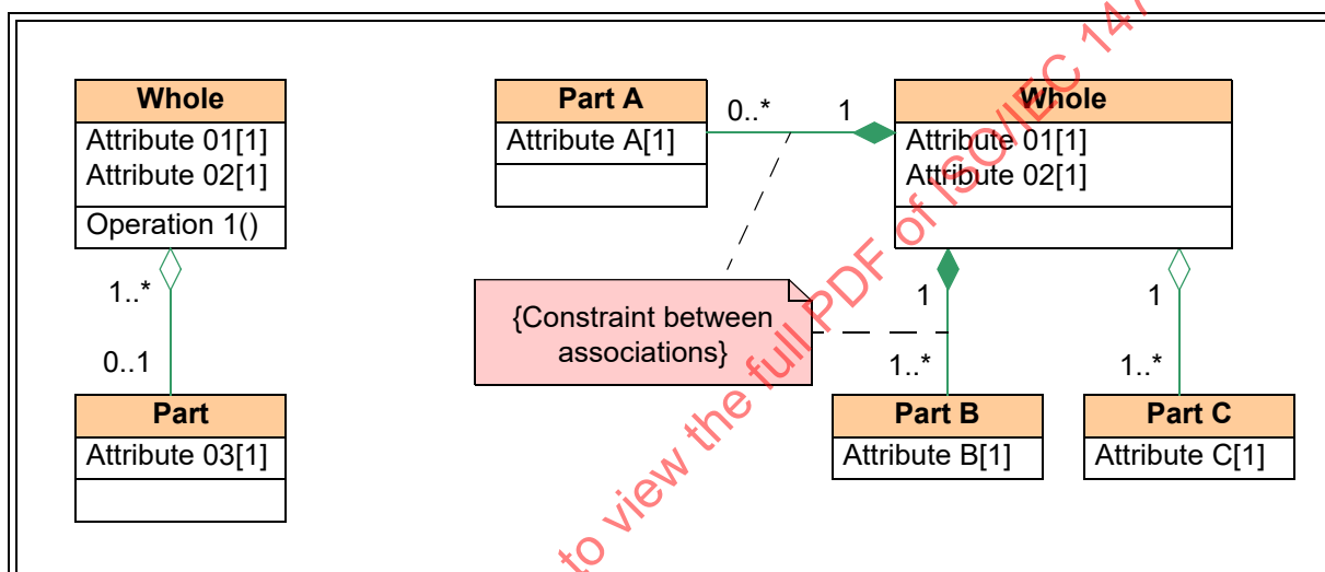
Figure 5 — Example class aggregation relationships
