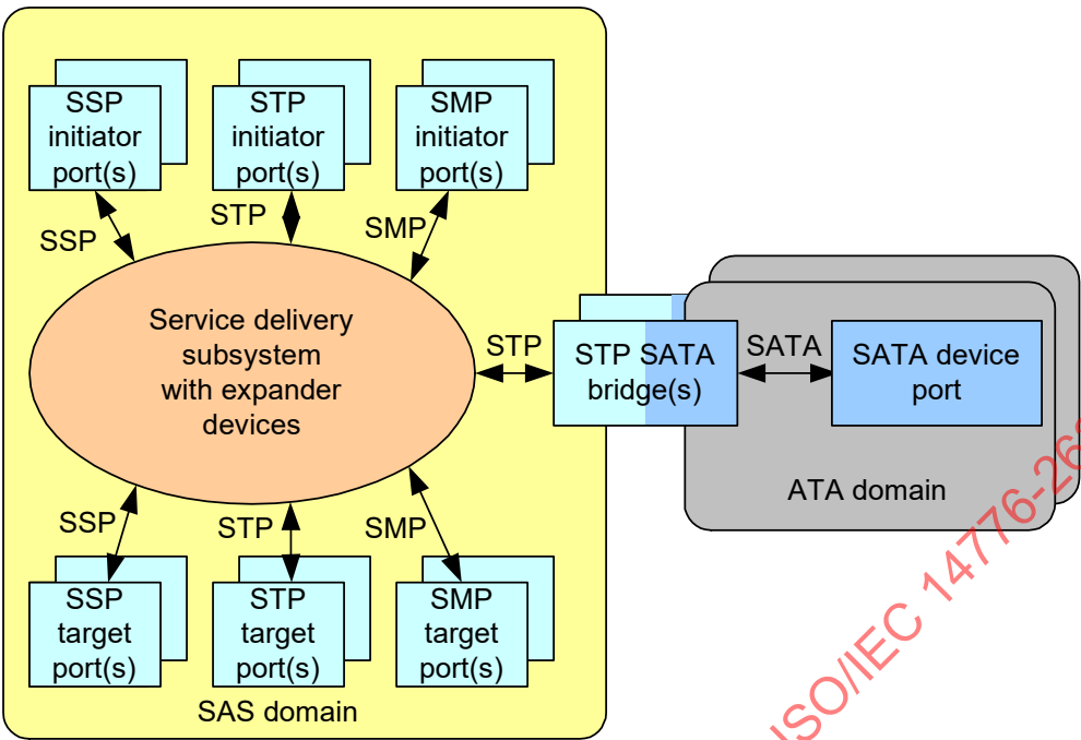
Figure 20 — SAS domain bridging to ATA domains
