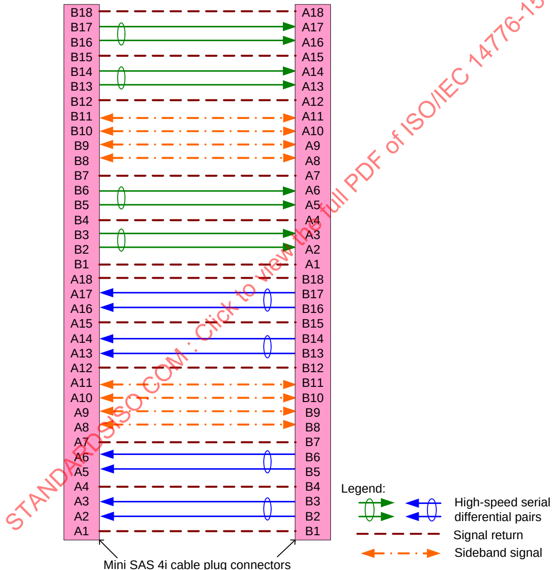
Figure 79 — SAS internal symmetric cable assembly - Mini SAS 4i
