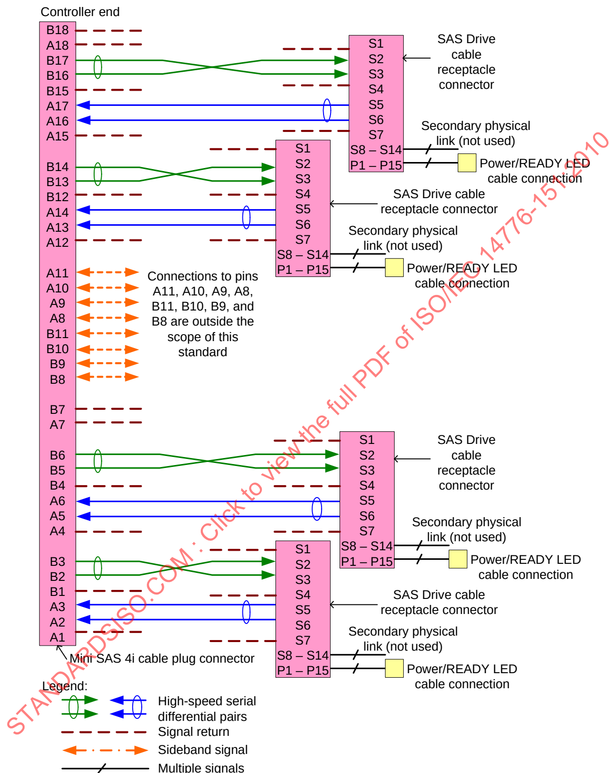
Figure 82 — SAS internal controller-based fanout cable assembly - Mini SAS 4i
