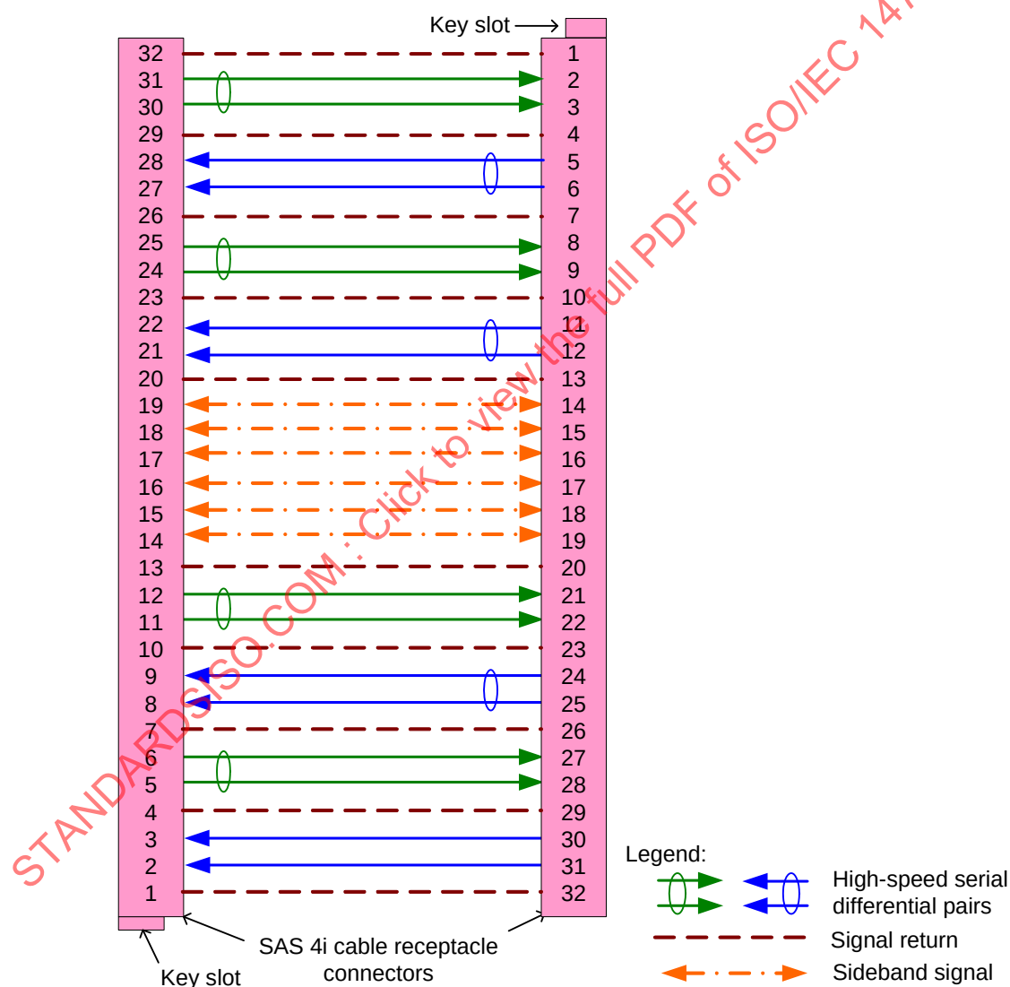
Figure 78 — SAS internal symmetric cable assembly - SAS 4i
