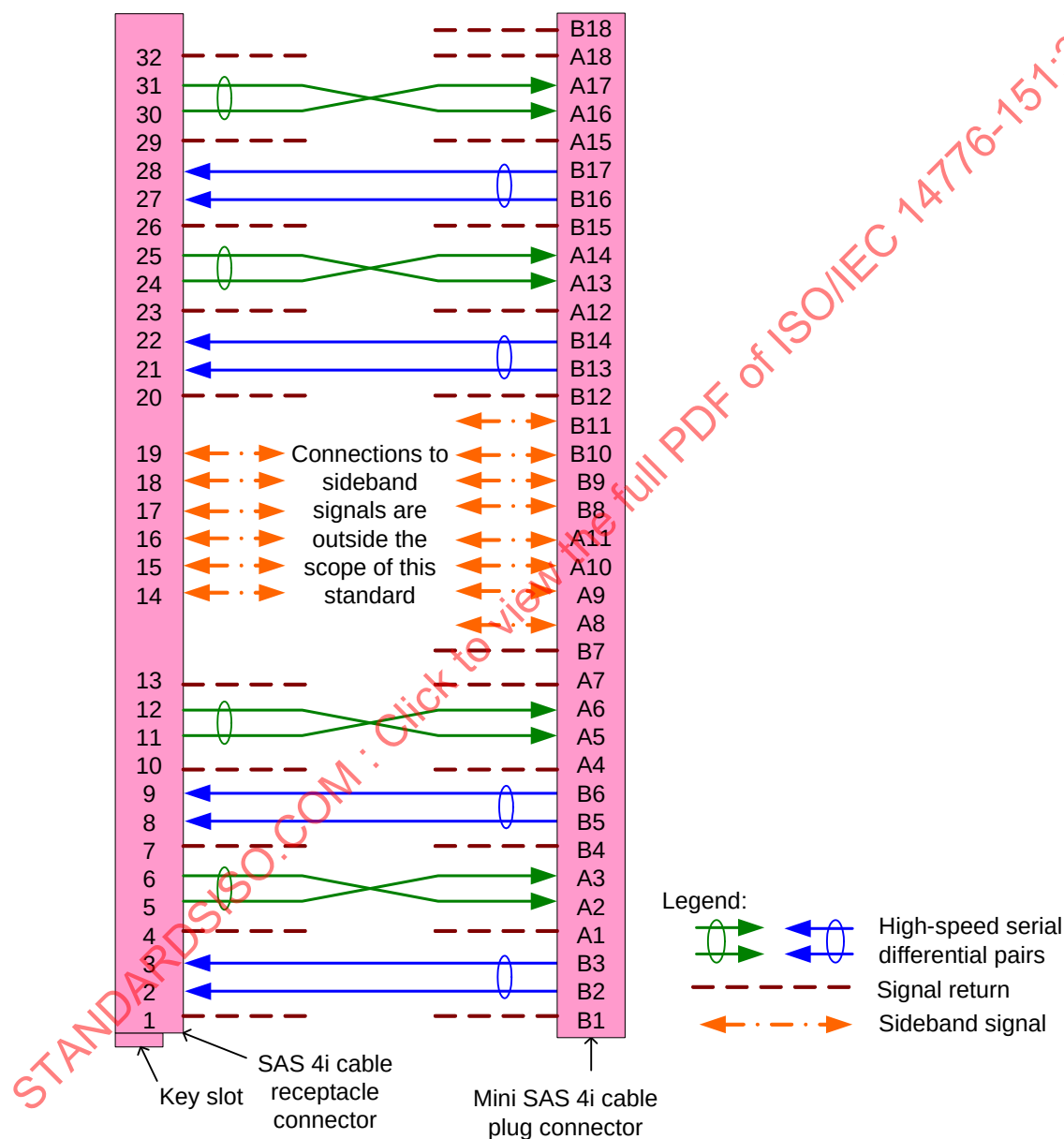
Figure 80 — SAS internal symmetric cable assembly - SAS 4i to Mini SAS 4i
