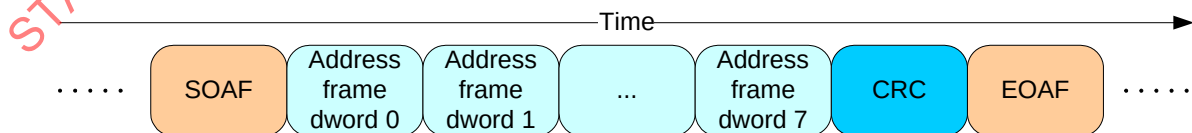
Figure 139 — Address frame transmission
