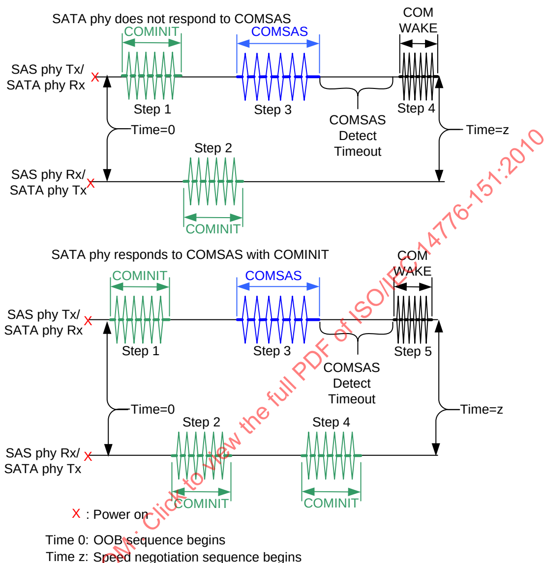
Figure 116 — SAS to SATA OOB sequence
