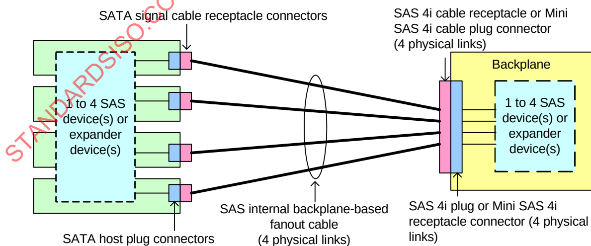
Figure 58 — SAS internal backplane-based fanout cable environment
