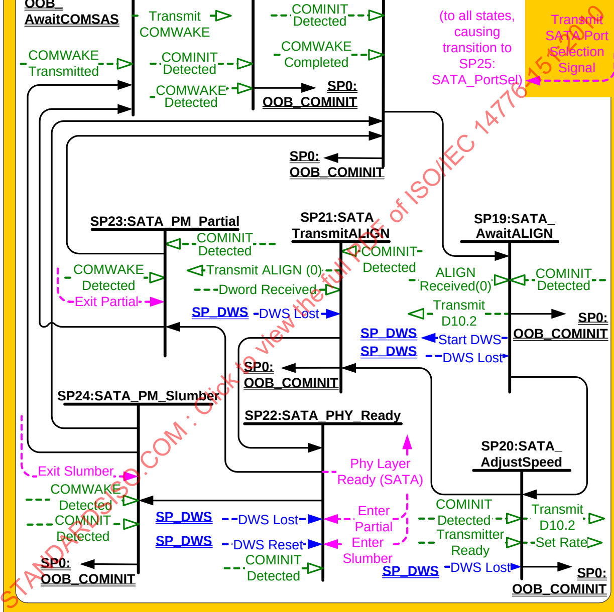
Figure 124 — SP (phy layer) state machine - SATA host emulation states
