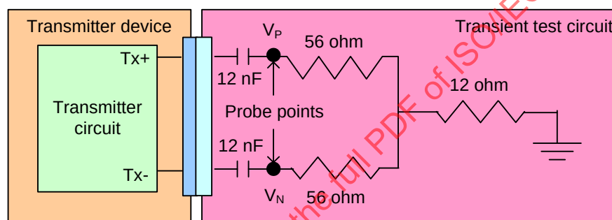
Figure 103 — Transmitter device transient test circuit
