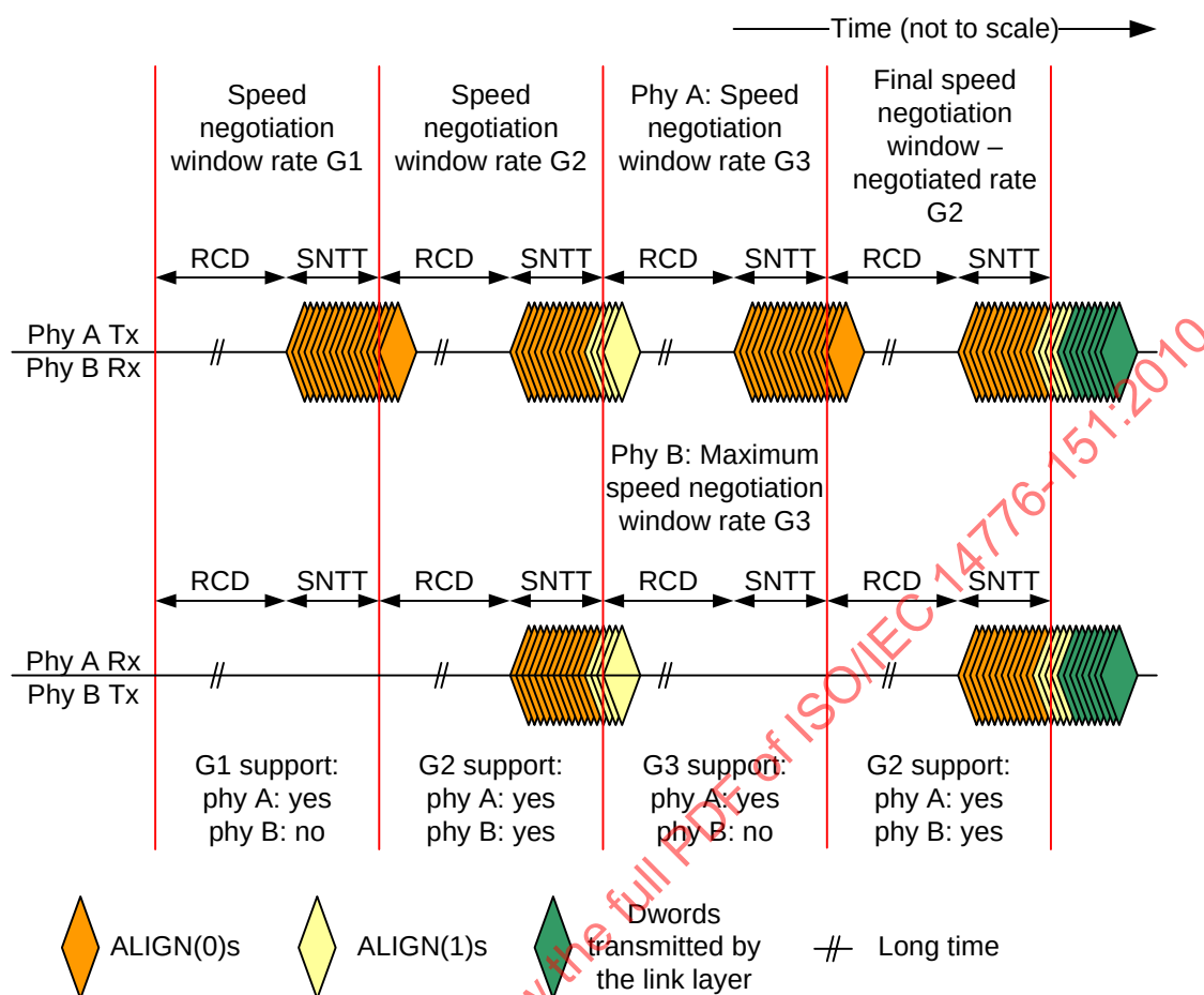
Figure 119 — SAS speed negotiation sequence (phy A: G1, G2, G3, phy B: G2 only)
