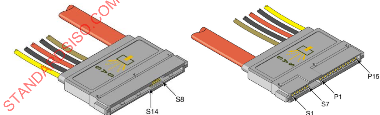
Figure 60 — Single-port SAS Drive cable receptacle connector
