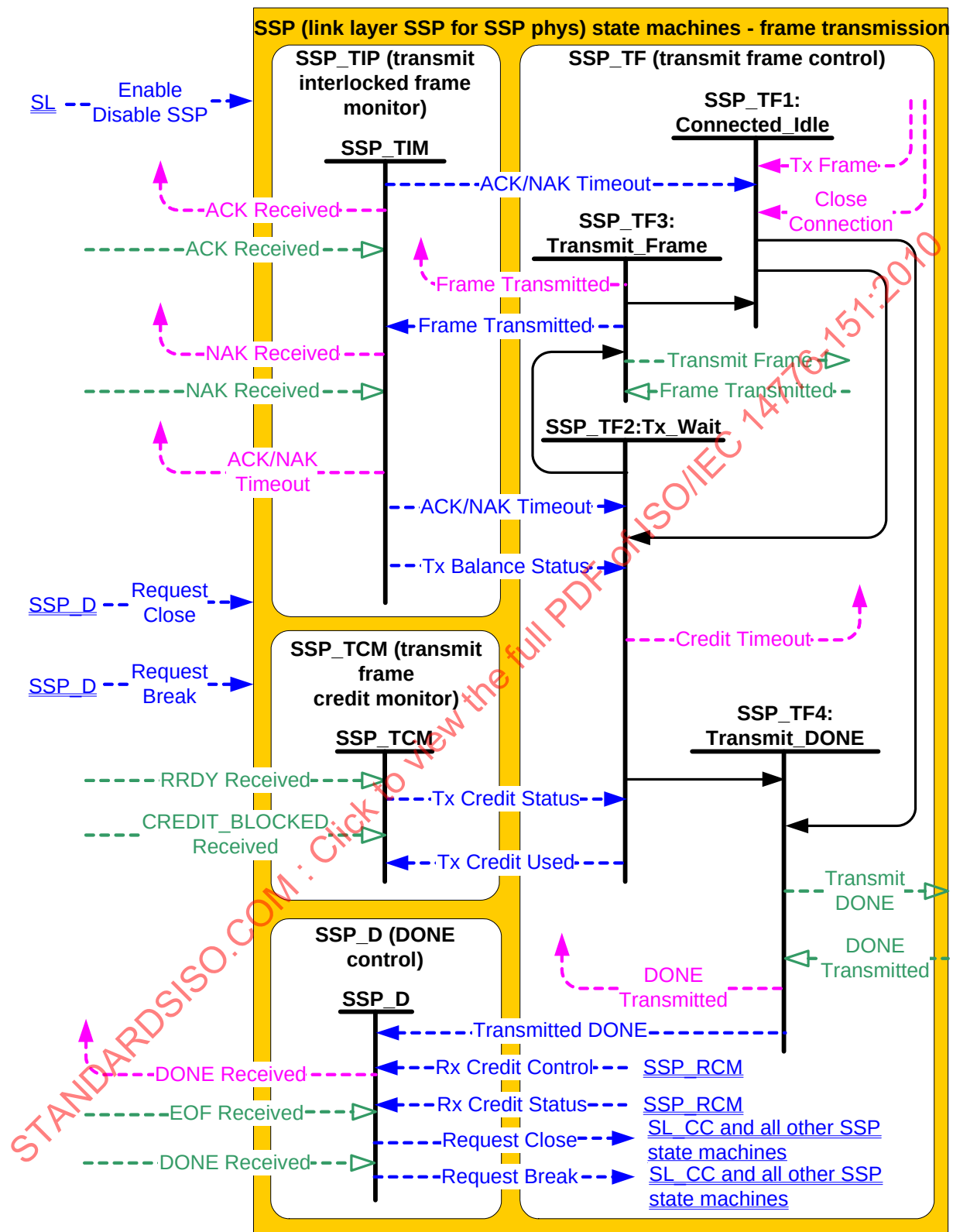
Figure 155 — SSP (link layer for SSP phys) state machines (part 1 - frame transmission)
