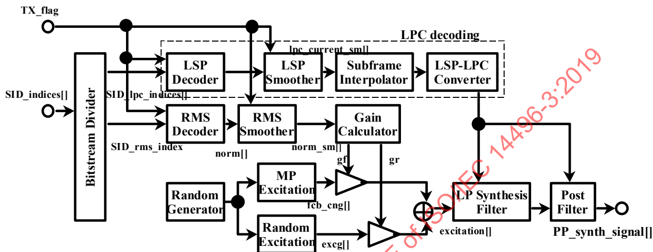
Figure 3.11 — CNG module
